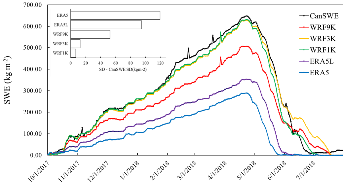
Figure 2. Temporal variation of SWE, from CanSWE data, WRF model resolutions, ERA5L and ERA5 over the SSRB region. The SWE data are aggregated for all stations inside the innermost domain. The spikes in the graph correspond to snowfall events, indicating the accumulation and subsequent melting of snow. The difference between CanSWE SD and each dataset is shown in the upper left.
