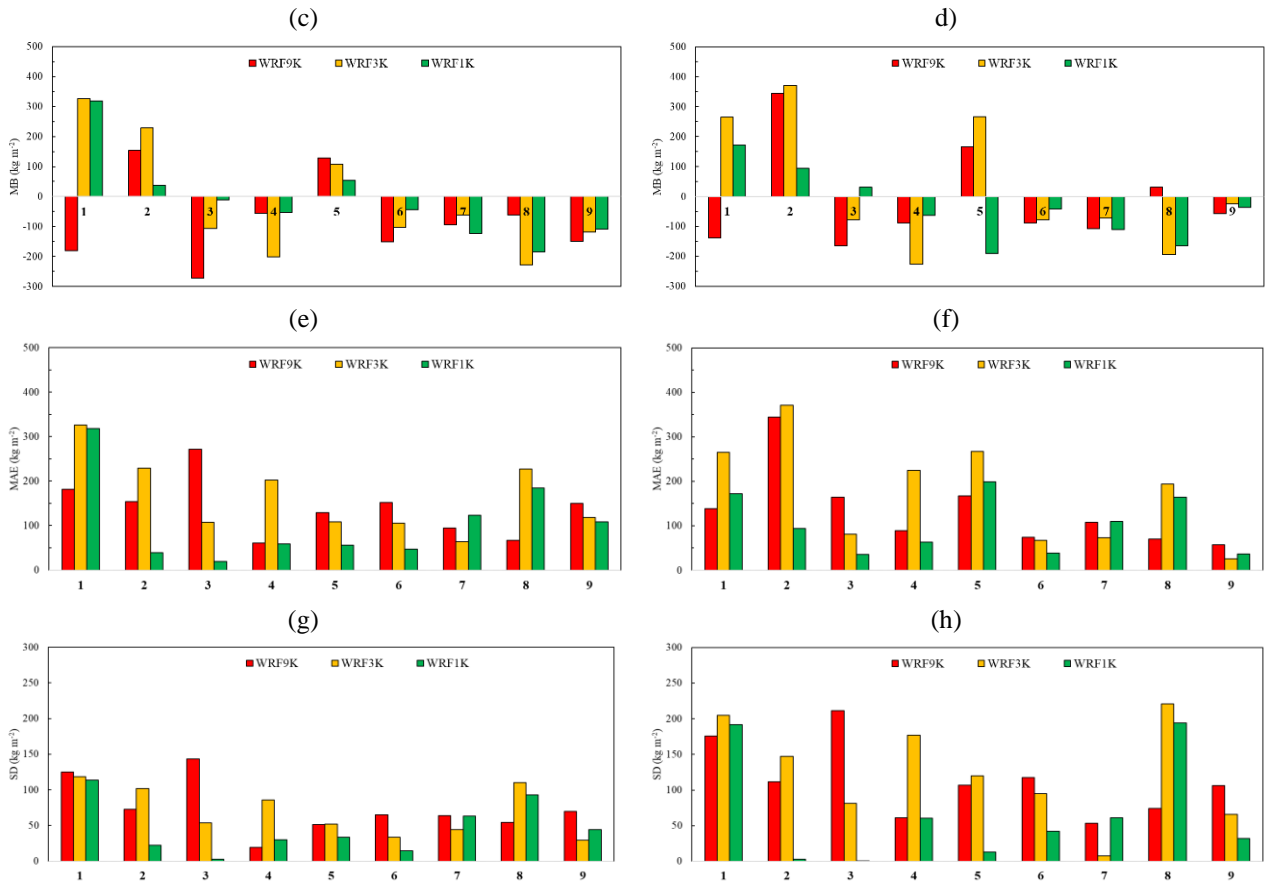
Figure 7. Evaluation metrics for each station including RMSE (a,b), MB (c,d), MAE (e,f) and SD (g,h) for accumulation (left column) and melting (right column) period.
