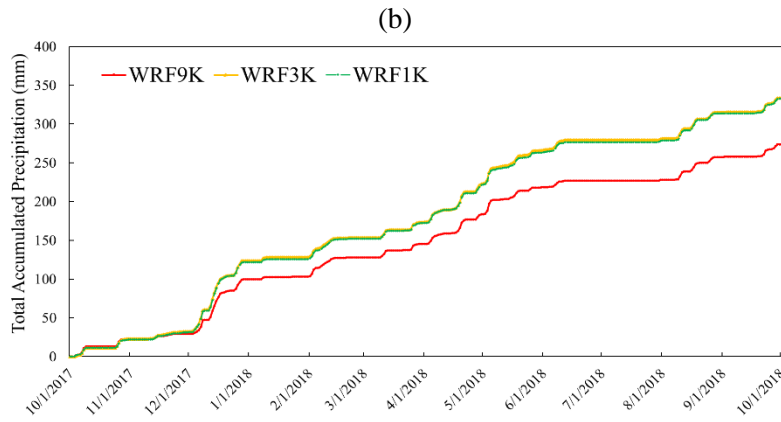
Figure 3. Temporal variation of 2m temperature (a) and precipitation (b) from the three WRF model resolutions over the SSRB region for the innermost domain.
