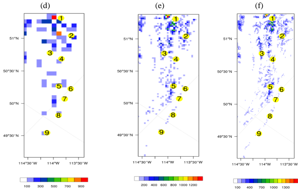
Figure 6. Simulated mean SWE ( \text{kg}/\text{m}^2 ) during the accumulation (1st October 2017- 22nd April 2018) and melting (23rd April 2018 to 1st October 2018) period for WRF9K (a,d), WRF3K(b,e) and WRF1K (c,f) over the inner model domain.
