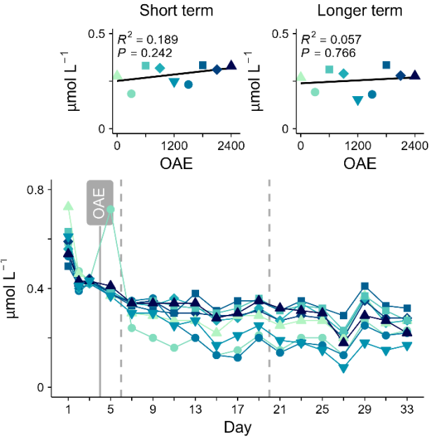
300 Fig. 4: Nutrient concentrations over time and in response to Ocean Alkalinity Enhancement OAE. Open symbols indicate data points excluded from linear regressions.
