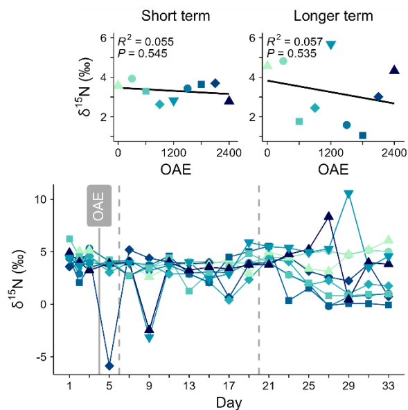
335 Fig. 6: a)-c) Particulate matter stoichiometry and d) stable isotope abundance in particulate nitrogen ( \delta^{15}\text{N} ) over time and in response to Ocean Alkalinity Enhancement (OAE). Horizontal dashed lines indicate the Redfield ratio for each element pair (C:N = 6.6, N:P = 16, C:P = 106).
