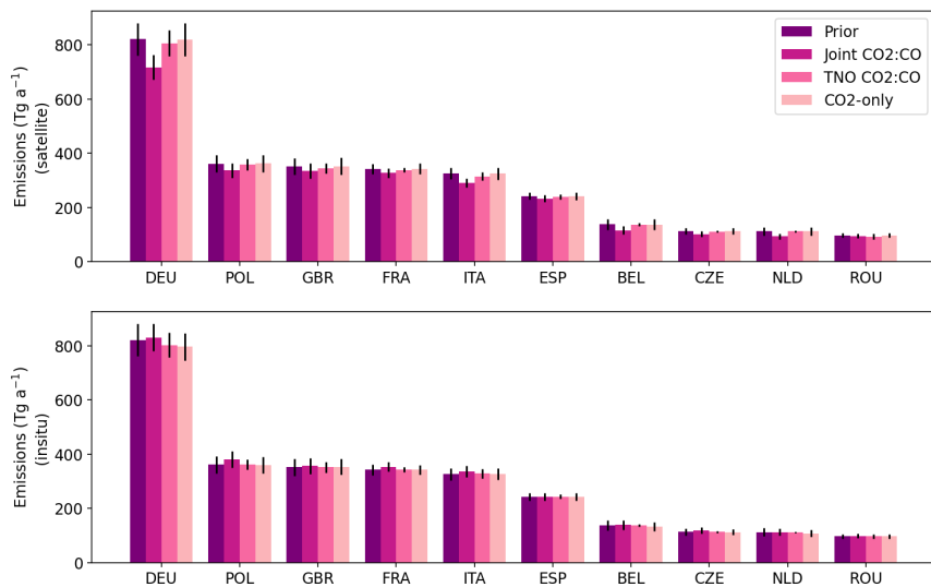
730 Figure 5. Annual mean a priori and a posteriori CO 2 combustion emissions by country for satellite (top) and in situ (bottom) inversions. We show the top 10 emitting countries in our European domain with emissions averaged over 2018-2021. The TNO and joint satellite inversion averages do not include dates prior to July 2018.
