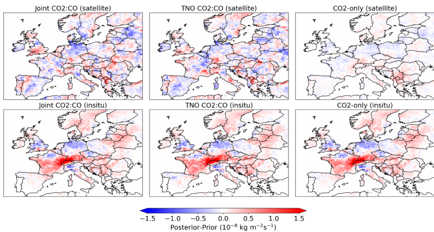
750 Figure 8. As Figure 6 but for non-combustion \text{CO}_2 flux estimates. The TNO and joint satellite inversion averages do not include 2018. The non-combustion emissions include biogenic and non-combustion anthropogenic emission sources.
