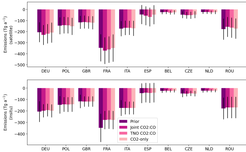
745 Figure 7. As Figure 5 but for non-combustion CO 2 fluxes estimates. The TNO and joint satellite inversion averages do not include 2018. The non-combustion emissions include biogenic and non-combustion anthropogenic emission sources.
