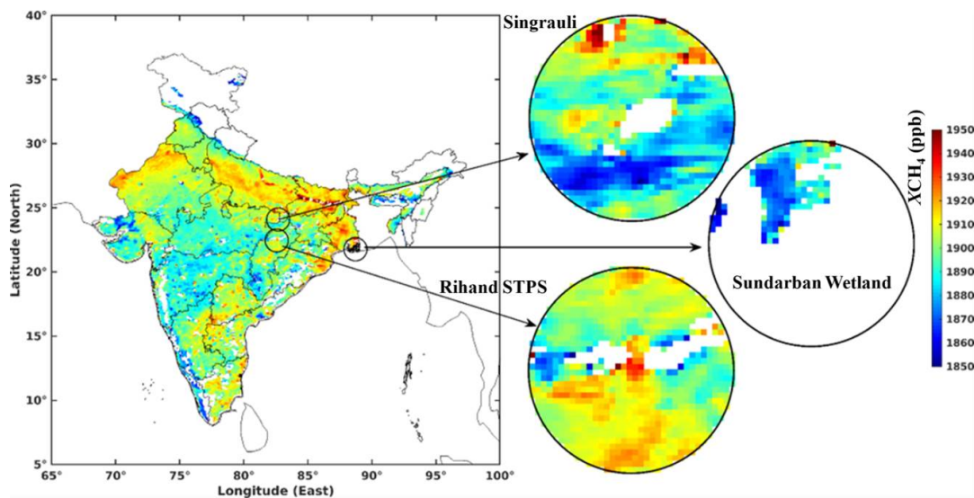
Figure 7. S5P/TROPOMI XCH_4 gridded to 0.05^\circ \times 0.05^\circ over the Indian region and XCH_4 over wetland, coal, and thermal power plant sites with a radius of 100 km.
