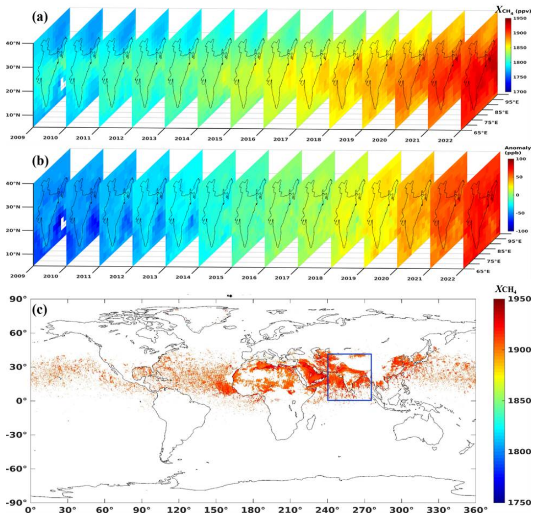
Figure 3. a) Remote Sensing (GOSAT) of atmospheric CH 4 variability over the Indian sub-continent; b) Anomaly during 2009 to 2022; and c) identification of probable high CH 4 concentration using S5P/TROPOMI data from 2019 to 2022 over the study region.
