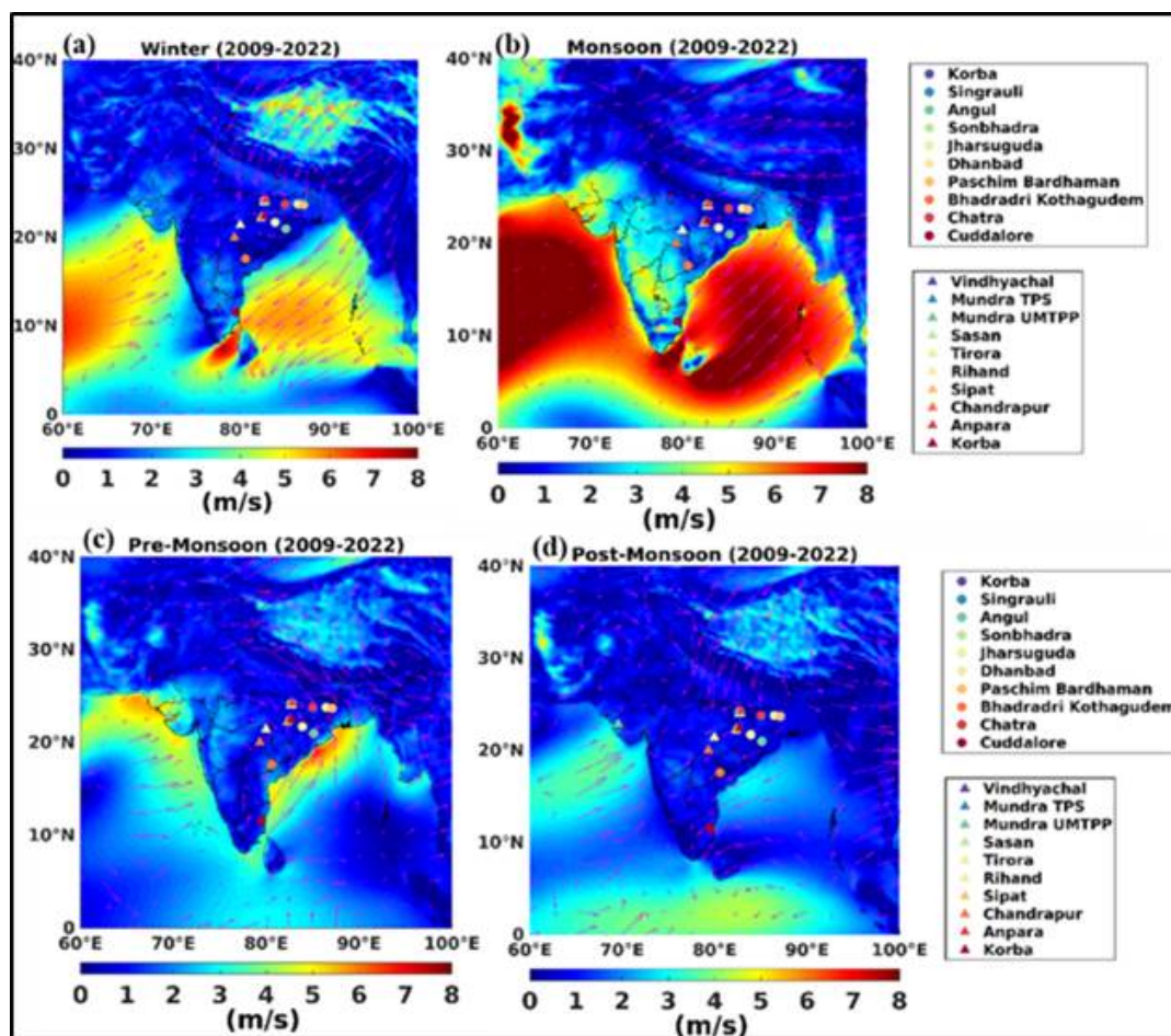
Figure 9. Long-term seasonal winds for source types (coal and thermal power plants) for the period 2009-2022: (a) winter, (b) monsoon, (c) pre-monsoon, and (d) post-monsoon respectively.
