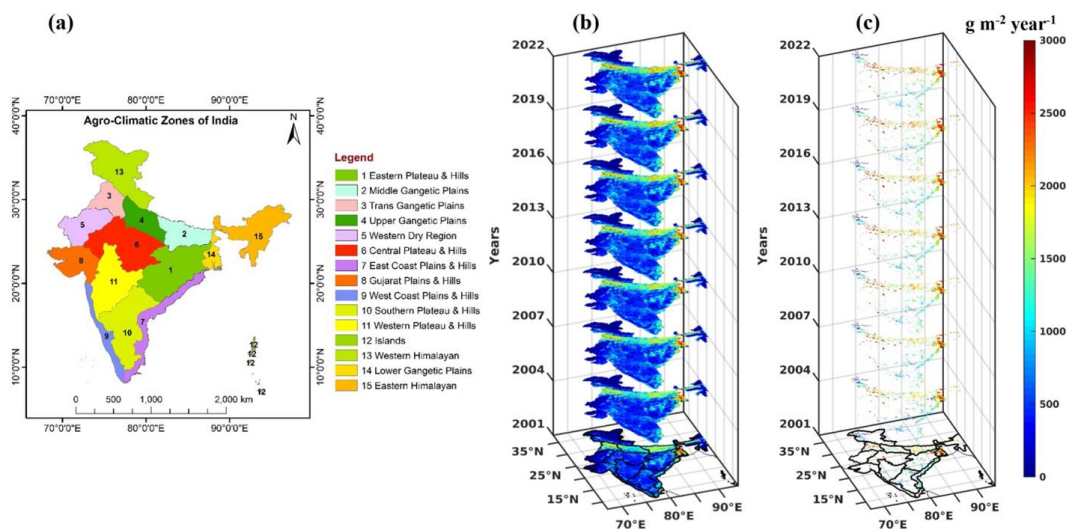
Figure 11. a) Agroclimatic zones of India, b) bottom-up \text{CH}_4 emissions inventory of EDGAR, and c) 90 th percentile statistical filter applied on \text{CH}_4 emissions from 2001 to 2022.
