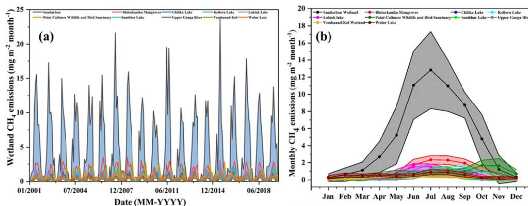
Figure 8. (a) Monthly Time series of Methane emissions ( mg\ m^{-2}\ month^{-1} ) over the wetland sites, (b) Seasonal methane emissions over the wetland sites from 2001 to 2019.
