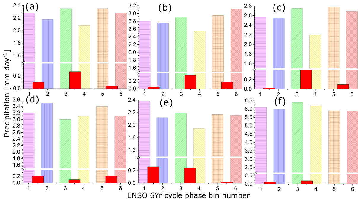
Figure 9. Local ENSO phase effects. Precipitation conditional means in the 6 ENSO phase bins at various coordinates: (a) 36° N 110° E, (b) 33° N 114° E, (c) 36° N 111° E, (d) 33° N 120° E, (e) 36° N 117° E, (f) 28° N 117° E. Red color represents difference between two adjacent bins.
