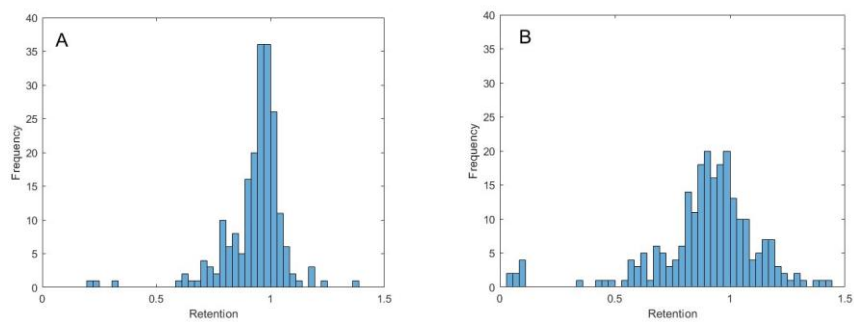
300 Figure 2. Histograms of Retention Coefficients for all measured L5 and above compounds that met peak quality constraints; (A) (-)HESI, (B) (+)HESI
