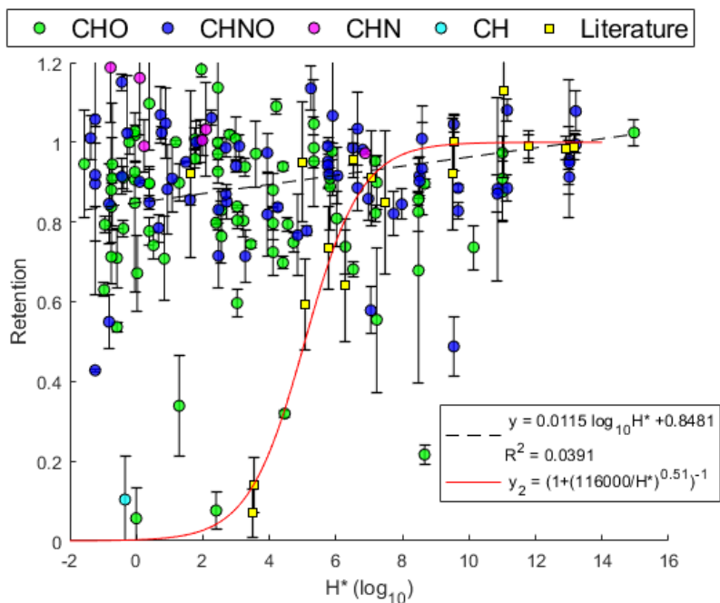
Figure 10. Effective Henry's Law Constant H^* versus Retention Coefficient; Color denotes compositional class of the assigned compound: Green for CHO, blue for CHNO, magenta for CHN, cyan for CH; Yellow squares denote values taken from Borchers et al., (2024), Jost et al., (2017), and Von Blohn et al., (2011, 2013). Dashed line shows linear fit. Solid red line gives the parameterization by Jost et al., (2017).
