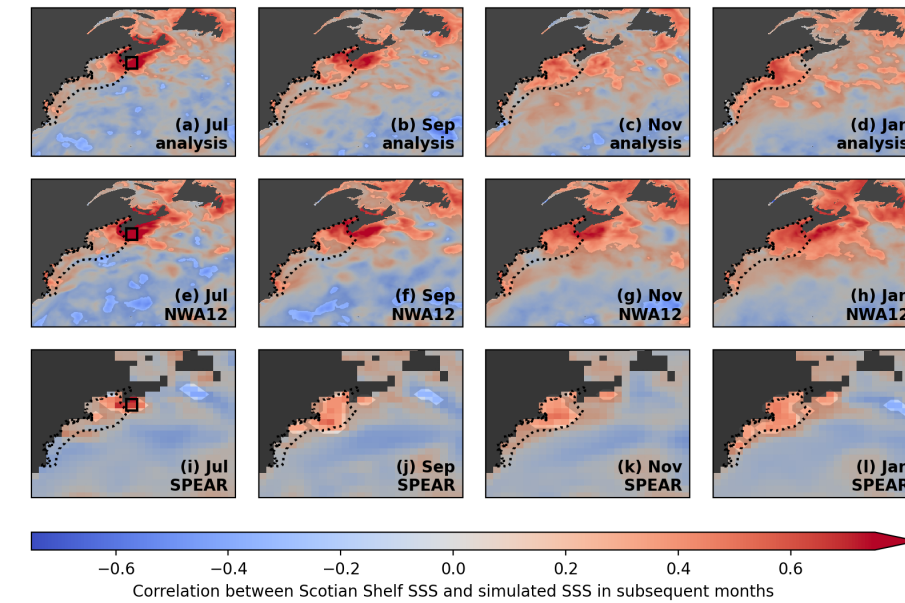
Figure 11. Correlation between June sea surface salinity in the Southwest Scotian Shelf (within the black box in the first panel leftmost panels ) and sea surface salinity in subsequent 1, 3, 5, and 7 months later , from the analysis simulation (a–d), the June-initialized downscaled forecasts (e–h) , and the June-initialized SPEAR forecasts (i–l) . The dotted line lines shows the boundary of the Northeast U.S. LME. Areas overlaid with a light gray shading are not statistically significant at the 90% level using the Bretherton et al. (1999) method.
