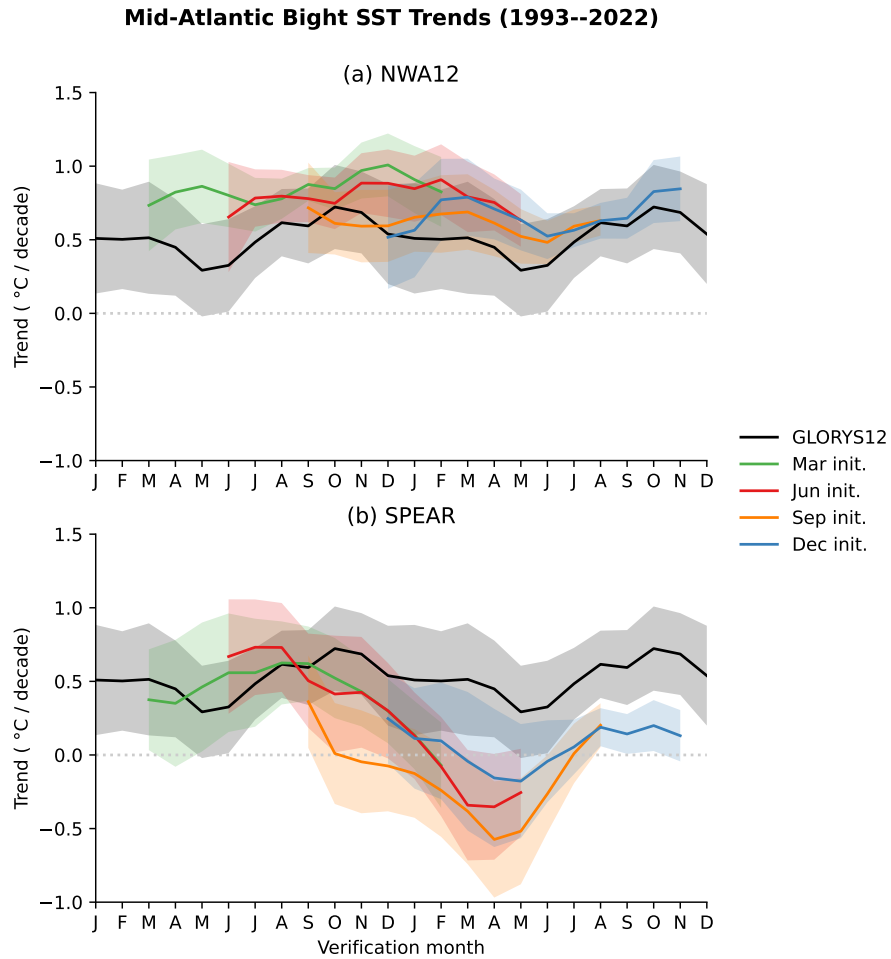
Figure 12. Linear trend of Mid-Atlantic Bight average SST as a function of the forecast initialization month and lead time. Shading denotes 90% confidence intervals.
