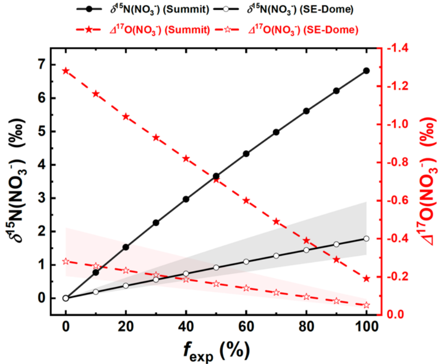
290 Figure 3. Sensitivity of the changes in \delta^{15}\text{N}(\text{NO}_3^-) and \Delta^{17}\text{O}(\text{NO}_3^-) of the ice-core nitrate to f_{\text{exp}} . Positive/negative values indicate deviations from initial deposition. The shaded area in the SE-Dome calculations represents results obtained using snow accumulation rates of 0.6 and 1.4 \text{ m w e a}^{-1} .
