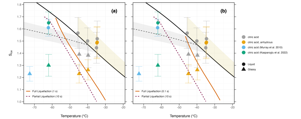
Figure 4: Thermodynamic onset conditions for citric acid ice nucleation and relevant literature as well as humidity-induced phase transitions calculated with the diffusion model. Magenta colored line indicates the modeled partial liquefaction timescale (10 s characteristic residence time of the SPIN) where particle volume has increased by more than 5 % due to water uptake. Orange lines indicate two modeled full liquefaction timescales where citric acid is expected to be fully liquefied within 1 s (a) or 0.1 s (b) after entering the SPIN. Shapes correspond to aerosol phase state as reported in literature or defined using methods described above (e.g. PCU temperature lower than T_{p,0.02} and ice nucleation observed below homogeneous freezing threshold). Black dashed line is the homogeneous freezing threshold of 0.1\text{ }\mu\text{m} diameter solution droplets (Koop et al., 2000) with shaded region indicating uncertainty in a_w of \pm 0.025 (Koop, 2004). Solid black line is water saturation with dashed gray lines denoting equivalent lines of various liquid saturation ratios. Shaded yellow region indicates expected droplet breakthrough regime within the SPIN.
