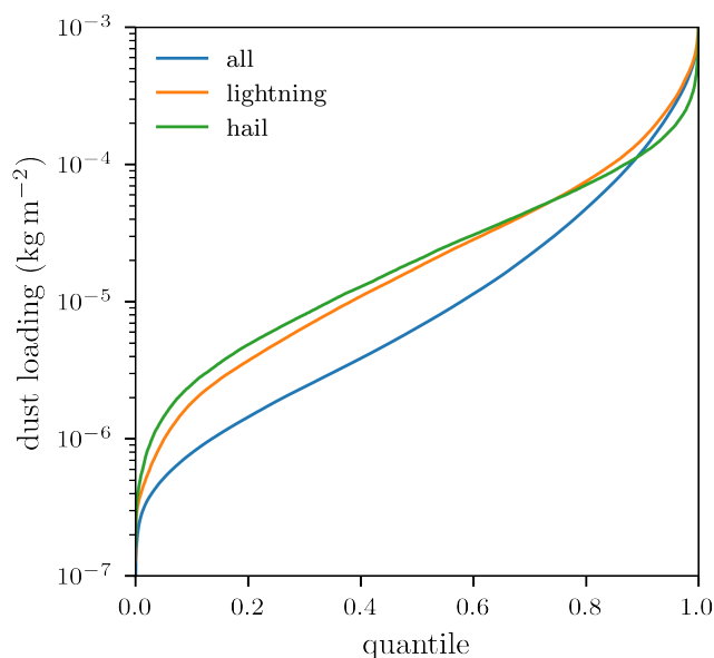
Figure A1. Quantiles from the local JJA dust loading climatology throughout the study domain and period (see Sect. 2 for specifics, CAMS vertically integrated mass of dust aerosol 0.03–20 μm), for all days (blue), thunderstorm days (orange) and hail days (green).
