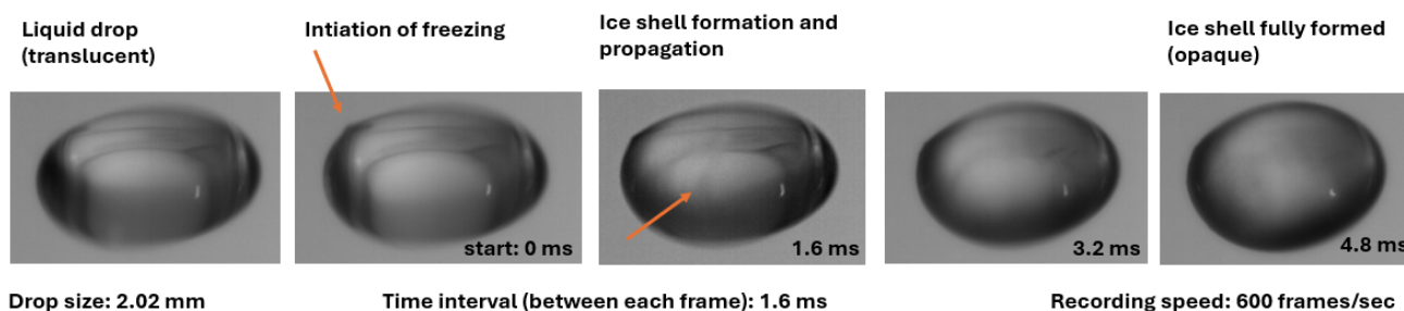
Figure B1. Consecutive frames showing the formation of ice-shell, recorded with a high speed camera at 600 frames per second, and at a cold room temperature of -15 °C. In the liquid phase (leftmost image), the drop is seen as translucent, which gradually turns opaque as the ice shell is formed (rightmost image).
