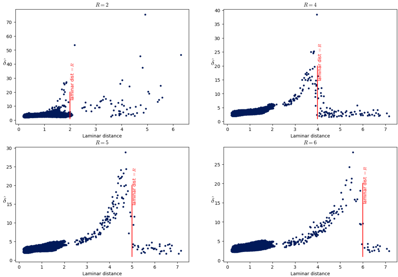
Figure B2. Same as Fig. 11 but for the Lorenz 96 system with n = 12 and F = 4.4 ( 10^5 points in the trajectory). The vertical red lines mark the value of the laminar distance which is equal to the radius R .
