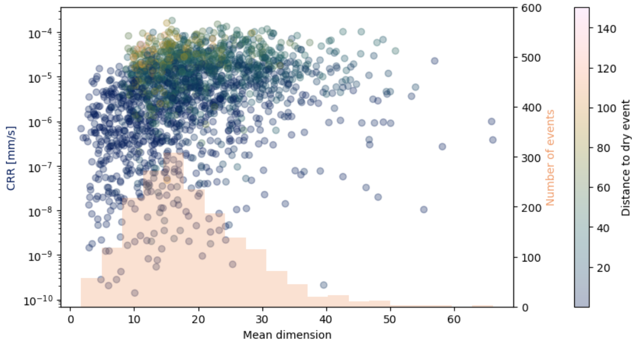
Figure 19. Histogram of the repartition of the mean dimension for our 2000 computation points (in orange) and scatter plot of this mean dimension with the CRR (in color scale). The color is the distance to the dry event.
