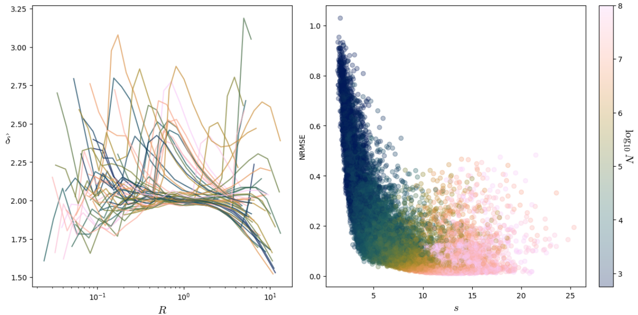
Figure 9. Left: Plot of \hat{\delta} versus R for 50 points of the Lorenz 63 system ( \rho = 28 ) with a trajectory of 10^7 points. Only fits with \text{NRMSE} < 0.4 , s > 5 are plotted. Right: scatter plot of \text{NRMSE} vs s for the same dataset, but for all 1000 computation points. The color represents the logarithm of the number of points used in the dimension estimation.
