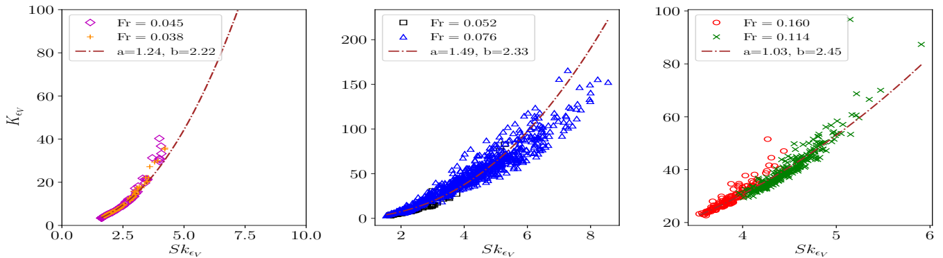
Figure 1. Stratified turbulence: Flatness-skewness plots for \epsilon_v for several Froude numbers (see insets with Fr and (a, b) parameters assuming a fit F \sim a * S k_{\epsilon_v}^b . Note the different scales on the axes, and in particular the high flatness values for the run with Fr \approx 0.076 (middle).
