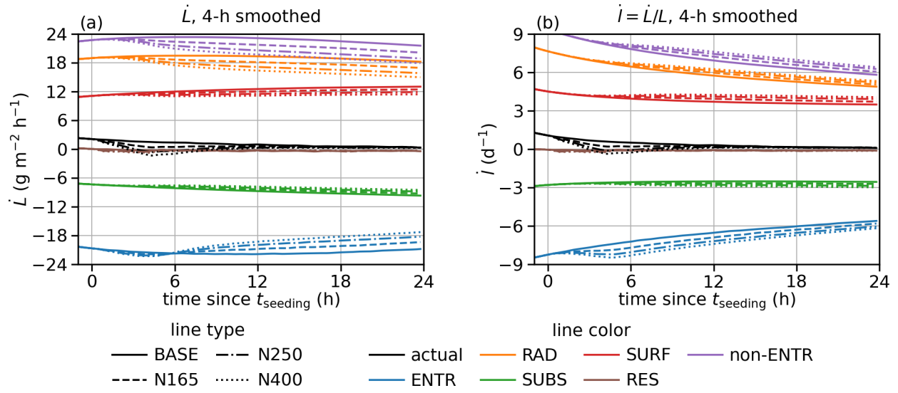
Figure 5. Same as Figure 3 but for (a) L budget and (b) l budget.
