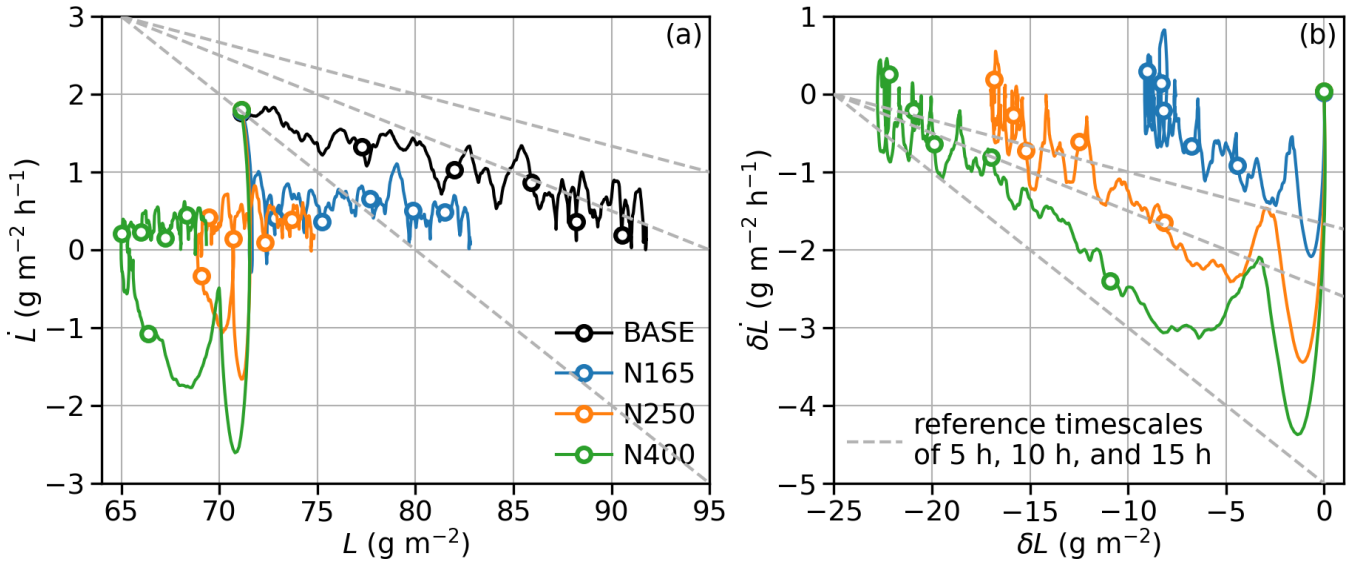
Figure 7. (a) Trajectories starting from t_{\text{seeding}} = 12 h, averaged across simulations for BASE, N165, N250, and N400, in the L-\dot{L} plane. All trajectories start around (71 \text{ g m}^{-2}, 1.8 \text{ g m}^{-2} \text{h}^{-1}) . Circles are 4 h apart from t_{\text{seeding}} to 20 h since t_{\text{seeding}} . (b) Same as Panel (a) but in the \delta L-\delta \dot{L} plane, where “ \delta ” indicates the deviation from BASE. All trajectories start around (0 \text{ g m}^{-2}, 0 \text{ g m}^{-2} \text{h}^{-1}) . For both panels, gray lines indicate the slopes for reference timescales of 5 h (the steepest one), 10 h, and 15 h (the least steep one).
