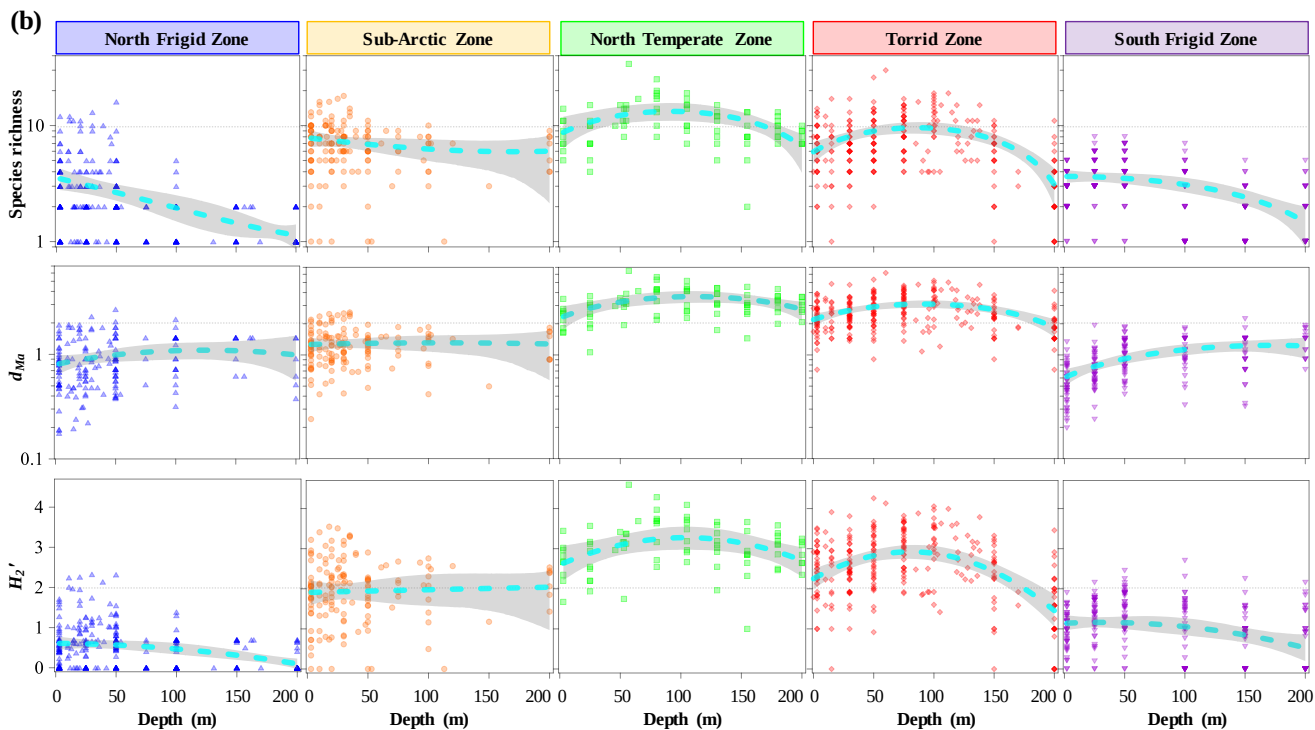
220 Figure 5: Variations of tintinnid species richness, Margalef index ( d_{Ma} ) and Shannon index ( H_2' ) in latitudinal (a) and vertical (b) direction of all regions.
