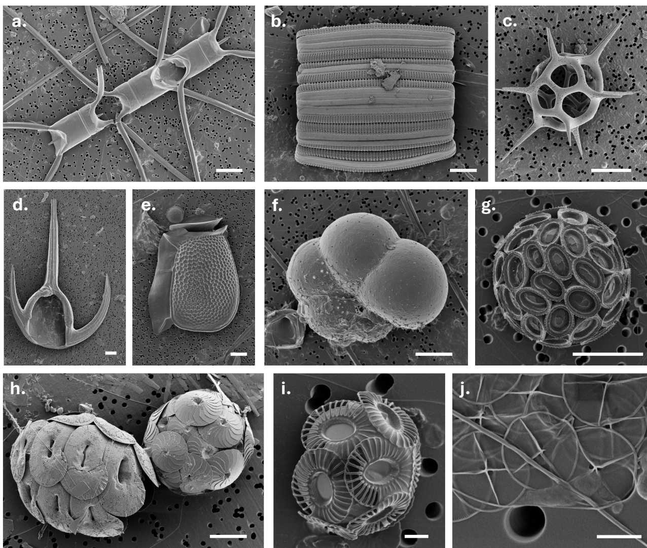
Figure A3. Scanning Electron Microscopy (SEM) images showing a range of taxonomic groups in samples from the SOTS site. a) centric diatom Chaetoceros atlanticus ; b) pennate diatom Fragilariopsis doliolus ; c) silicoflagellate Dictyocha speculum ; d) dinoflagellate Tripos azoricus ; e) dinoflagellate Dinophysis truncata ; f) foraminifera; g) coccolithophorid Coronosphaera cf mediterranea ; h) coccolithophorids Helicosphaera carteri (left) and Calcidiscus leptoporus (right); i) coccolithophorid Emiliana huxleyi calcification morphotype B/C; j) haptophyte scales from a species of Chrysochromulina . Scales bars are 10 \mu\text{m} (a – f), 5 \mu\text{m} (g, h) and 1 \mu\text{m} (i, j). All images by R. Eriksen.
