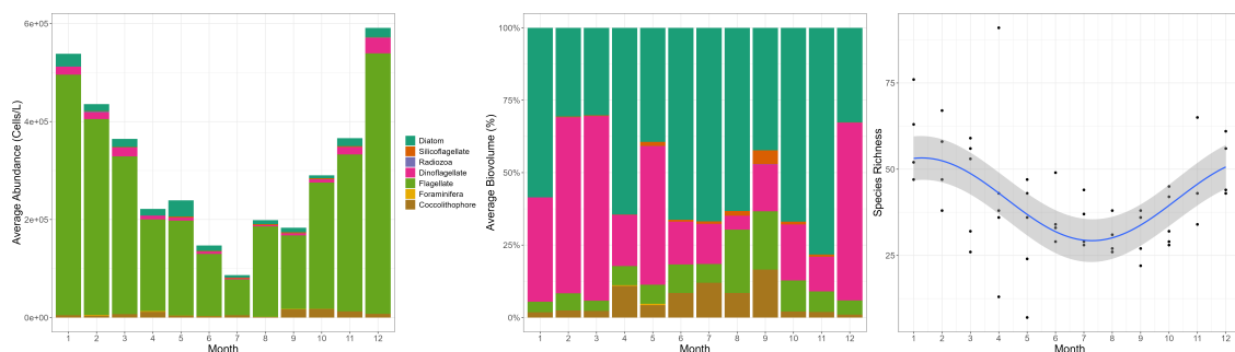
Figure 11. Climatological seasonality of phytoplankton and microplankton community composition at the STOS site. a) abundance; b) biovolume; c) species richness. The colours in panels a and b indicate the dominant taxa.
