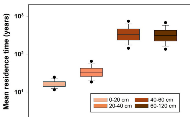
Figure 7. Distributions of mean residence times for SOM calculated in the sensitivity analysis for four depths in the soil profiles of production area P04 in east-central Sweden. Horizontal lines show median values, the box defines the inter-quartile range, error bars define 10 th and 90 th percentiles and solid symbols indicate 5 th and 95 th percentiles.
