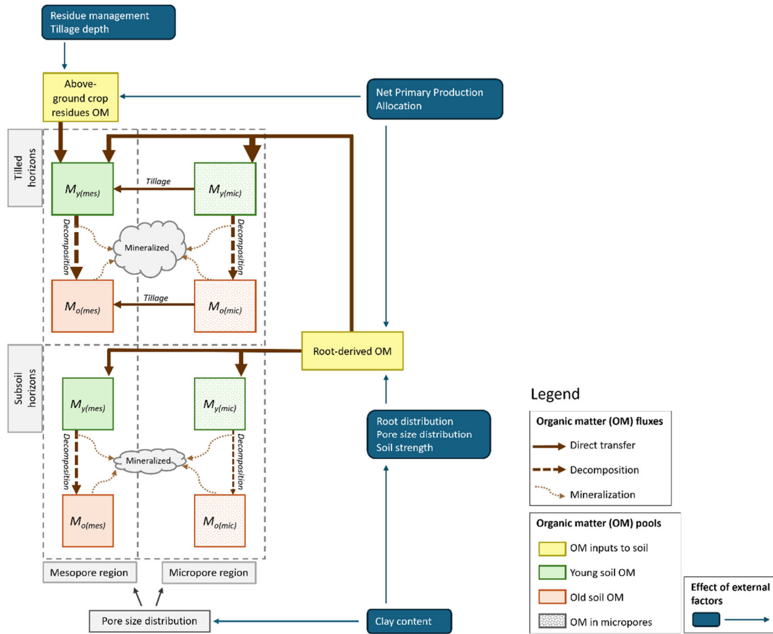
Figure 1. Schematic diagram of the organic matter (OM) pools ( M = mass, Y = young; O = old ) and fluxes and of the main external factors affecting OM inputs to the soil (for definitions see equations 1 to 6, 10 to 13 and 20 to 24). The grey boxes with dashed lines indicate tilled and subsoil horizons in the soil profile, both partitioned between two pore regions (micropores and mesopores). This partitioning is estimated from the soil clay content using pedotransfer functions (equations 10 to 13). OM located in the micropores is partially physically protected from decomposition (by a factor F_p see equations 3 and 4). In tilled horizons, OM from the above-ground crop residues is added only to the mesopore region and a fraction of OM located in the micropores is transferred by tillage. Root-derived OM is added to both pore regions as a function of pore size distribution and soil strength through effects on root distribution in the soil profile (see equations 21-24). The sizes of the boxes and arrows illustrate that OM contents and fluxes are generally smaller in subsoil as a result of lower OM inputs, which, in turn, leads to greater energy limitation (equations 5 and 6).
