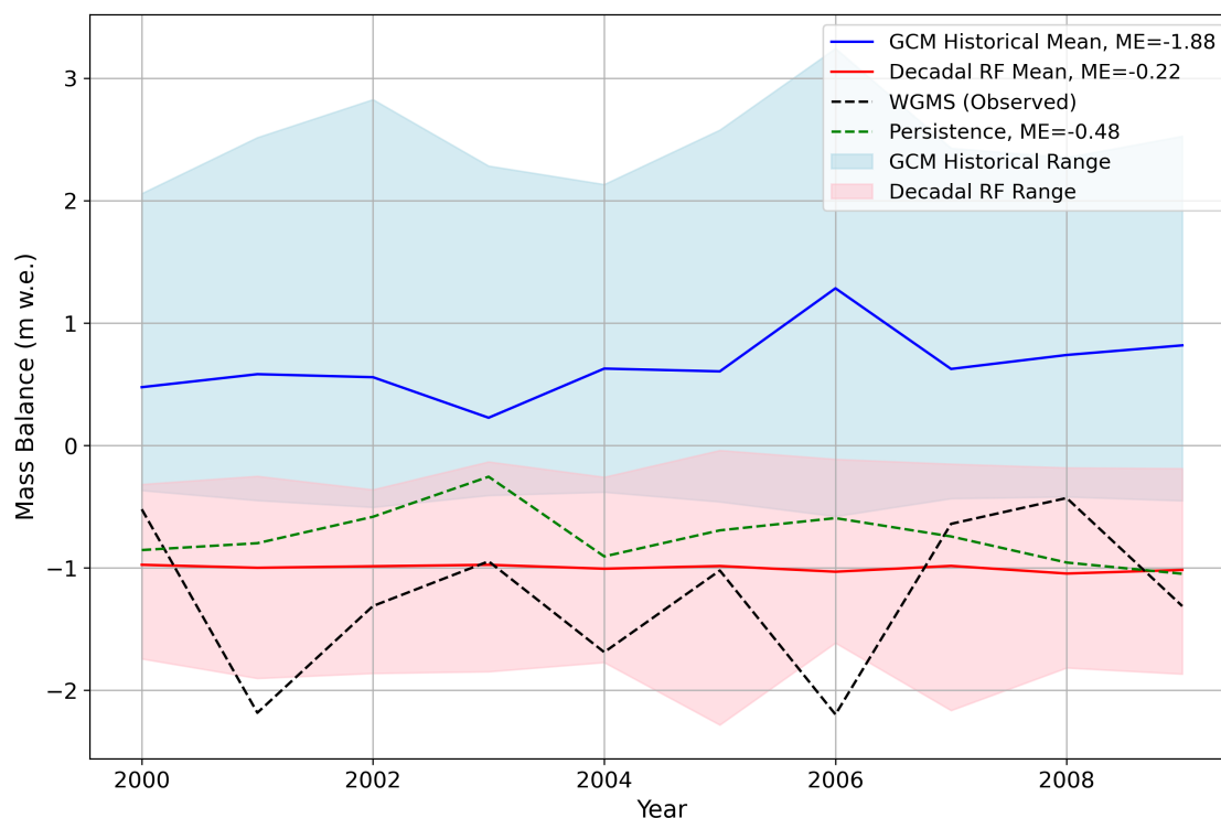
Figure A2. Single glacier result example for the Langfjordjoekulen, Norway. Mean errors (ME) for the different experiments, for mean mass balance over the decade, as in Table 2, are indicated in the legend. This means the difference between the mean observed mass balance and the mean simulated mass balance for the different experiments. For the GCM historical and decadal RF experiments, ‘simulated’ refers to the ensemble mean.
