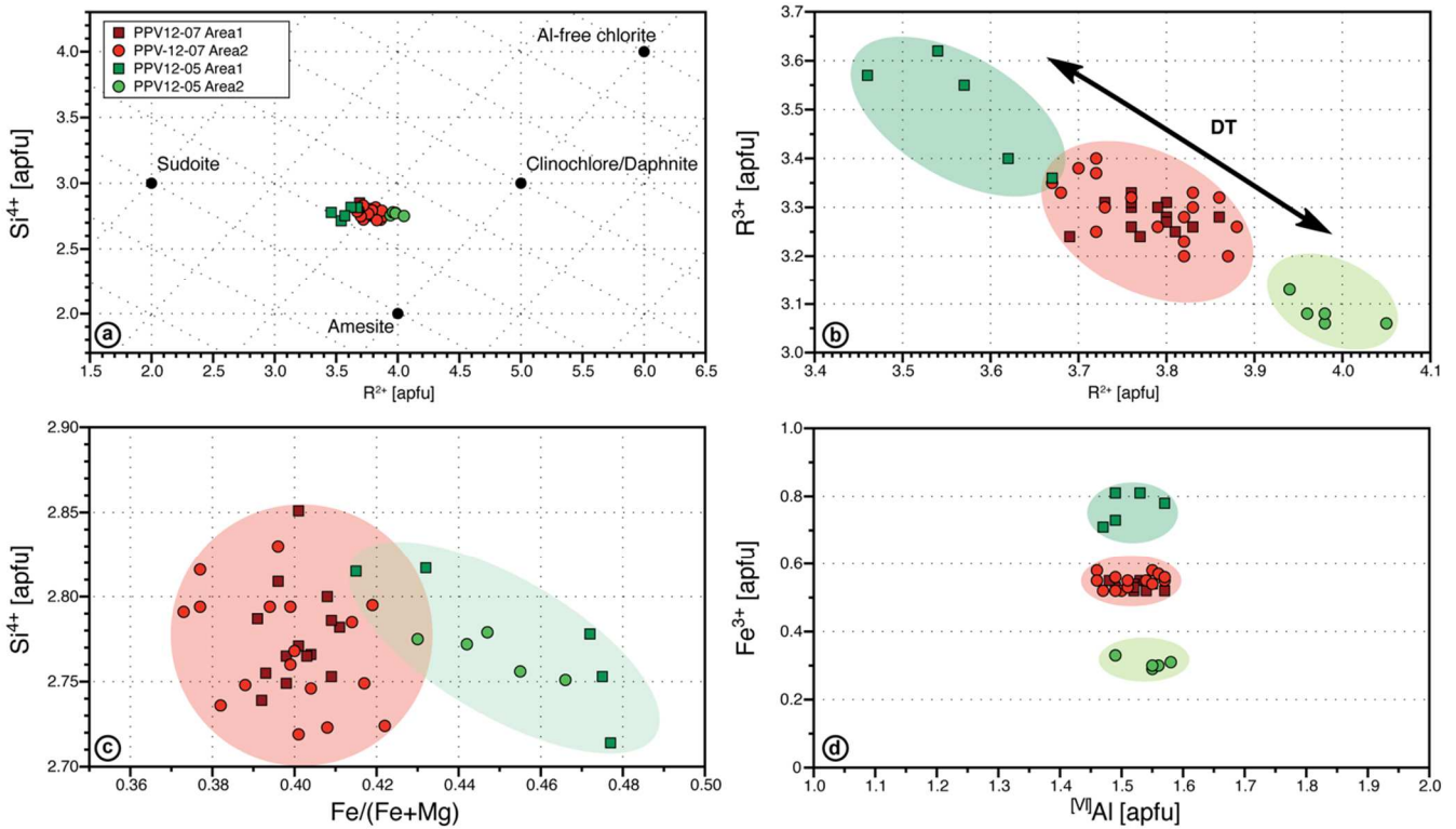
350 Figure 8. Structural formulas values of synkinematic chlorite from the damage zone in red (sample PPV12-07) and from the core zone in green (sample PPV12-05), squares for Area 1 and circles for Area 2 (cf. to Figs. 5 and 6 for analyses location). The graphs show a: Si vs. R^{2+} , b: R^{3+} vs. R^{2+} , c: Si vs. Fe_{total}/(Fe_{total}+Mg) , and d: Fe^{3+} vs [VI]Al diagrams. Note that R^{2+} refers to divalent cations ( Fe^{2+} and Mg^{2+} ), and R^{3+} refers to trivalent cations ( Al^{3+} , Fe^{3+} ). Fe is regarded as total iron, i.e., Fe^{2+} and Fe^{3+} . apfu: atoms per formula unit, [VI]Al : aluminium in octahedral sheets. 355
