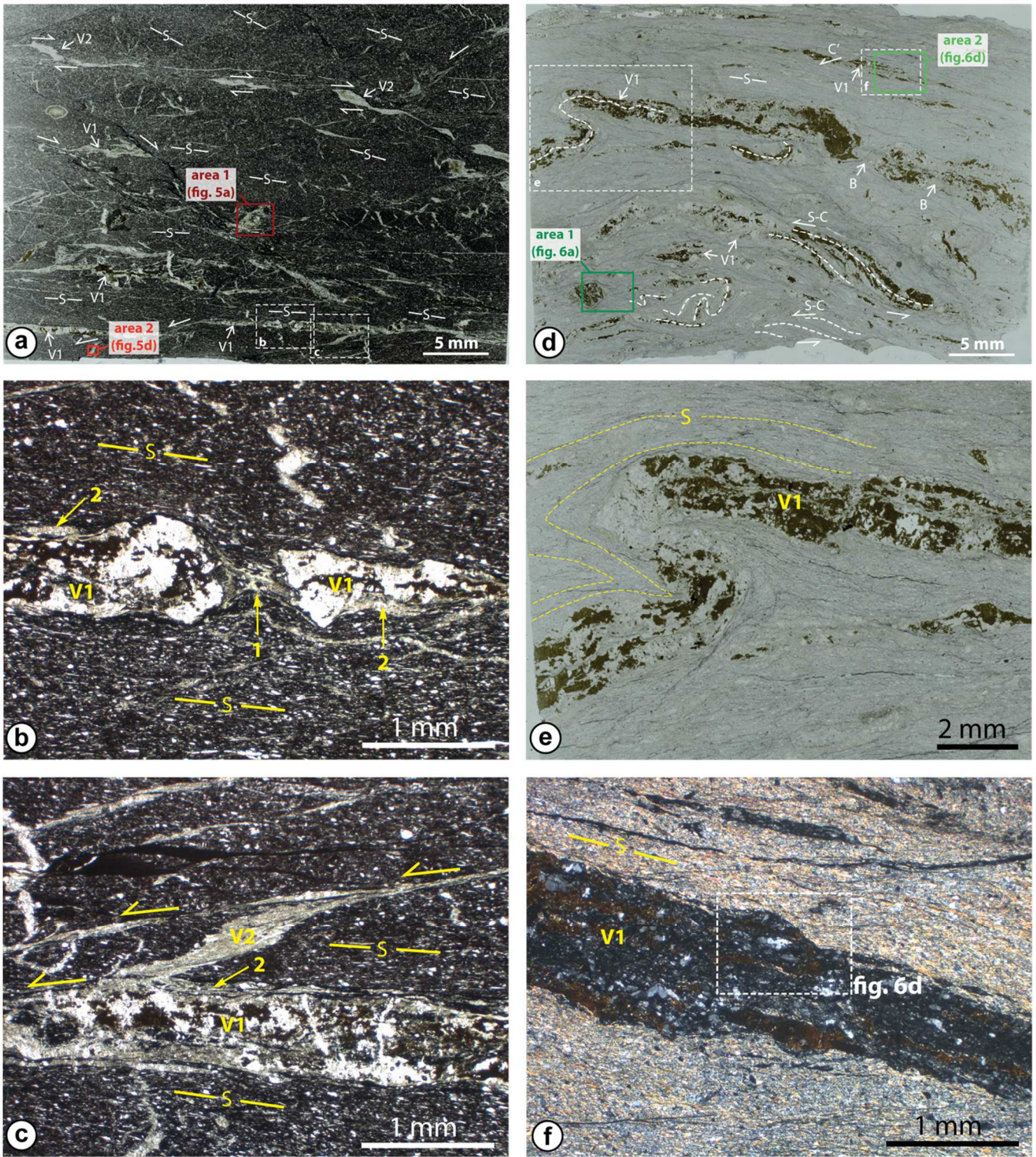
265 Figure 4. Scan images of the studied thin-sections in the Triassic rocks of the thrust fault hanging wall showing detail of microstructures. a to c: PPV 12-07 sample from the damage zone. a: Early, schistosity-parallel quartz veins featuring iron oxide patches are stretched by boudinage and cross-cut by younger shear surfaces (arrows). A second generation of quartz + chlorite veins occurs in releasing oversteps along shear surfaces. b: Boudinage of an early, schistosity-parallel quartz vein with iron oxide patches, with quartz + chlorite precipitation in the interboudin and along the early vein. c: Late quartz + chlorite vein in a releasing overstep 270 along shear surfaces (arrows) and quartz + chlorite precipitation along the early vein. d to f: PPV 12-05 sample from the core zone. Same early, schistosity-parallel veins as in a are stretched by boudinage, folded and involved together with schistosity in S-C shear structures. Fold asymmetry and S-C structures indicate top-to-left (south) shearing C. Folded early, schistosity-parallel quartz vein. d: Early vein with mylonitized quartz fill. e: quartz + chlorite precipitated in interboudin opening. f: quartz + chlorite precipitated 275 along early quartz vein. Frames localize detail pictures in Figures 5 and 6. B: boudinage; C, C': shear surfaces; S: schistosity; V1: early, schistosity-parallel quartz veins; V2: younger quartz + chlorite veins in releasing oversteps along shear surfaces.
