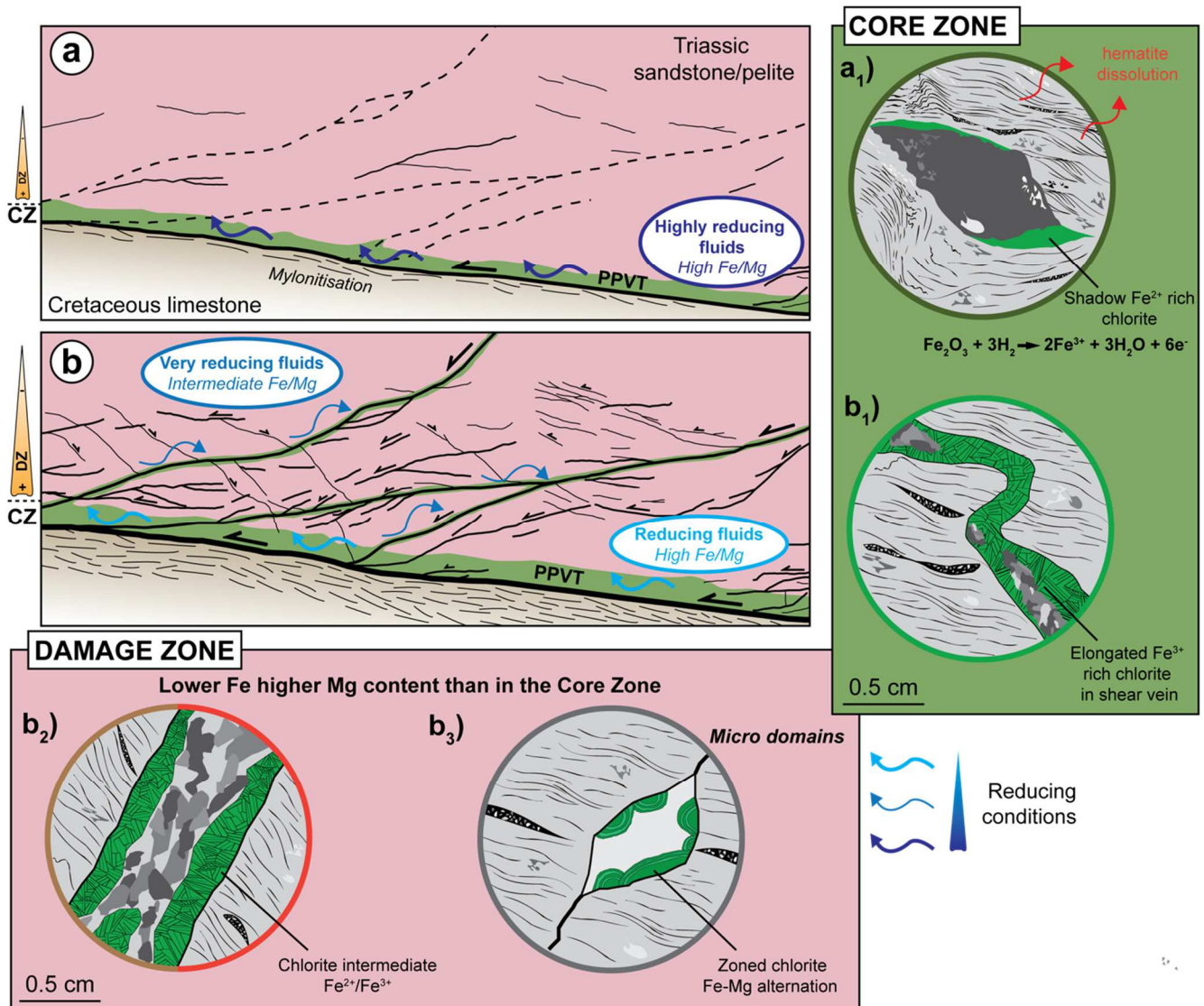
Figure 10. Schematic PPVT fluid circulations and chemical transfers. a Percolation of a highly reducing fluid along the thrust fault leading to the dissolution of hematite and the crystallization of the Fe 3+ -rich chlorite a 1 . b Transformations of the initial fluid and circulation of the modified fluid leading to the crystallization of the elongated chlorite b 1 in core zone and to the chlorites of the damage zone b 2 and b 3 .
