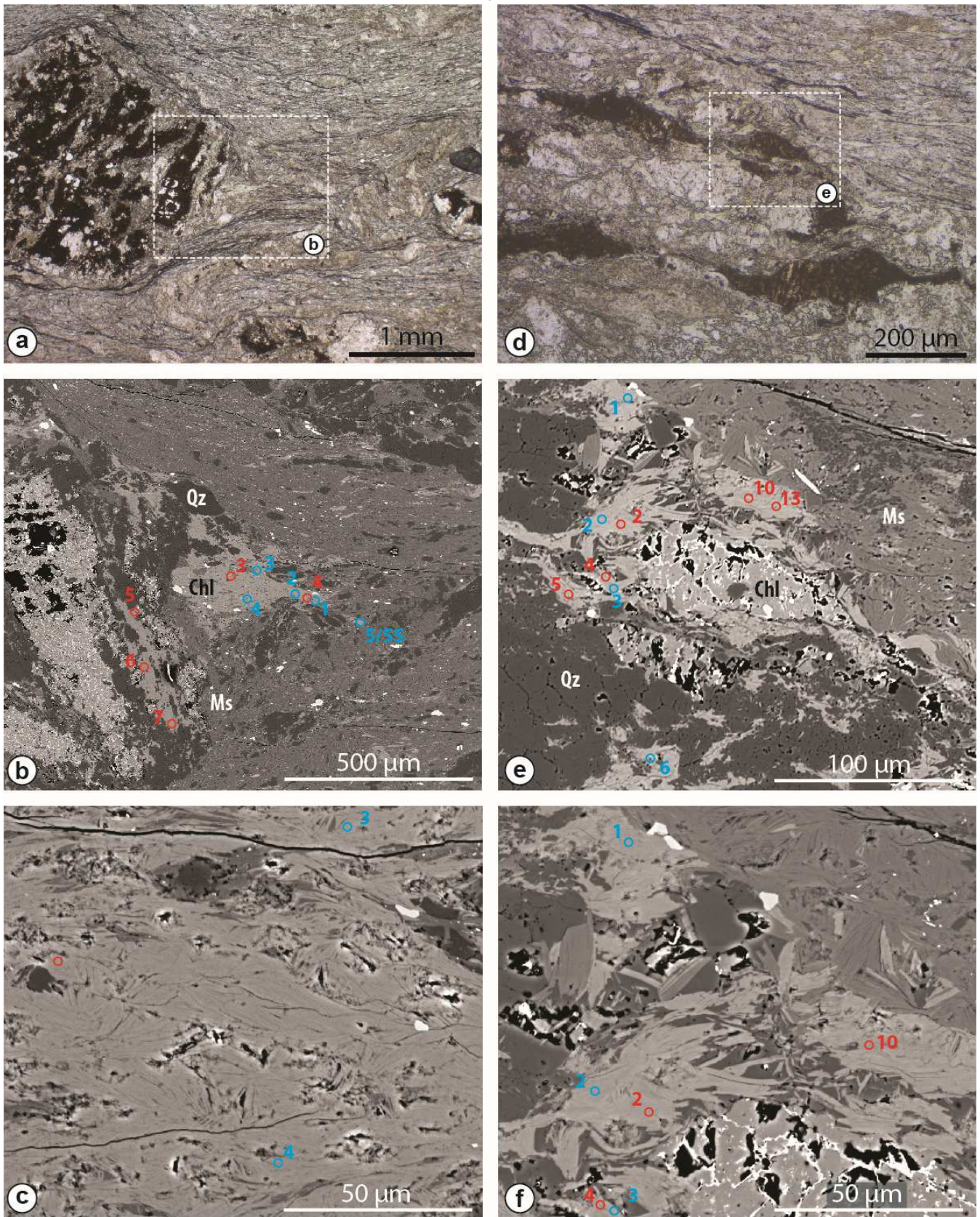
285 Figure 6. Location of analyses on PPV12-05 sample from the core zone. a to c Area 1 in Fig. 4d. a Thin-section scan image showing boudinage and schistosity-parallel quartz vein with oxide patches; Quartz + chlorite precipitated in the interboudin opening and in high angle extension veins across the early quartz vein. b SEM image showing chlorite in the strain shadow at the edge of boudinage opening (cf. frame in a). The location of the \mu -XANES analyses is in blue, and the microprobe analyses are in red. c Detail of the chlorite particles morphology. d to f Area 2 in Fig. 4d. d Optical microscope image showing an early, schistosity-parallel quartz vein 290 deformed by shear bands with mylonitized quartz and chlorite precipitation. e SEM image showing chlorite located at the edge of a shear vein of quartz + chlorite (cf. frame in d). The location of the \mu -XANES analyses is in blue, and the microprobe analyses are in red. f Detail of chlorite particles morphology. Elongated chlorite particles are imbricated with quartz grains.
