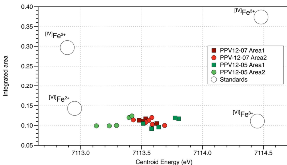
Figure 7. Integrated area versus centroid position variogram showing the positions of standards (Andradite for [\text{VI}]\text{Fe}^{3+} , Sanidine for [\text{IV}]\text{Fe}^{3+} , Sauroilite for [\text{IV}]\text{Fe}^{2+} , Siderite for [\text{VI}]\text{Fe}^{2+} ), together with the data from chlorite particles from the damage zone in red (sample PPV12-07) and from the core zone in green (sample PPV12-05), squares for Area 1 and circles for Area 2 (cf. to Figs. 5 and 6 for analyses location). [\text{VI}]\text{Fe} : iron in octahedral sheets; [\text{IV}]\text{Fe} : iron in tetrahedral sheets.
