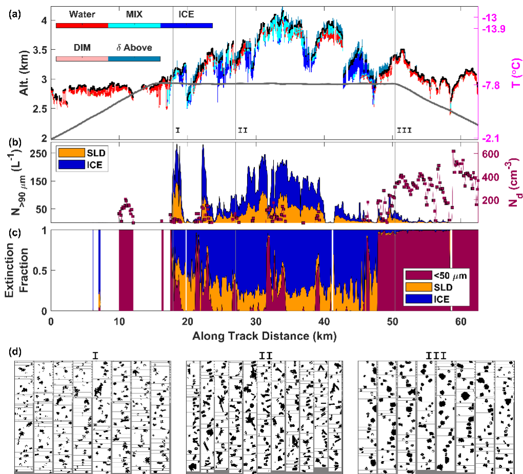
775 Figure 6: An ACTIVATE flight segment from February 28, 2020, showing the matched King Air and Falcon cloud data. (a) HSRL phase categorization (colors), cloud top height (black), Falcon flight track (grey) and a nearby dropsonde used to provide the temperature scale highlighting the inversion structure (right axis). (b) Number concentrations of microphysical classes: droplets ( < 50 \mu m ), supercooled large drops (SLD; > 90 \mu m ) and ice ( > 90 \mu m ). (c) Extinction fraction of microphysical classes for periods in cloud. (d) Selected samples of 2D-S particle imagery corresponding to the locations marked in (a).
