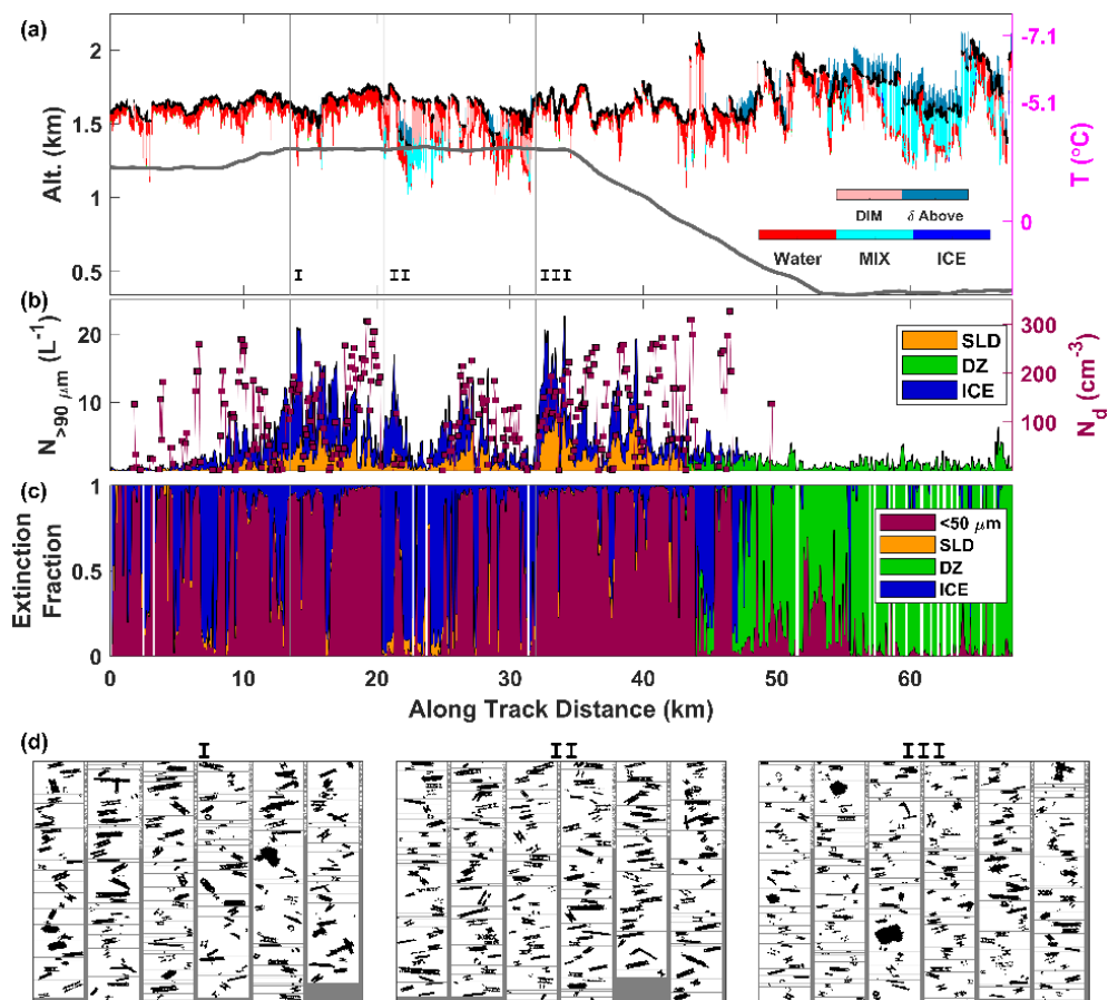
785 Figure 8: As Figure 6, but for a flight segment on January 27, 2022. Note that Falcon classes also include the drizzle (DZ) class substituting SLD for altitudes lower than 0°C.
