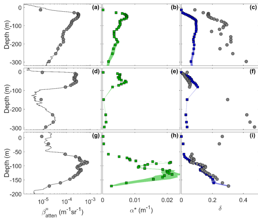
Figure 4: As Figure 3 but for (a-c) a mixed phase profile, (d-f) a profile with liquid-dominant conditions above ice-dominant, 765 (g-i) a profile with ice-dominant conditions above liquid-dominant
