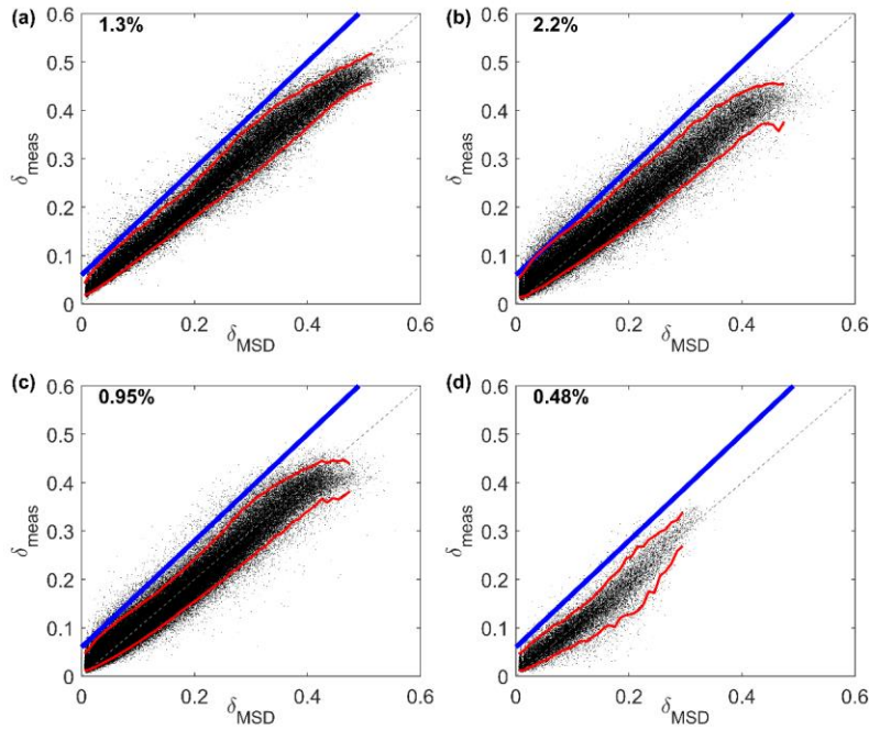
Figure 5: Comparison of the MSD modelled with the measured \delta for control cases (a) CPEX, (b) ACTLOW1, (c) ACTLOW2, and (d) ACTHIGH. In each panel a 1:1 line is included (grey dash), 5% and 95% bounds in the measured \delta for increments of MSD (red), the boundary of the WATER-MIX classifications (blue), and the false positive fraction in the upper left.
