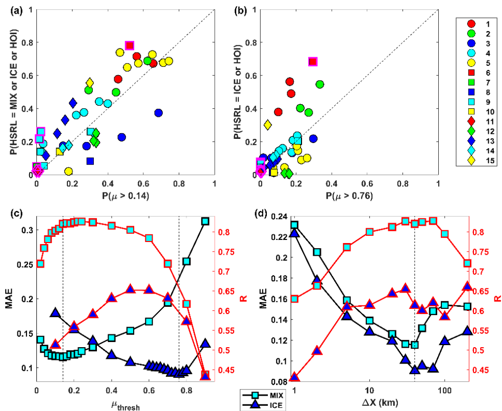
Figure 10: Comparison of the frequency of (a) ice-containing HSRL categories (MIX, ICE, HOI) and (b) ice-dominant categories (ICE, HOI) with the frequency of Falcon observations that exceed an ice extinction fraction of 0.14 and 0.76, respectively. Each comparison point represents a subsegment (see text) of a matchup cloud scene where the scene indices (Table 3) are shown in the legend. (c) Sensitivity of the ice extinction fraction thresholds, as assessed by the mean absolute error (MAE) and correlation coefficient (R) of the data shown in (a) and (b). (d) Sensitivity of the subsegment length ( \Delta X ) when the ice extinction fraction thresholds are held at their optimal values.
