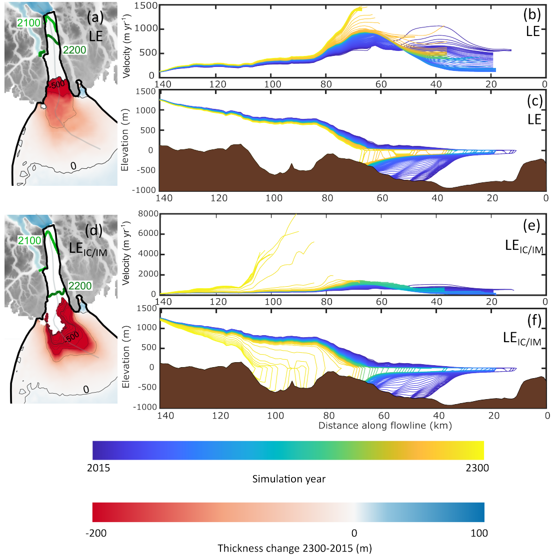
Figure 4. Changes in front position, velocity, and ice thickness from LE (a to c) and LE_{IC/IM} (d to f). The thickness change between 2015 and 2300 is shown in panels a and d, where the front positions in 2100 and 2200 are shown. The front position in 2300 corresponds to the limit of the thickness change map. Contours of thickness change are also shown, with thin lines denoting 100m of change and the bold lines denoting 500m of change. Panels b and e show velocity along a flowline with time (note the different y axes scale), and panels c and f show glacier geometry along a flowline with time. The flowline follows the retreating glacier front and is shown as a pale grey line in panels (a) and (d). Bedrock topography, bathymetry, and ice mask data is from BedMachine v5 Morlighem et al. (2017).
