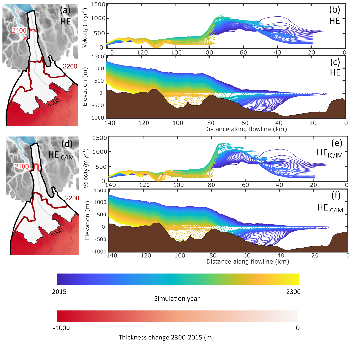
Figure 5. Changes in front position, velocity, and ice thickness from HE (a to c) and HE IC/IM (d to f). The thickness change between 2015 and 2300 is shown in panels a and d, where the front positions in 2100 and 2200 are shown. The front position in 2300 corresponds to the limit of the thickness change map. Contours of thickness change are also shown, with thin lines denoting 100m of change and the bold lines denoting 500m of change. Panels b and e show velocity along a flowline with time, and panels c and f show glacier geometry along a flowline with time. The flowline follows the retreating glacier front and is shown as a pale grey line in panels (a) and (d). Note that the thickness change scale is different than that used in Fig. 4. Bedrock topography, bathymetry, and ice mask data is from BedMachine v5 Morlighem et al. (2017).
