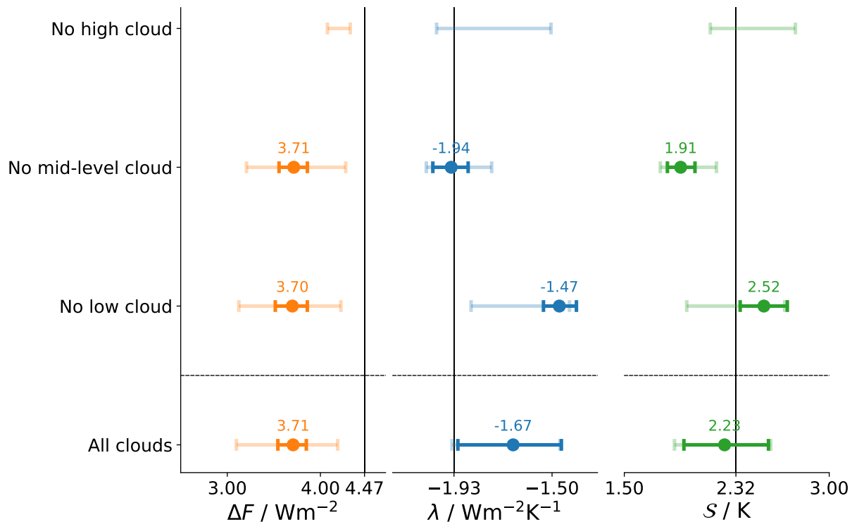
Figure 4. Distribution of the adjusted radiative-forcing \Delta F , the climate feedback parameter \lambda , the equilibrium climate sensitivity \mathcal{S} . The faded lines depict the 5 %–95 % interval of all possible CRE values in the full ensemble. The bold lines show the same range, but for a plausible subsample that is in agreement with satellite observations. Different “rows” of the figure show results for different simulations, in which certain cloud layers were turned off (e.g. the first for describes a simulation with all but high clouds).
