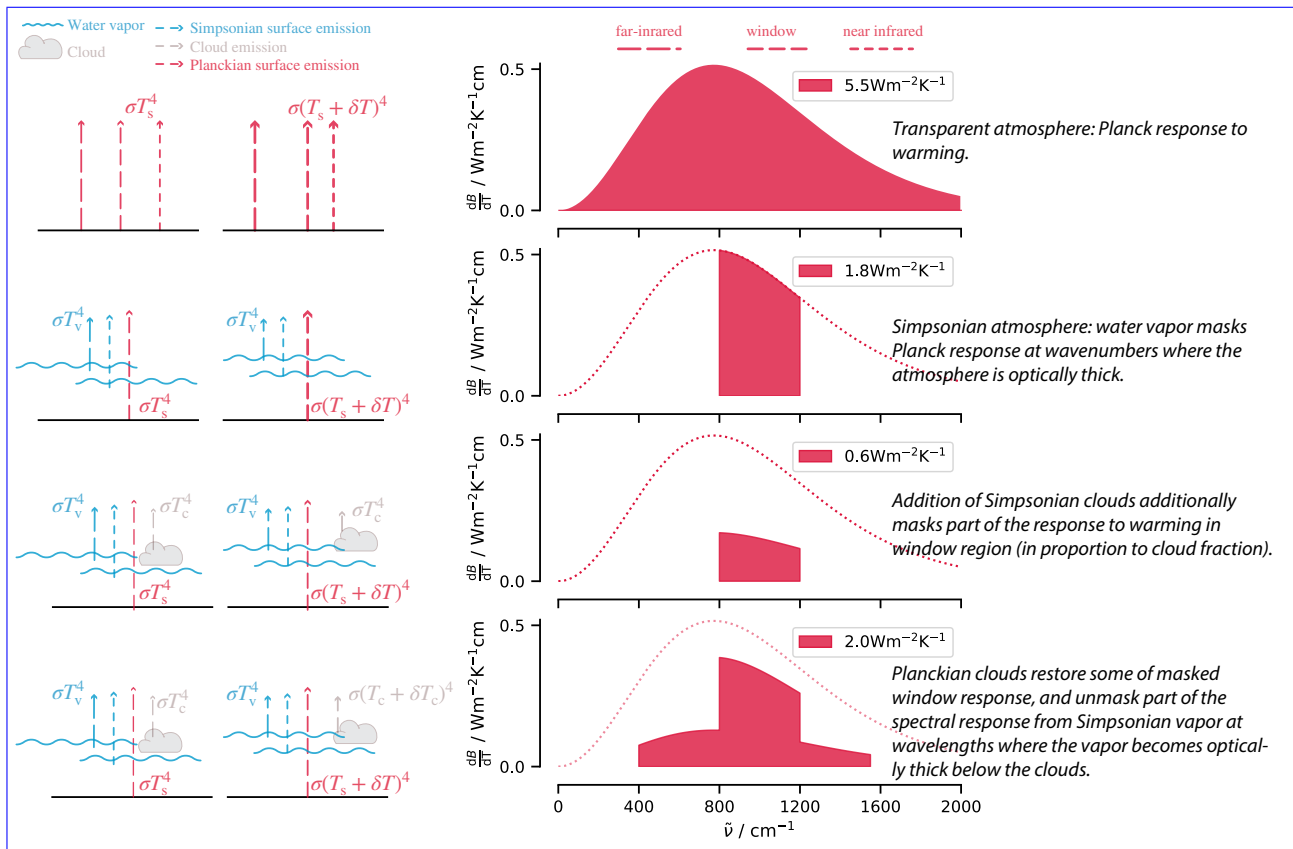
Figure 1. Conceptual framework showing how Simpsonian clouds and water vapor mask the radiative response at wavenumbers where they control the emission to space, and how part of the spectral response is restored from Planckian clouds.
