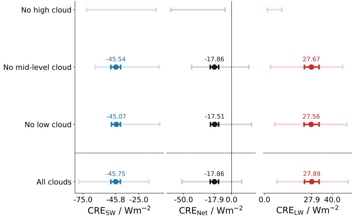
Figure 3. Distribution of the shortwave cloud-radiative effect \text{CRE}_{\text{SW}} , the net cloud-radiative effect \text{CRE}_{\text{Net}} , the longwave cloud-radiative effect \text{CRE}_{\text{LW}} . The faded lines depict the 5%–95% interval of all possible CRE values in the full ensemble. The bold lines show the same range, but for a plausible subsample that is in agreement with a \pm 5 \text{ Wm}^{-2} range around the mean values from the CERES satellite observations (given as tick labels on the x-axis). Different “rows” of the figure show results for different simulations, in which certain cloud layers were turned off (e.g. the first for describes a simulation with all but high clouds).
