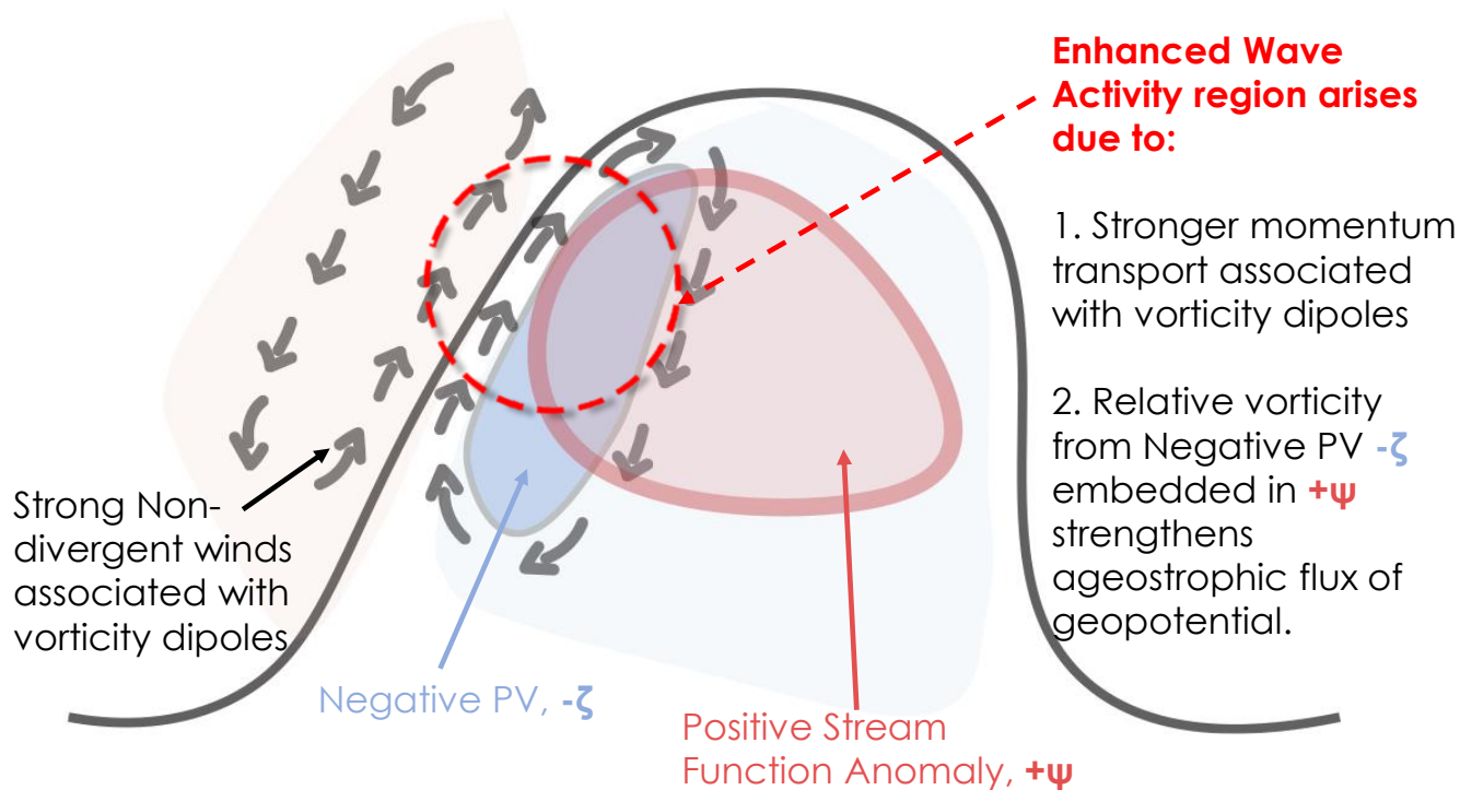
Figure 11. Schematic illustrating dry-dynamics mechanisms by which NPV interacts with the jet stream through the two-dimensional wave activity flux perspective. Features of importance are labeled. Other features not labeled include the black contour, representing the 2 PVU line, light blue shading represents a negative PV anomaly associated with the ridge, the light orange shading represents a positive PV anomaly associated with the trough.
