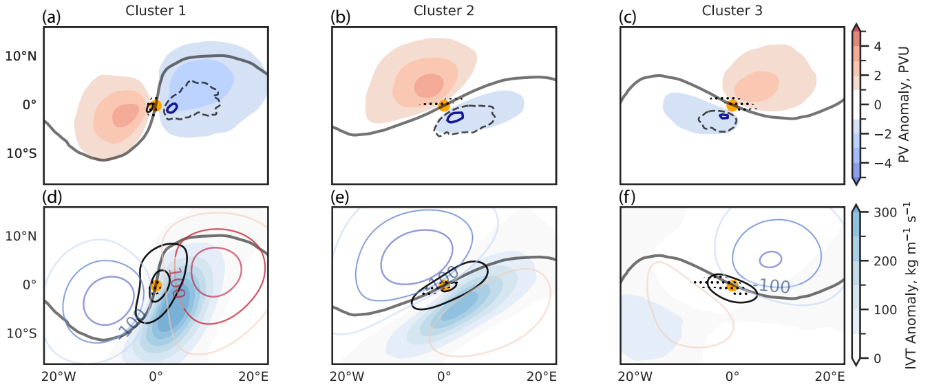
Figure 7. As in Figure 6 (first two rows) but for NPV-jet interactions using the 100-300 km threshold. Cluster 1 = 642 cases, Cluster 2 = 1969 cases, Cluster 3 = 1224 cases. Each NPV-jet (100-300 km) event is categorized into one of these clusters based on the event's similarity to the cluster centroids from Figure 6. A modification is made to the NPV frequency (dark blue contour) to show regions where synoptic-scale NPV is more frequent than 45% of the time. Stippling shows statistical significance at the 2% level using a student t-test. (a-c) shows statistically significant differences with respect to Figure 6 and where the PV gradient is greater than 1.25 PVU per 100 km. (d-f) shows statistically significant differences with respect to Figure 6 and where the wind speed differences are greater than 5 \text{ m s}^{-1} .
