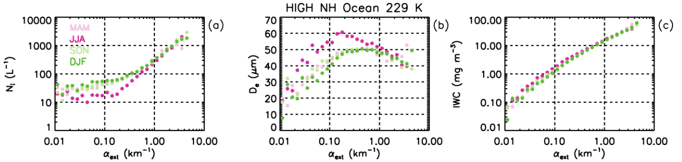
Figure 15. Seasonal analysis of the region 60-90° N over oceans for the 229 K temperature levels in terms of the extinction dependence of (a) N_i , (b) D_e , and (c) IWC. Extinction at maximum D_e , indicative of het-hom transition, is the smallest in JJA (dark pink) compared to MAM (light pink), SON (light green) and DJF (dark green), yielding the greatest hom fraction during JJA.
