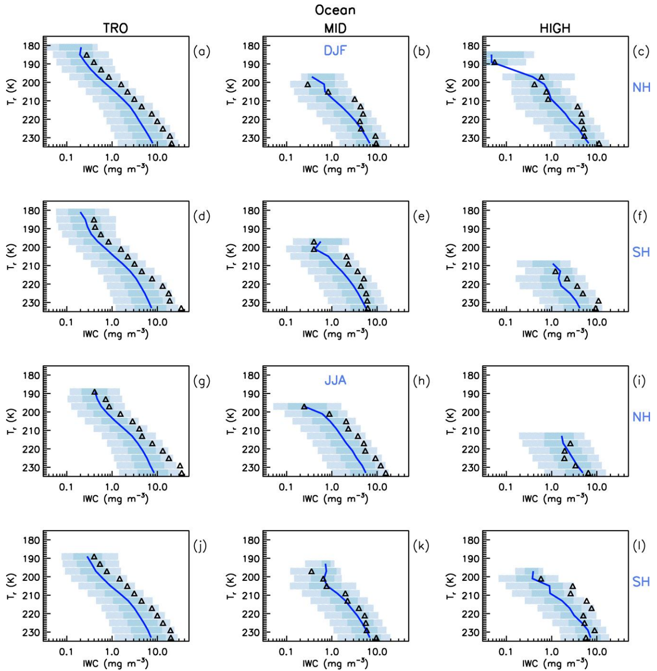
Figure 17. Comparing the median IWC (navy blue curves) over oceans (using all samples) with the temperature-dependent heterom transition point (black triangles) based on the D_e maximum and the corresponding extinction coefficient \alpha_{ext} for a given 4 K temperature interval. Latitude zones and seasons (DJF and JJA) are denoted as in Figs. 12 and 13. The light-blue shade lies between the 10 th and the 90 th percentiles and the overplotted medium-blue shade lies between the 25 th and 75 th percentiles.
