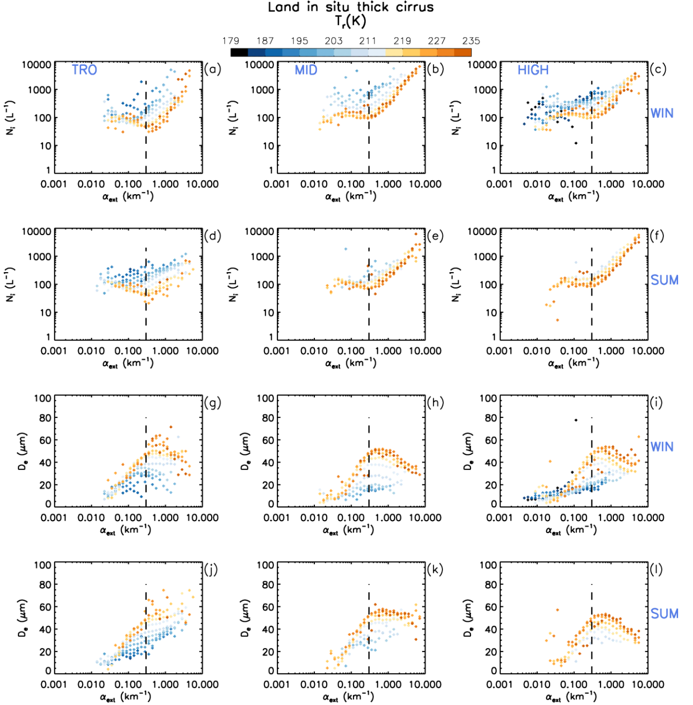
Figure 10. Same as in Fig. 9 but for retrievals over land for optically thick in situ cirrus ( \sim 0.3 < \tau < \sim 3 ).
