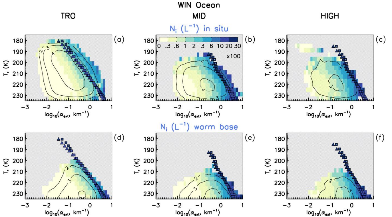
Figure 7. Median retrieved ice particle number concentration N_i plotted in T_r vs. \log(a_{ext}) space to separate the het- and hom-regimes. The black contours show the \log_{10} of the number of samples. The numbers in the color legend are to be multiplied by 100 to give N_i in L^{-1} . Retrievals are over ocean using all IIR samples for in situ cirrus and WBC as indicated, with \tau ranging from \sim 0.01 to \sim 3 , for the tropics (TRO, panels a and d), midlatitudes (MID, panels b and e), and high latitudes (HIGH, panels c and f) during winter (WIN) using both hemispheres during 2008, 2010, 2012 and 2013. The triangles and squares represent theoretical and empirical predictions for ice nucleation through hom. The color within each triangle or square indicates the approximate N_{max} for pure hom conditions via the color bar legends.
