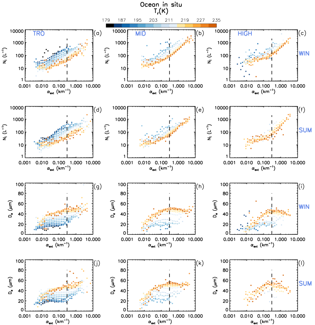
Figure 9. The dependence of median log N_i (upper half, panels a-f) and median D_e (lower half, panels g-l) on \alpha_{ext} for all in situ cirrus samples over oceans ( \sim 0.01 < \tau < \sim 3 ). The various T_r intervals (4 K/interval) are given by the color legend. Each row features the tropics (TRO), midlatitudes (MID), and high latitudes (HIGH) in both hemispheres for either winter (WIN) or summer (SUM). The vertical dashed line at \alpha_{ext} = 0.3 km -1 in panels a – f marks where a change in slope generally occurs for the 231–235 K interval. These same dashed line positions are also indicated in panels g – l showing their relation to the D_e maximum.
