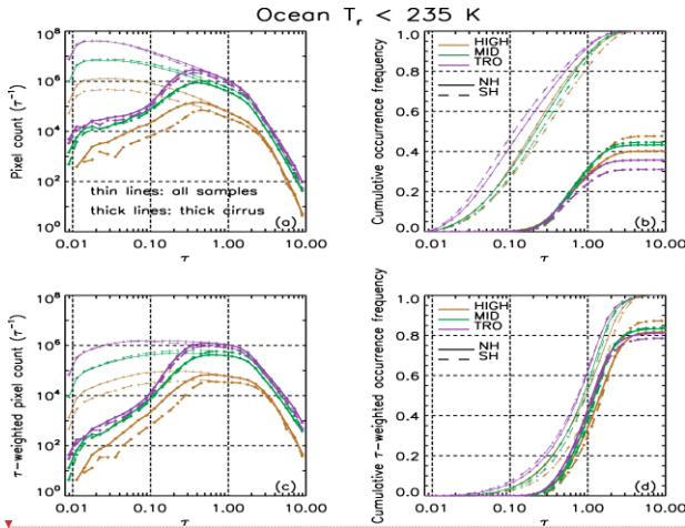
Figure 1. The upper panels (a and b) show IIR cirrus sampling statistics during 2008, 2010, 2012 and 2013 over visible optical depth ( \tau ) while the lower panels (c and d) show the same distribution of sampled pixels multiplied by \tau . All samples have a cloud radiative temperature T_r \leq 235 K for the tropics (purple), midlatitudes (green) and high latitudes (brown). Solid and dashed patterns refer to the northern and southern hemispheres, respectively. The product of the number of IIR pixels \times \tau is a proxy for the radiative impact of cirrus clouds. The thin curves indicate all IIR samples while the thicker curves are for the optically thick clouds. The right panels (b and d) show the cumulative distributions. The IIR pixels count is normalized per \tau bin-size. Retrievals are only over oceans to minimize uncertainties at the lowest \tau .
