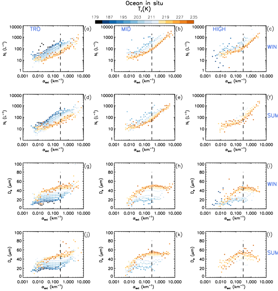
415 Figure 9. The dependence of median log N_i (upper half, panels a-f) and median D_e (lower half, panels g-l) on \alpha_{ext} for all in situ cirrus samples over oceans ( -0.01 < \tau < \sim 3 ). The various T_r intervals (4 K/interval) are given by the color legend. Each row features the tropics (TRO), midlatitudes (MID), and high latitudes (HIGH) in both hemispheres for either winter (WIN) or summer (SUM). The vertical dashed line at \alpha_{ext} = 0.3 km^{-1} in panels a – f marks where a change in slope generally occurs for the 231-235 K interval. These same dashed line positions are also indicated in panels g – l showing their relation to the D_e maximum.
