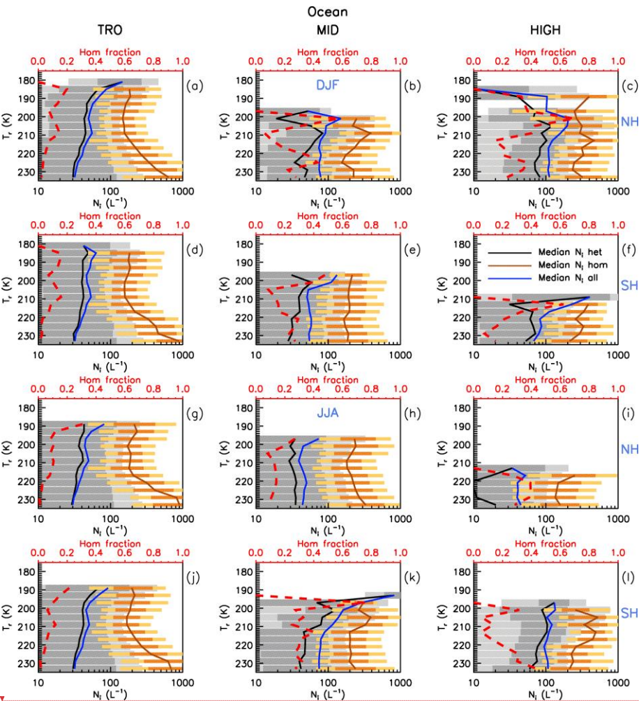
Figure 12. The T_r dependence of the hom fraction (red dashed) for all samples over oceans ( \sim 0.01 < \tau < 3 ). Each row features the tropics (TRO), midlatitudes (MID), and high latitudes (HIGH) for either the northern (NH) or southern (SH) hemisphere in DJF and JJA during 2008, 2010, 2012, and 2013. Also shown are median N_i profiles for all cirrus (blue), for het cirrus (black), and for hom cirrus (orange). The 25 to 75 percentile range is indicated by darker grey shading for het cirrus and darker orange shading for hom cirrus, while the 10 to 90 percentile range is indicated by lighter grey shading for het cirrus and lighter orange shading for hom cirrus.
