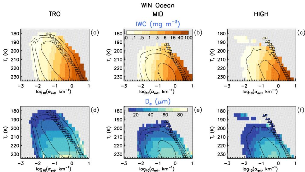
Figure 8. Median retrieved IWC (panels a–c) and D e (panels d–f) plotted in T r vs. log(α ext ) space to separate the het- and hom-regimes. The black contours show log 10 (number of samples). The color-bars give IWC (mg m -3 ) and D e (μm). Retrievals are over oceans using all IIR samples (both in situ and WBC), with τ ranging from ~0.01 to ~3, for the tropics (TRO, panels a, d), midlatitudes (MID, panels b, e), and high latitudes (HIGH, panels c, f) during winter (WIN) using both hemispheres during 2008, 2010, 2012 and 2013. The triangles and the squares represent predictions from simple hom theory using Eq. (4) and Schneider et al. (2021), respectively, and the color within each triangle or square indicates the approximate IWC hom (panels a–c) and hom D e (panels d–f) values via the color bar legends.
