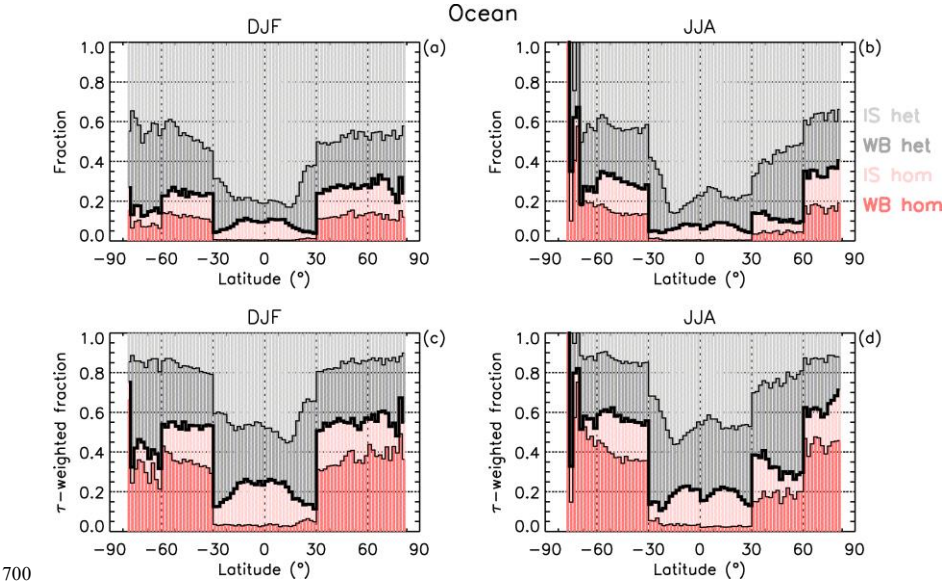
Figure 16. Upper panels (a and b): the fraction of warm base (WB) (red) and in situ (pink) hom affected cirrus and of WB (dark grey) and in situ (light grey) het cirrus vs. latitude (negative in SH) in (a) DJF and (b) JJA based on all samples over oceans. The thick black histogram gives the total fraction of hom affected cirrus. Lower panels (c and d): same as upper panels except that the fractions are weighted by cloud optical depth ( \tau ).
