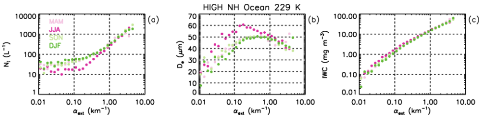
Figure 15. Seasonal analysis of the region 60-90° N over oceans for the 229 K temperature levels in terms of the extinction dependence of (a) N_i , (b) D_e , and (c) IWC. Extinction at maximum D_e , indicative of het-hom transition, is the smallest in JJA (dark pink) compared to MAM (light pink), SON (light green) and DJF (dark green), yielding the greatest hom fraction during JJA.
