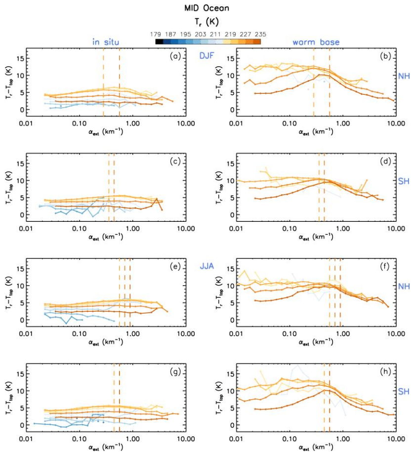
760 Figure 18. Dependence of T_r - T_{top} (which is related to cirrus cloud geometrical thickness) on the extinction coefficient \alpha_{ext} for various 4 K temperature bins indicated by the color bar. Retrievals were over oceans ( \sim 0.01 < \tau < \sim 3 ) for in situ cirrus (panels a, c, e, g) and WBC (panels b, d, f, h) clouds at mid-latitude for two seasons (DJF & JJA) in both hemispheres (NH & SH) during 2008, 2010, 2012, and 2013. Vertical lines indicate D_c maxima for the three “warmest” temperature bins, revealing a correspondence between cloud thickness and D_c maxima. Panels having only two vertical lines result from two D_c maxima having the same \alpha_{ext} .
