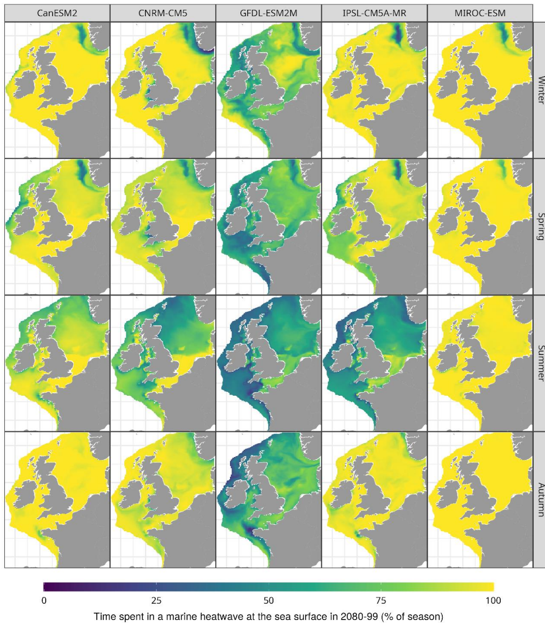
205 Figure 4: Projected average rate of heatwave occurrence at the sea surface for each season in 2080-2099 using five dynamically downscaled climate models and climate change scenario RCP 8.5. Each column shows the projection from one model.
