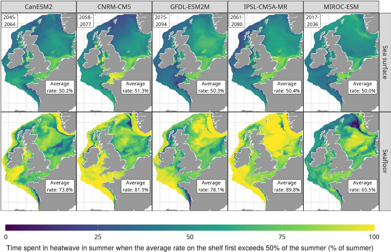
Figure 5: Marine heatwaves at the sea surface and seafloor in the first 20-year period when, on average across the shelf, heatwaves occur more than 50% of the summer at the surface. The 20-year period shown in the top-left of each panel indicates when the 50% threshold is first exceeded. In the bottom-right of each plot, the average fraction of time the shelf is in a heatwave at the surface or seafloor is shown. For example, CanESM2 projects that in 2045-2064, surface heatwaves will occur on average 50.2% of the summer, but seafloor heatwaves will occur 73.8% of the summer.
