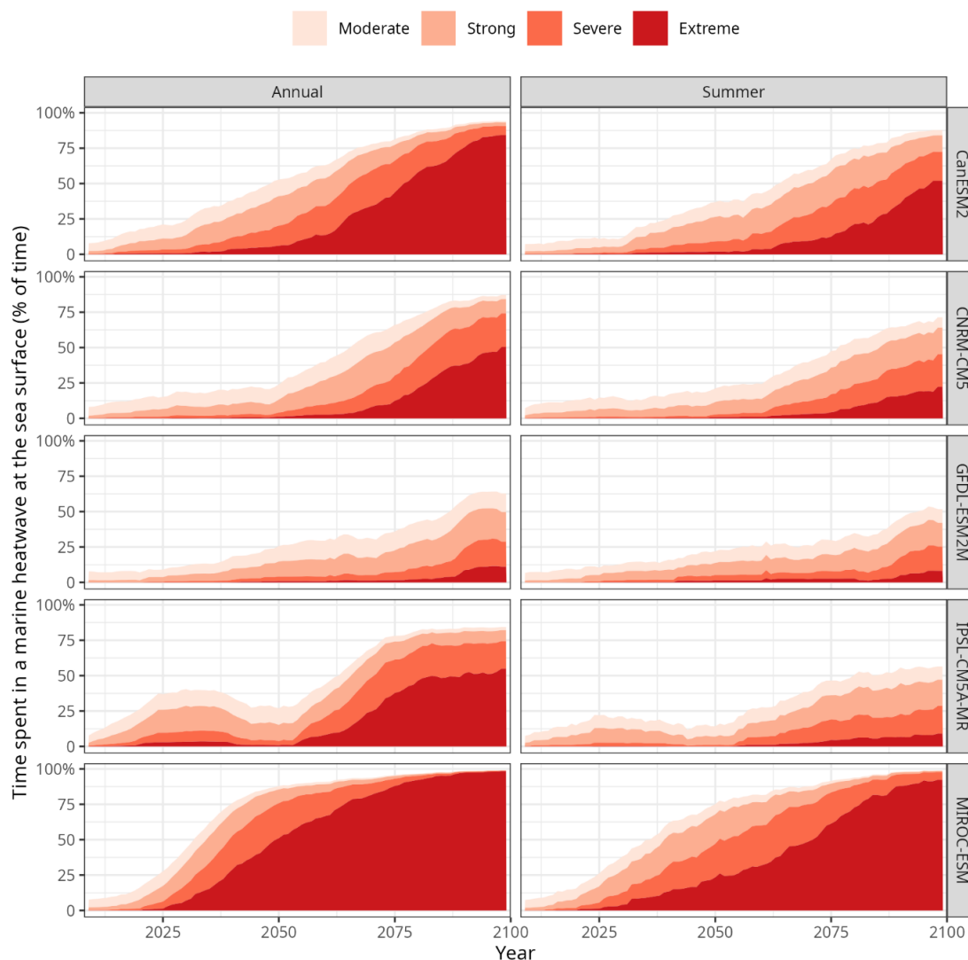
Figure 7: Projected average rate of marine heatwave occurrence by category at the sea surface, averaged across the northwest European Shelf, using five dynamically downscaled climate models under RCP 8.5. Heatwaves are stacked by colour, i.e., the total frequency of heatwaves is shown by the top line. The left column shows the average frequency of heatwaves each year, and the right column shows the frequency during summer. A 20-year rolling average is shown, with the output aligned to the final year in each 20-year period.
