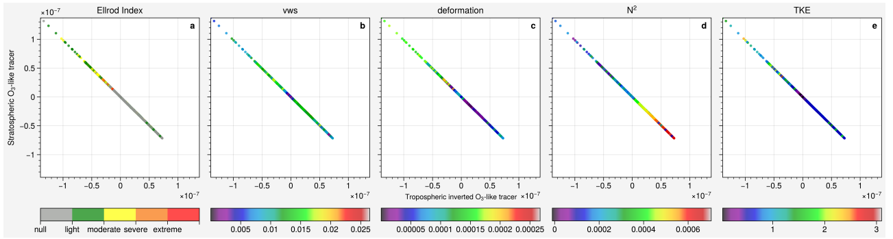
Figure 11. Case 2: Delta tracer-tracer correlation of stratospheric O 3 -like/Inverted tropospheric O 3 -like tracers ( \text{kg}^{-1} \text{kg}^{-1} ) color-coded with (a) Ellrod Index ( \text{s}^{-2} ), (b) vertical wind shear ( \text{s}^{-1} ), (c) deformation ( \text{s}^{-1} ), (d) Brunt-Väisälä frequency ( \text{s}^{-2} ) and (e) turbulence kinetic energy ( \text{m}^2 \text{s}^{-2} ) at 2016-02-05 05:00.
