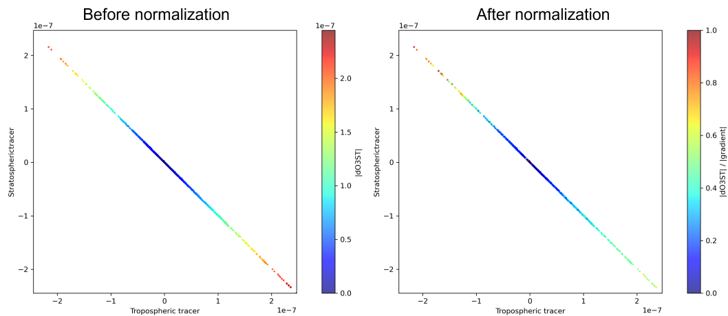
Figure 10. Delta tracer-tracer correlation color-coded with |\Delta O3ST| ( \text{kg}^{-1} \text{kg}^{-1} ; left) and |\Delta O3ST| / |\text{gradient}| (right)
