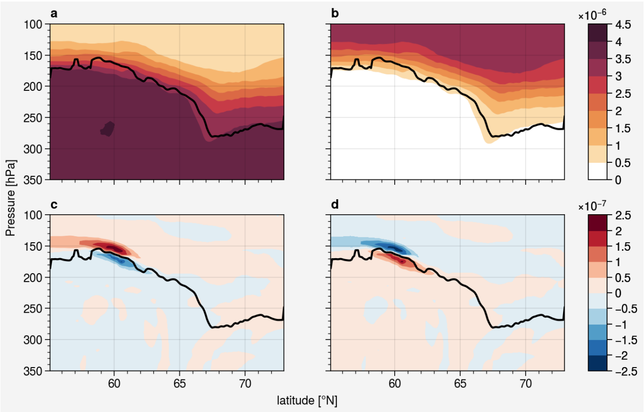
Figure 5. Cross section of distribution (a) Inverted O3-like tracers, (b) O3-like tracers; difference (vdiff on - off) (c) Inverted O3-like tracers, (d)O3-like tracers at 2016-02-05 18:00. The black line indicates the PV-tropopause.
