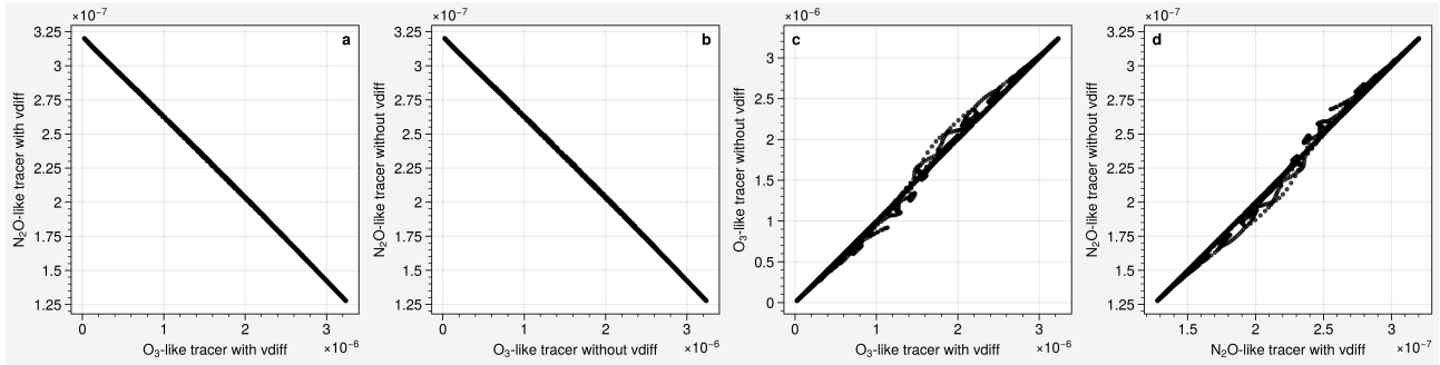
Figure 6. tracer-tracer correlation for (a) O 3 -like/N 2 O-like tracers with vdiff; (b) O 3 -like/N 2 O-like tracers without vdiff; (c) O 3 -like tracers with/without vdiff, (d) N 2 O-like tracers with/without vdiff at 2016-02-05 18:00.
