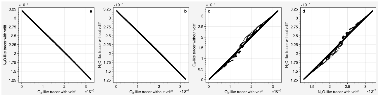
Figure 6. tracer-tracer correlation for (a) O3-like/N2O-like tracers with vdif; (b) O3-like/N2O-like tracers without vdif; (c) O3-like tracers with/without vdif, (d) N2O-like tracers with/without vdif at 2016-02-05 18:00.
