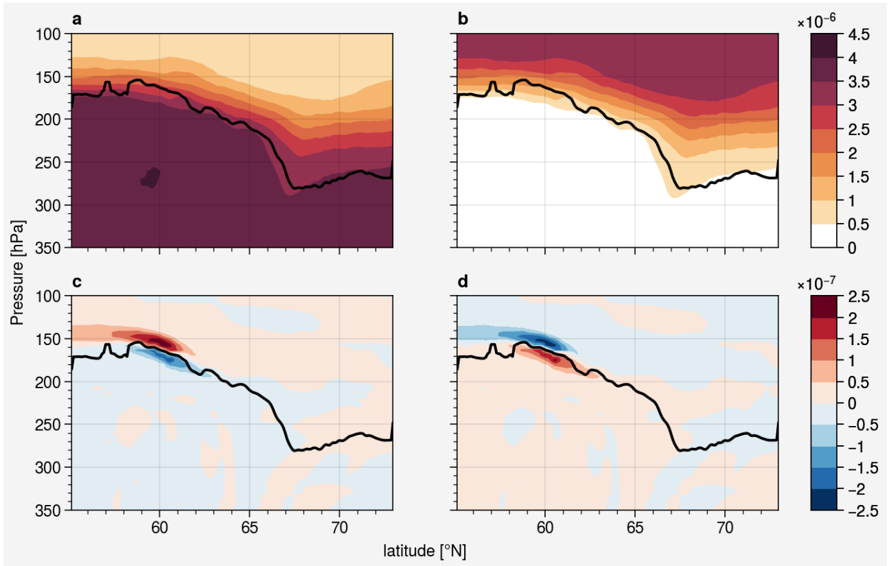
Figure 5. Cross section of distribution (a) Inverted O3-like tracers, (b) O3-like tracers; difference (vdif on - off) (c) Inverted O3-like tracers, (d) O3-like tracers at 2016-02-05 18:00. The black line indicates the PV-tropopause.
