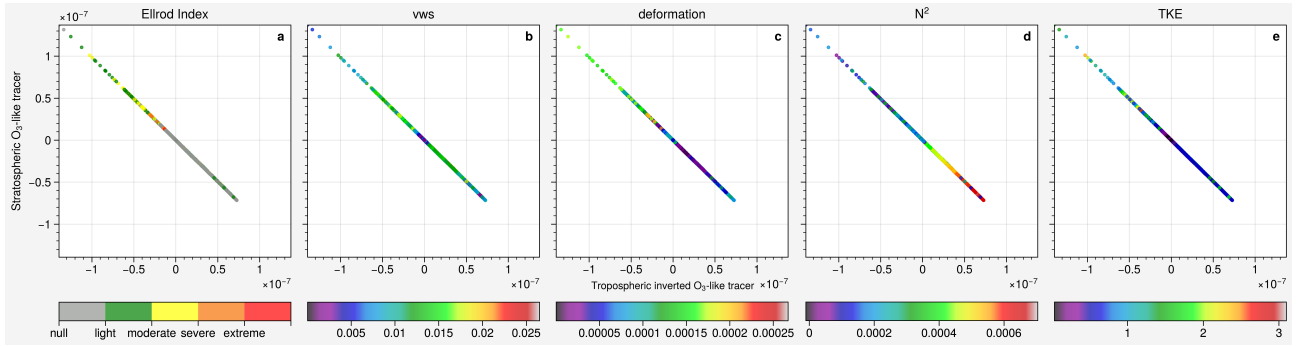
Figure 11. Case 2: Delta tracer-tracer correlation of stratospheric O 3 -like/Inverted tropospheric O 3 -like tracers ( kg^{-1} kg^{-1} ) color-coded with (a) Ellrod Index ( s^{-2} ), (b) vertical wind shear ( s^{-1} ), (c) deformation ( s^{-1} ), (d) Brunt-Väisälä frequency ( s^{-2} ) and (e) turbulence kinetic energy ( m^2 s^{-2} ) at 2016-02-05 05:00.
