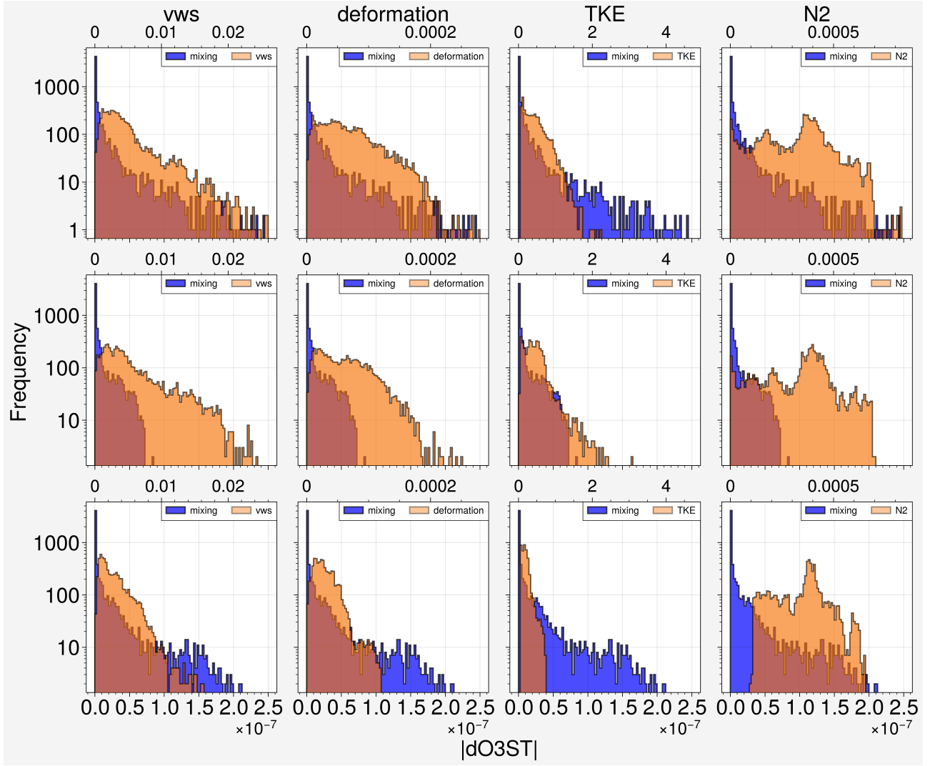
Figure 13. Frequency distribution of |\text{mixed } d\text{O3ST}|/(\text{kg}^{-1} \text{kg}^{-1}) of O3-like tracers, vertical wind shear, deformation, TKE and N2 for case 1 (top), case 2 (middle), case 3 (bottom)
