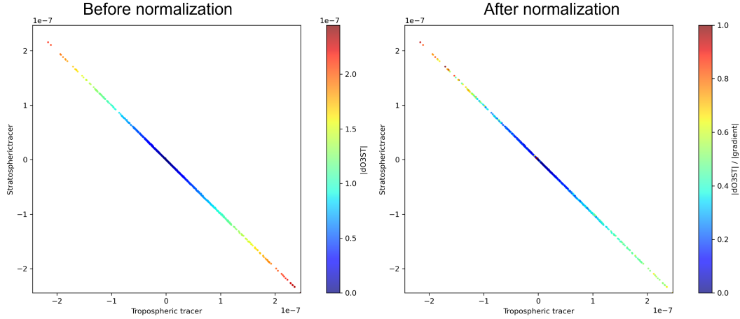
Figure 10. Delta tracer-tracer correlation color-coded with |mixing dO3ST| ( kg^{-1} kg^{-1} ; left) and |mixing dO3ST|/|gradient| (right)
