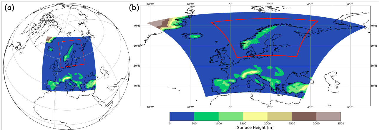
Figure 1. Model domain for MECO(n) with surface height: (a) an overview, (b) a close-up for CM40 and CM10.
