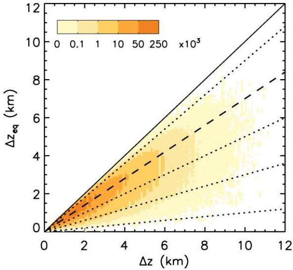
340 Figure 6. \Delta z_{\text{eq}} vs. \Delta z for all sampled cirrus over oceans during 2008, 2010, 2012, and 2013. The colors represent the IIR pixels density. The dashed and dotted lines, from bottom to top, represent \Delta z_{\text{eq}}/\Delta z of 0.1, 0.3, 0.5, 0.7, and 0.9.
