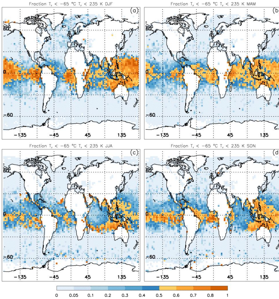
Figure 16. Seasonal maps of the fraction of cirrus cloud pixels ( T_r \leq 235 K) having T_r < -65^\circ\text{C} (208 K) over oceans only, where \sim 0.01 < \tau < \sim 3 . This is the fraction of cirrus clouds for which the ATTREX-POSIDON formulation is used in this retrieval. The four panels are for (a) December-January-February (DJF), (b) March-April-May (MAM), (c) June-July-August (JJA), and (d) September-October-November (SON) during 2008, 2010, 2012 and 2013.
