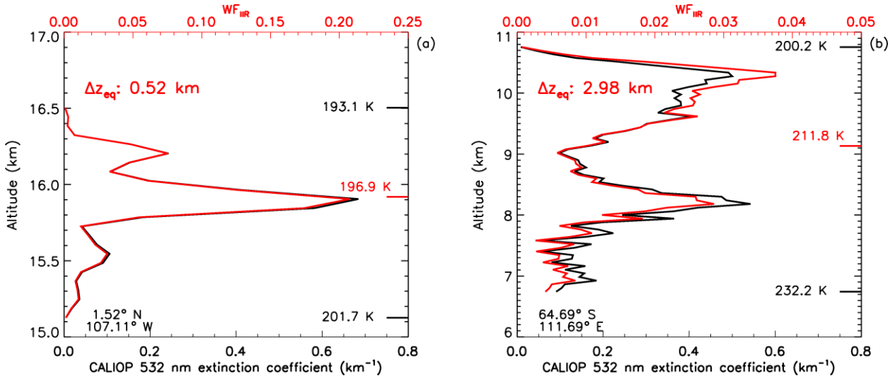
335 Figure 5. Two cirrus cloud examples showing the CALIOP extinction coefficient ( \alpha_{\text{part}} ) profile in black and the IIR weighting function ( WF_{\text{IIR}} ) profile in red, with \Delta z_{\text{eq}} indicated in red. The temperatures in black on the right-hand side of each panel are at cloud top and base, and in red is the radiative temperature ( T_r ) at the corresponding altitude. These examples are extracted from CALIPSO granules (a) 2010-06-04T08-39-58ZN and (b) 2008-08-12T07-26-54ZD, with latitude and longitude given in the lower left corner of the respective panels.
