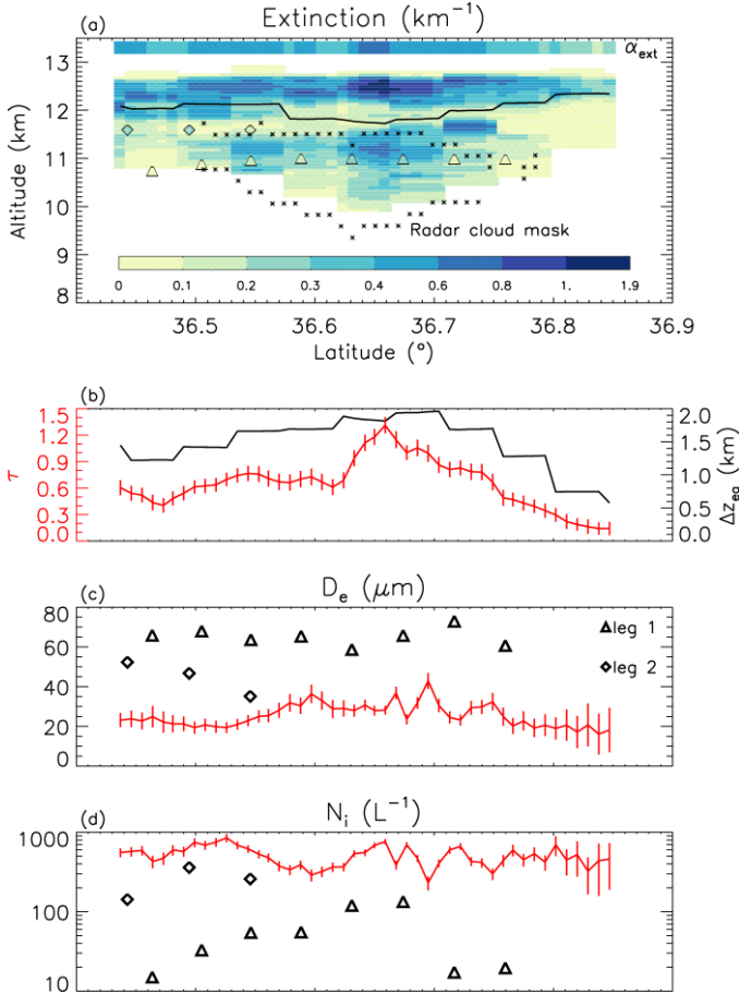
690 Figure 21. Comparison of IIR retrievals and in situ observations on 30 March 2010 during the SPARTICUS field campaign (CALIPSO granule 2010-03-30T19-27-25ZD). (a) extinction profile derived from the CALIOP lidar, IIR layer \alpha_{ext} , and PSD extinctions in leg 1 (triangles) and leg 2 (diamonds). The solid black line in panel a is the radiative altitude corresponding to \tau_r . The stars denote the boundaries of the CloudSat radar GEOPROF cloud mask, and the color bar at the bottom gives \alpha_{ext} values; (b) IIR \tau (red) and \Delta z_{eq} (black, right axis); (c) IIR (red) and in situ (triangles and diamonds) D_e ; (d) same as (c) but for N_i . The vertical bars in red in panels b-d represent the IIR estimated uncertainties.
