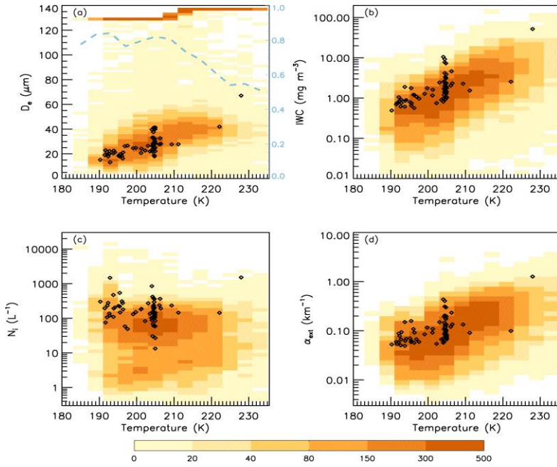
Figure 18. Pixel sampling densities (given by the color bar) for retrievals of (a) D_e , (b) IWC, (c) N_i , and (d) a_{ext} taken during the period of the ATTREX field campaign (February–March 2014) over the ATTREX domain ( 0^\circ \text{ N} - 20^\circ \text{ N} and 130^\circ \text{ E} - 160^\circ \text{ E} ) where \sim 0.01 < \tau < 3 . Black diamonds indicate corresponding aircraft PSD measurements of these properties. The right vertical axis of the D_e plot indicates the fraction of cirrus clouds sampled having \beta_{eff} greater than the \beta_{eff} sensitivity limit given by the blue-dashed curve while the high sample densities having D_e between 130 \mu\text{m} and 136 \mu\text{m} are from samples having \beta_{eff} lower than the \beta_{eff} sensitivity limit (i.e., non-quantifiable D_e ). The change in D_e from 130 to 136 is due to the temperature interpolation (ATPO to TC4).
