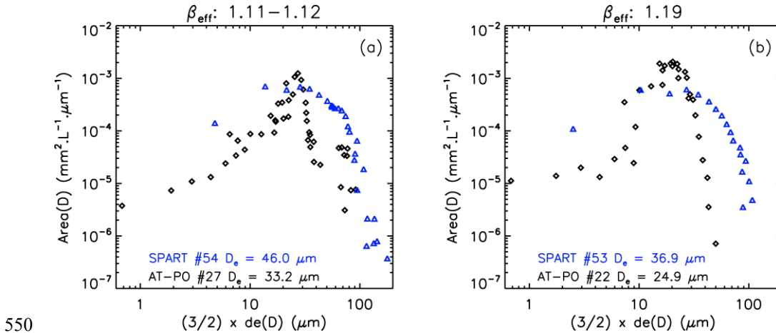
Figure 15. Comparisons of area PSDs from the ATTREX-POSIDON (black) and SPARTICUS (blue) campaigns having very similar \beta_{\text{eff}} values but considerably different D_e values, illustrating how differences in PSD shape between the two field campaigns can yield different D_e - \beta_{\text{eff}} relationships.
