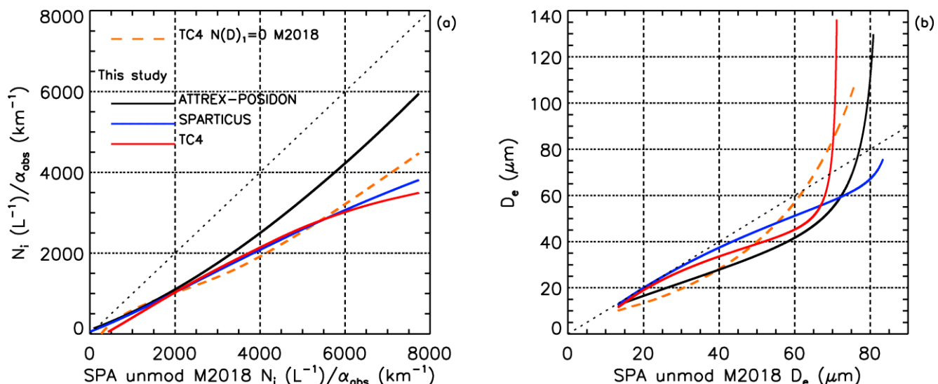
600 Figure 17. Comparison of (a) N_i and (b) D_e retrievals in this study (black: ATTREX-POSIDON, navy blue: SPARTICUS, red: TC4) and from TC4 N(D)_1 = 0 in M2018 (dashed orange) with retrievals from SPARTICUS N(D)_1 unmodified in M2018.
