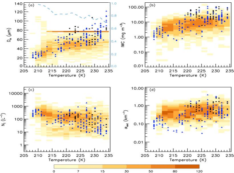
Figure 20. Pixel sampling densities (given by the color bar) for retrievals of (a) D_e , (b) IWC, (c) N_i , and (d) \alpha_{\text{ext}} taken during the period of the SPARTICUS field campaign (January through April 2010) over the SPARTICUS domain (31- 42 °N; 90-103 °W) where \sim 0.3 < \tau < \sim 3 . Black diamonds indicate corresponding aircraft PSD measurements of these properties. The right vertical axis of the D_e plot indicates the fraction of cirrus clouds sampled having \beta_{\text{eff}} greater than the \beta_{\text{eff}} sensitivity limit given by the blue-dashed curve while the high sample densities having D_e \sim 78 \mu\text{m} are from samples having \beta_{\text{eff}} lower than the \beta_{\text{eff}} sensitivity limit (i.e., non-quantifiable D_e ).
