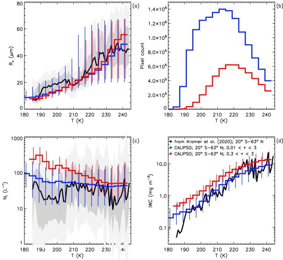
735 Figure 22. Temperature dependence of median values of (a) R_v ( \mu\text{m} ), (c) N_i ( \text{L}^{-1} ), and (d) IWC ( \text{mg m}^{-3} ) from the IIR retrievals (red: \sim 0.3 < \tau < 3 ; blue: \sim 0.01 < \tau < 3 ) and from the Krämer et al. (2020) in situ climatology (black curves). The vertical bars indicate the IIR 25 th and 75 th percentiles, except in panel (b) which shows the number of IIR sampled pixels. The light shade of grey in panels (a) and (c) is between the 10 th and 90 th percentiles and the superimposed darker shade of grey is between the 25 th and 75 th percentiles for the in situ data.
