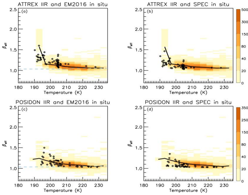
Figure 11. IIR \beta_{\text{eff}} vs. temperature in 0^\circ \text{N} - 20^\circ \text{N} and 130^\circ \text{E} - 160^\circ \text{E} during February and March 2014 (ATTREX, panels a and b) and October 2016 (POSIDON, panels c and d) compared with \beta_{\text{eff}} of PSDs (diamonds) measured during the denoted campaigns using the EM2016 (panels a and c) and the SPEC (panels b and d) mass-dimension relationships. The colors indicate IIR samples density and black curves represent median IIR \beta_{\text{eff}} . The horizontal dashed light blue lines in panels a and c indicate \beta_{\text{eff}} at the sensitivity limit (see Sect. 3). IIR optical depth > \sim 0.3 .
