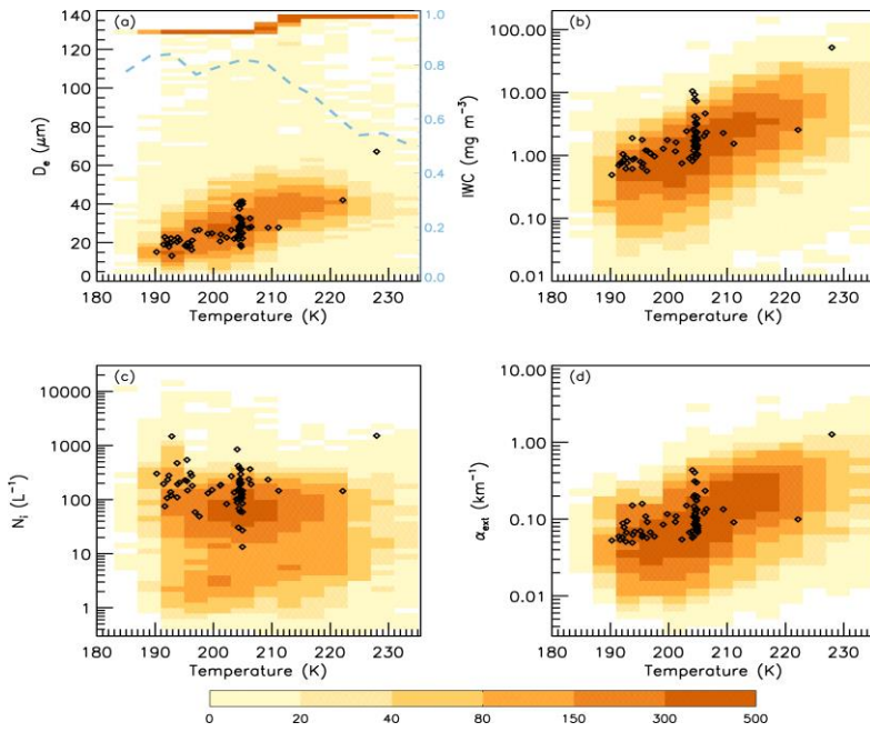
Figure 18. Pixel sampling densities (given by the color bar) for retrievals of (a) D_e , (b) IWC , (c) N_i , and (d) a_{ext} taken during the period of the ATTREX field campaign (February-March 2014) over the ATTREX domain ( 0^\circ N - 20^\circ N and 130^\circ E - 160^\circ E) where \sim 0.01 < \tau < 3 . Black diamonds indicate corresponding aircraft PSD measurements of these properties. The right vertical axis of the D_e plot indicates the fraction of cirrus clouds sampled having \beta_{eff} greater than the \beta_{eff} sensitivity limit given by the blue-dashed curve while the high sample densities having D_e between 130 \mu\text{m} and 136 \mu\text{m} are from samples having \beta_{eff} lower than the \beta_{eff} sensitivity limit (i.e., non-quantifiable D_e ). The change in D_e from 130 to 136 is due to the temperature interpolation (ATPO to TC4).
