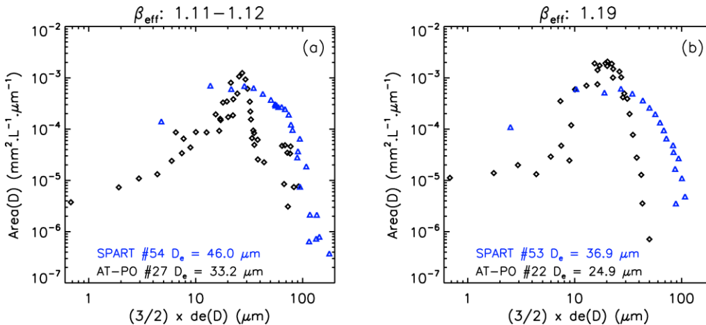
Figure 15. Comparisons of area PSDs from the ATTREX-POSIDON (black) and SPARTICUS (blue) campaigns having very similar \beta_{\text{eff}} values but considerably different D_e values, illustrating how differences in PSD shape between the two field campaigns can yield 545 different D_e - \beta_{\text{eff}} relationships.
