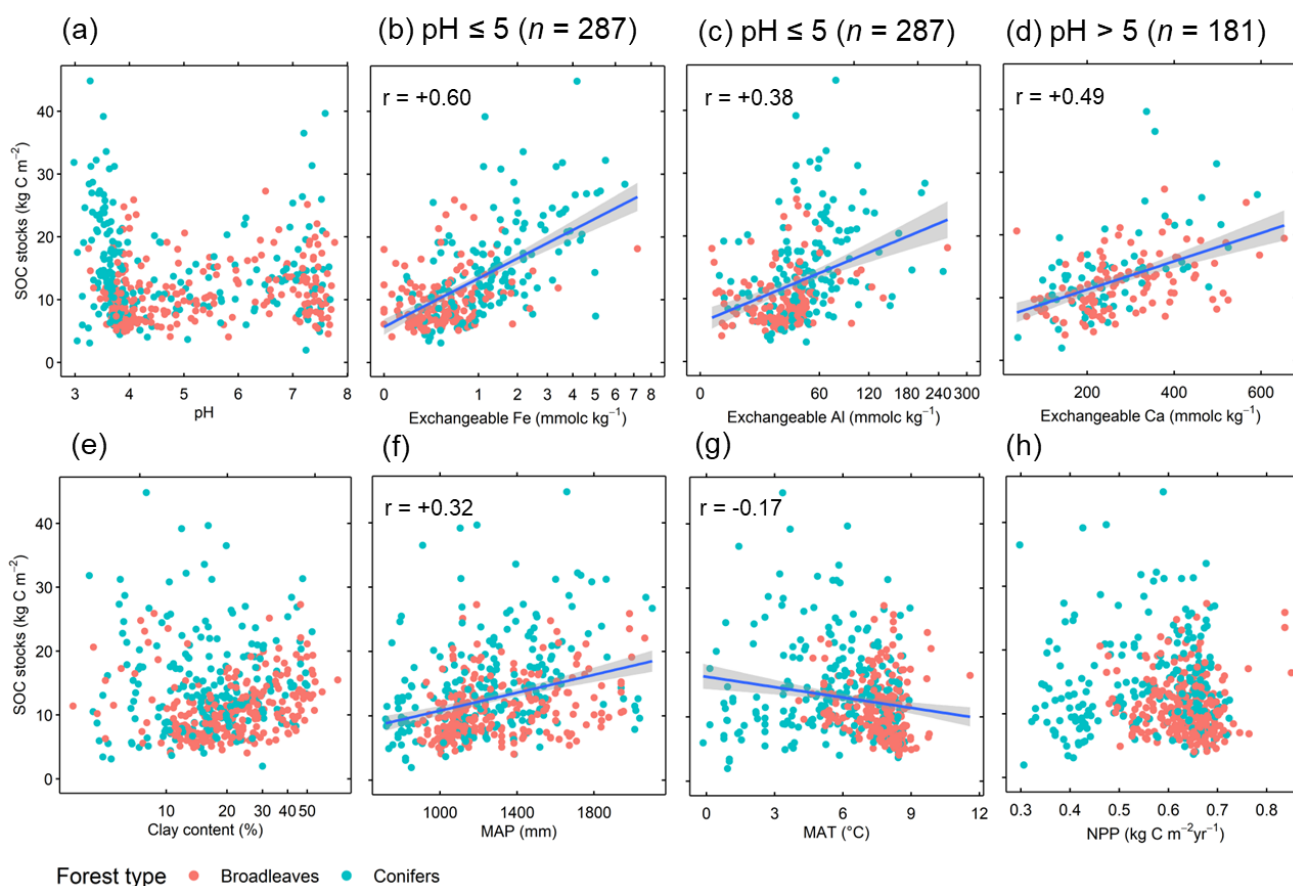
260 Figure 4: Correlations between total SOC stocks and selected soil properties (exchangeable Fe and Al are shown on a square-root scale axis, clay on a natural-logarithm scale axis) and site variables (MAP = mean annual precipitation; MAT = mean annual temperature; NPP = net primary production). Total n sites = 468 (waterlogged soils excluded). Plotted lines show significant linear correlations ( P < 0.05 ) with 95% confidence intervals in grey and the Pearson correlation coefficient ( r ).
