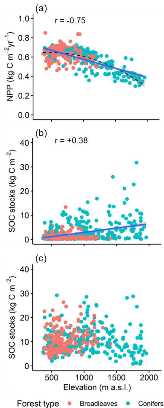
225 Figure 2: Net primary production (NPP) from MODIS (average 2001-2022) (a), SOC stocks in the organic layers (b), and in the mineral soil at 0-100 cm depth (c) against elevation in 468 forest sites across Switzerland (excluding waterlogged soils). Plotted lines show significant linear correlations ( P < 0.05 ) with 95% confidence intervals in grey and the Pearson correlation coefficient ( r ). A polynomial regression is also shown as dotted line in (a).
