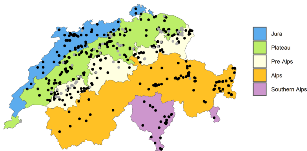
Figure 1: Distribution of the sampled forest sites (total n sites = 556, of which n = 88 waterlogged soils shown in grey) in the five biogeographic regions of Switzerland. Note that the Alps have fewer sites since largely un-forested (i.e. above the treeline).
