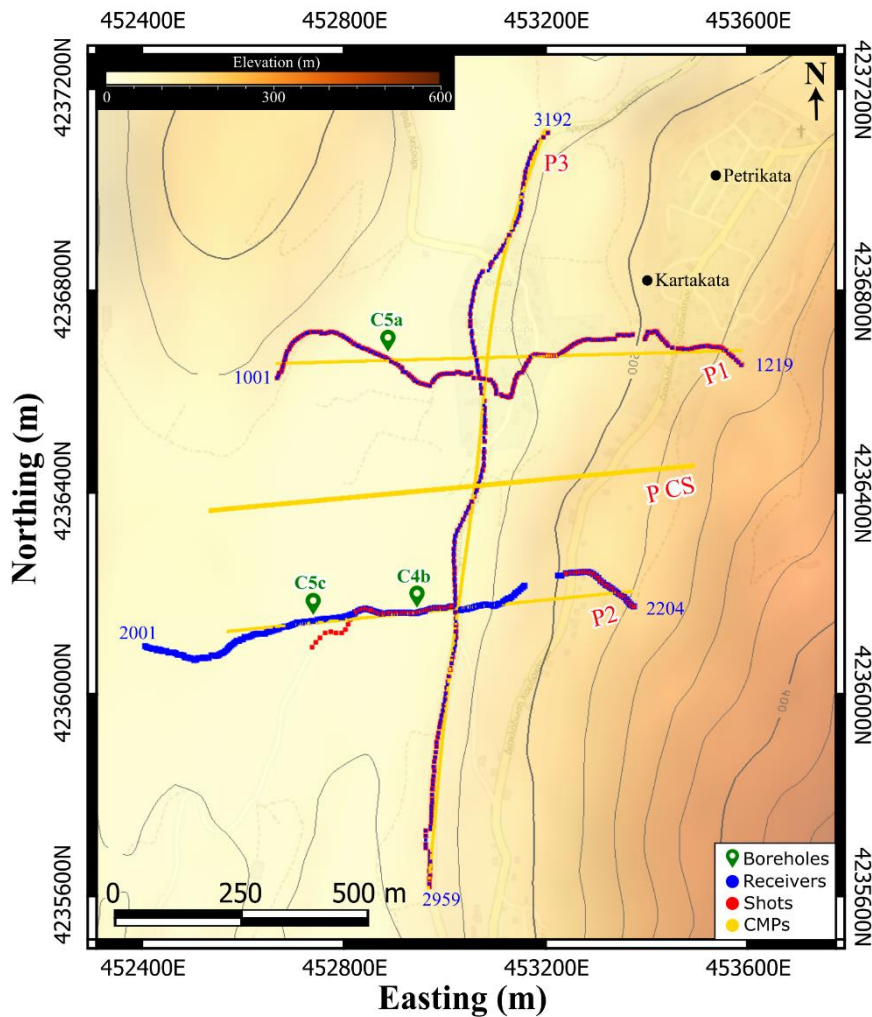
130 Figure 2: Seismic profiles 1 (P1), 2 (P2), 3 (P3), and CS (P CS) shown with the surface topography. Red dots correspond to source positions, blue dots correspond to receiver positions and yellow dots correspond to CMP positions used for data processing. Green pins correspond to boreholes C4b, C5a and C5c. Contour lines on the surface topography are 40 m apart.
