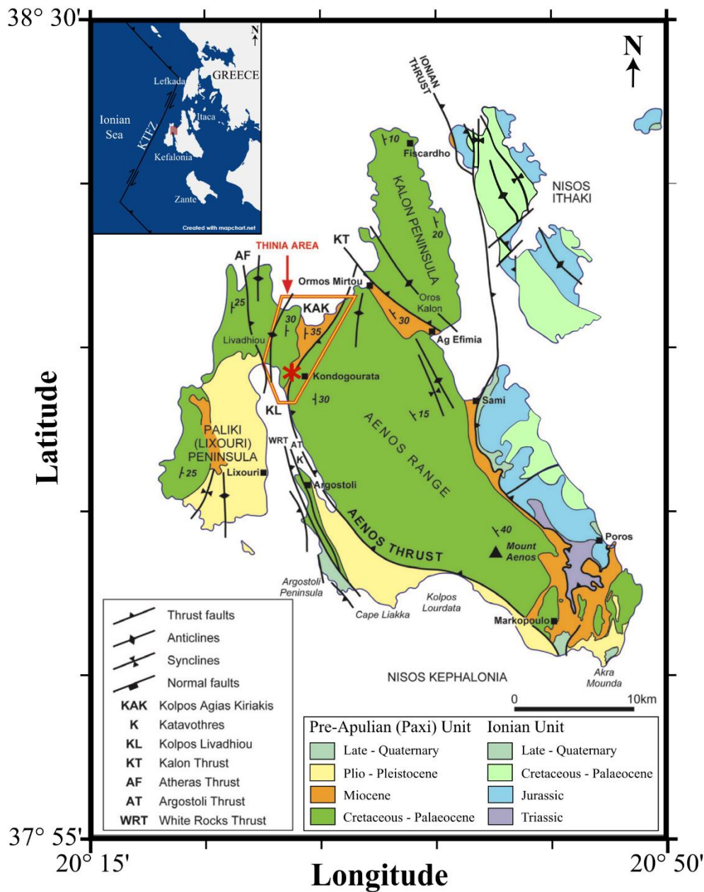
Figure 1: Geological map showing the main tectonic features of Kefalonia island and the location of the three-profile survey , (in red asterisk ) within the marked polygon (adapted from Underhill, 2006).
