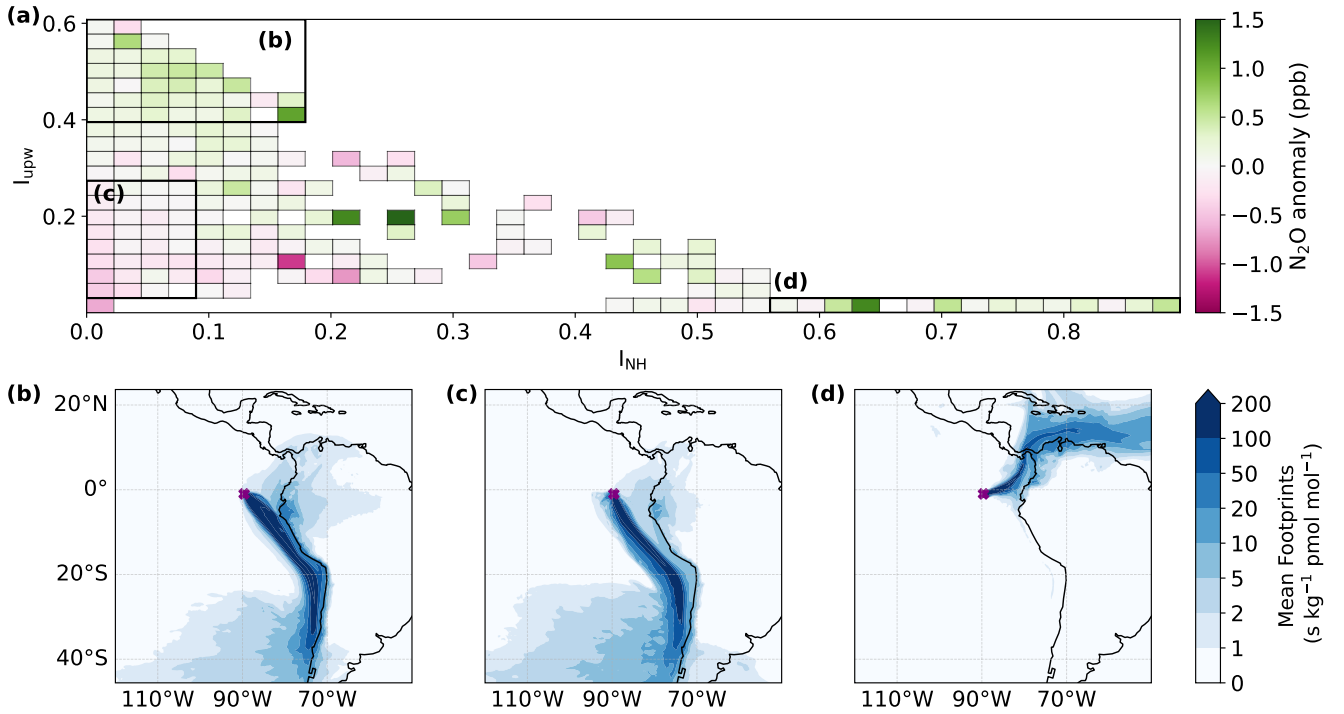
Figure 8. Attribution of observed nitrous oxide ( \text{N}_2\text{O} ) enhancements to air mass source regions, specifically the Peruvian and Chilean upwelling systems and the northern hemisphere. Panel (a) shows the mean anomaly of \text{N}_2\text{O} mole fractions relative to a 7-day mean, binned by varying levels of influence from upwelling systems ( I_{upw} ) and the northern hemisphere ( I_{NH} ). Definitions of the upwelling systems and northern hemisphere regions are provided in Fig. 2, and regional influences are calculated using Equation 3. Mean footprint maps are shown under varying influences: (b) high upwelling, low northern hemisphere; (c) low upwelling, low northern hemisphere; (d) low upwelling, high northern hemisphere. Panel (a) shows bin locations corresponding to Panels (b) – (d).
