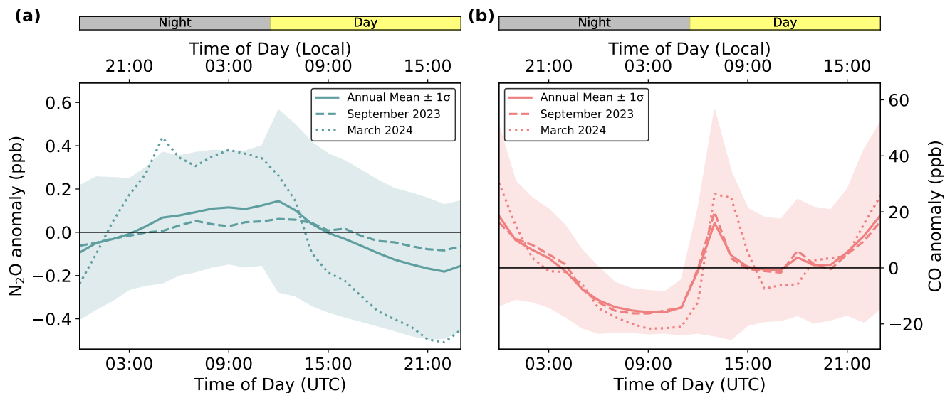
Figure 4. Observed diurnal cycle in (a) nitrous oxide (N 2 O) and (b) carbon monoxide (CO) at GEMSGAL . The diurnal cycle is represented as the hourly anomaly from the daily mean mole fractions. Shading signifies one standard deviation range for the overall mean. The solid black line represents zero anomaly. The time is reported in UTC to match the time zone used for reporting the mole fraction observation. The local time in the Galapagos is GMT-6. The color bar above each panel indicates daytime in yellow and nighttime in gray. No significant variation in day length is observed in the Galapagos due to its proximity to the equator.
