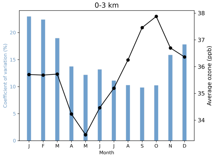
300 Figure 1: Evaluation of regional coefficient of variation (CV) and average of monthly mean ozone in the lowermost troposphere in 2017 over the Tropical Atlantic (25° S–25° N, 34° W–18° W). Light blue bar and black line indicate the coefficient of variation (CV) and average calculated from three products (IASI+GOME2, TCR-2 and CAMS reanalysis), respectively.
