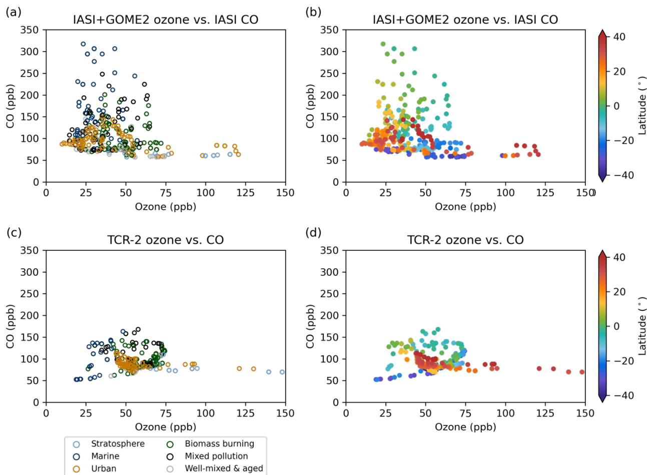
Figure 10: Scatter plots of CO vs. ozone for air masses sampled by ATom-2 derived from (a and b) satellite measurements of IASI and IASI+GOME2 and (c and d) TCR-2, respectively. Colours indicate (a and c) the air masses classification into six categories and (b and d) the latitude location.
