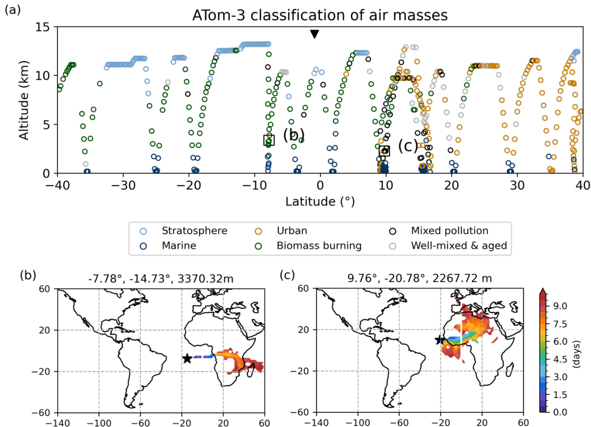
425 Figure 8: Classification and origin of air masses along the transect sampled by ATom-3. (a) Air masses are classified into six categories: marine (navy), stratosphere (light blue), urban (light brown), biomass burning (dark green), mixed pollution (black), and well-mixed and aged air (grey). Black inverted triangle indicates the well mixed and aged air influenced by lightning emissions. (b–c) Colours indicate average time since trajectories are initialized with NCEP winds.
