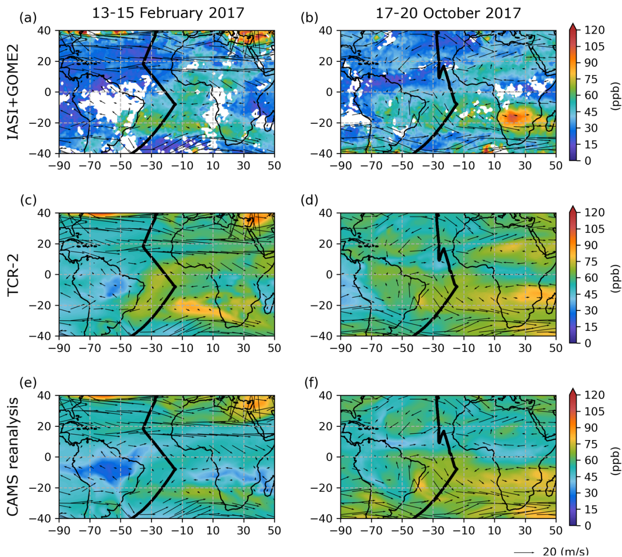
Figure 6: Distribution of mean ozone from 6 km to 9 km during 13–15 February and 17–20 October 2017. Black bold lines indicate the ATom-2 and ATom-3 flight tracks in (a–b) IASI+GOME2, (c–d) TCR-2 and (e–f) CAMS reanalysis. Winds at 9 km altitude from ERA5 are indicated by black arrows.
