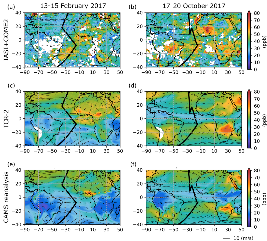
Figure 5: Distribution of mean ozone from surface to 3 km, during 13–15 February and 17–20 October 2017. Black bold lines indicate the ATom-2 and ATom-3 flight tracks in (a–b) IASI+GOME2, (c–d) TCR-2 and (e–f) CAMS reanalysis. Winds at 3 km altitude from ERA5 are indicated by black arrows.
