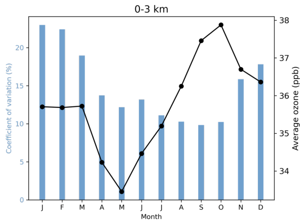
575 Figure 1: Evaluation of regional coefficient of variation (CV) and average of monthly mean ozone in the lowermost troposphere in 2017 over the Tropical Atlantic (25° S–25° N, 34° W–18° W). Light blue bar and black line indicate the coefficient of variation (CV) and average calculated from three products (IASI+GOME2, TCR-2 and CAMS reanalysis), respectively.
