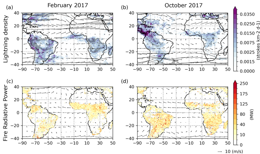
580 Figure 2: Monthly WGLC lightning density and fire radiative power (FRP) of presumed vegetation fire in (a and c) February and (b and d) October 2017. Winds at 3 and 10 km of altitude from ERA5 are indicated by black arrows in February and October, respectively. Black dots (a–b) indicate areas with OLR < 220 \text{ W m}^{-2} .
