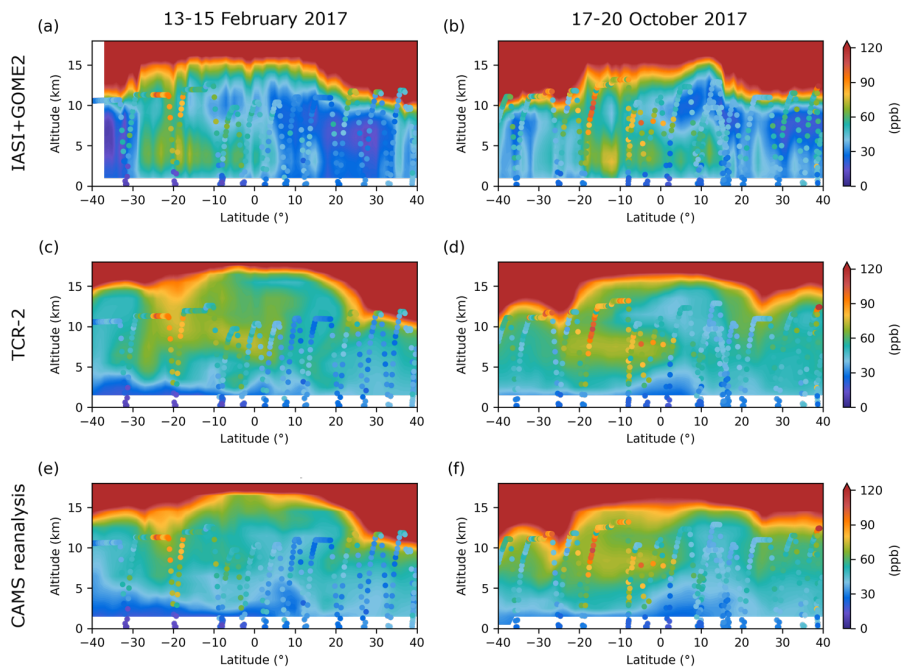
Figure 11: The ozone concentrations of (a–b) IASI+GOME2, (c–d) TCR-2 and (e–f) CAMS reanalysis are averaged for the period from 13 to 15 February 2017 and from 17 to 20 2017, respectively, and are extracted along the ATom flight tracks. Vertical profiles of ozone concentrations for the periods from 13 to 15 February and from 17 to 20 October 2017. Dots indicate ATom-2 and ATom-3 observations.
