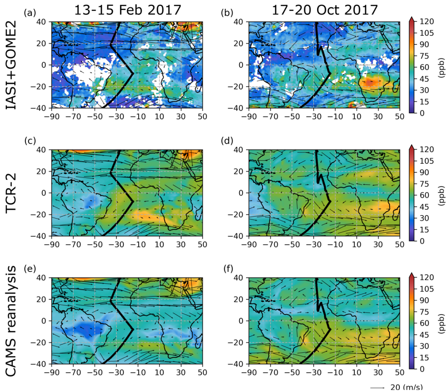
Figure 5: Distribution of mean ozone from 6 km to 9 km during 13–15 February and 17–20 October 2017. Black bold lines in (a–b) IASI+GOME2, (c–d) TCR-2 and (e–f) CAMS reanalysis indicate the ATom-2 and ATom-3 flight tracks. Winds at 9 km altitude from ERA5 are indicated by black arrows.
