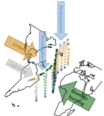
削除: Figure 16: Schematic of mechanisms that ozone and CO concentrations over the South and Tropical Atlantic for the period from 13 to 15 February 2017. →
