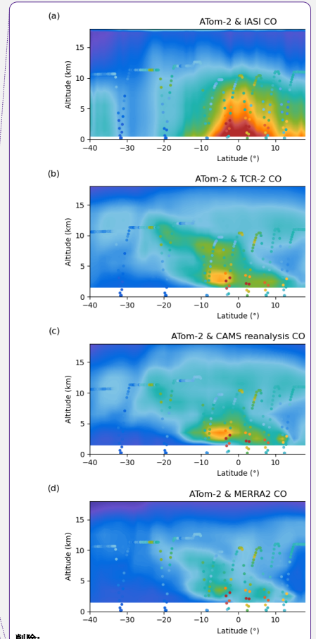
Figure 7: Vertical profiles of CO concentrations for the periods from 13 to 15 February and from 17 to 20 October 2017. Dots indicate ATom-2 and ATom-3 observations. The CO concentrations of (a) IASI, (b) TCR-2 and (c) CAMS reanalysis are averaged for the period from 13 to 15 February 2017 and from 17 to 20 October 2017, respectively, and are extracted along the ATom flight tracks.
