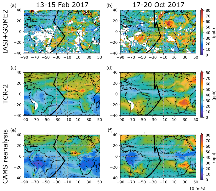
Figure 4: Distribution of mean ozone from surface to 3 km during 13–15 February and 17–20 October 2017. Black bold lines in (a–b) IASI+GOME2, (c–d) TCR-2 and (e–f) CAMS reanalysis indicate the ATom-2 and Atom-3 flight tracks. Winds at 3 km altitude from ERA5 are indicated by black arrows.
