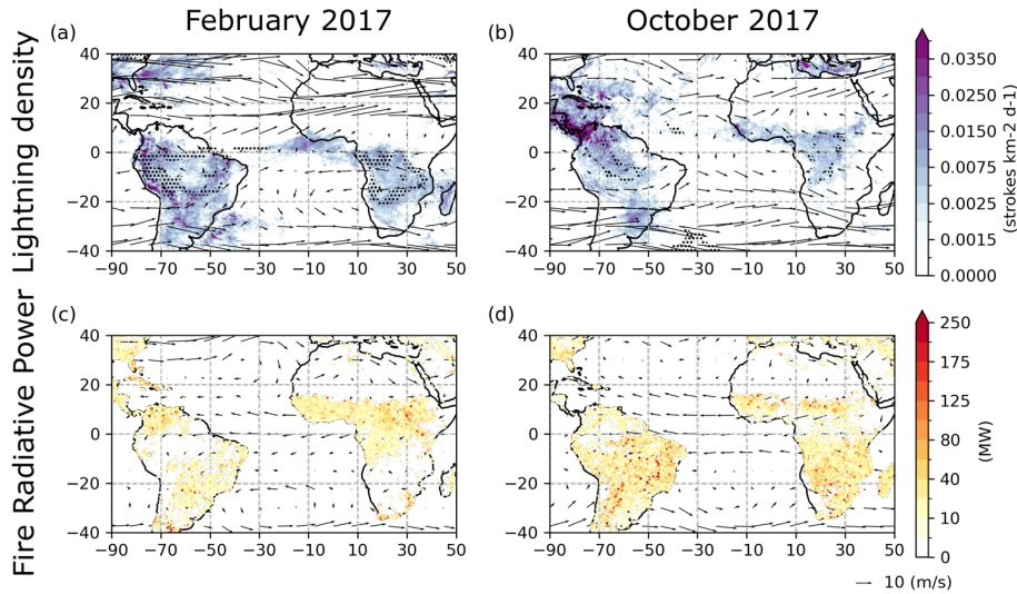
Figure 1: Monthly WGLC lightning density and fire radiative power (FRP) of presumed vegetation fire in (a and c) February, and (b and d) October, 2017. Winds at 3 and 10 km of altitude from ERA5 are indicated by black arrows in February and October, respectively. Black dots (a–b) indicate areas with OLR < 220 \text{ W m}^{-2} .
