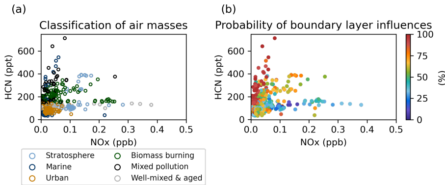
Figure 11: Scatterplots of NO x vs. HCN (biomass burning tracer) of ATom-2 observation with colours indicating (a) the air masses classification into six categories: marine (navy), stratosphere (light blue), urban (light brown), biomass burning (dark green), mixed pollution (black), well-mixed and aged air (grey), and (b) the probability of boundary layer influences.
