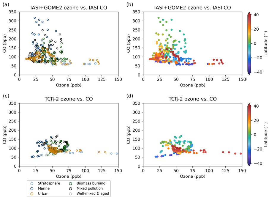
145 Figure 12. Scatterplots of CO vs. ozone for air masses sampled by ATom-2 derived from (a and b) satellite measurements of respectively IASI and IASI+GOME2 and (c and d) TCR-2. Colours indicate (a and c) the air masses classification into six categories (idem as Figs. 9a and 10a) and (b and d) the latitude location.
