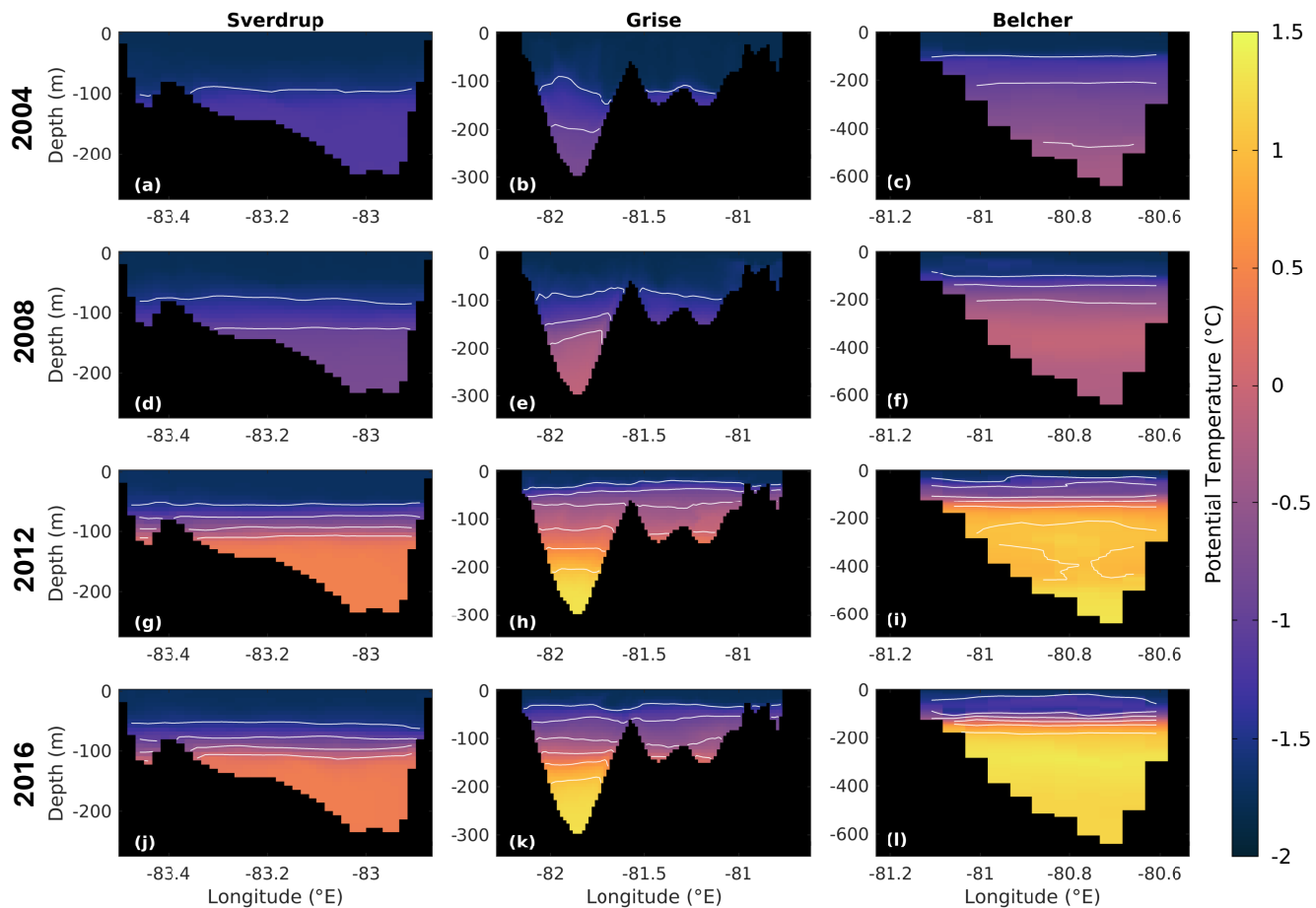
Figure A3. Vertical profiles of ocean potential temperature in April of (a-c) 2004, (d-f) 2008, (g-i) 2012, and (j-l) 2016 taken through (a/d/g/j) Sverdrup Bay, (b/e/h/k) Grise Fiord, and (c/f/i/l) the oceanic region adjacent to Belcher Glacier (white, yellow, and red lines in figure 8a). Areas of black denote land and white contours correspond to ocean temperature levels that start at -2^{\circ}\text{C} and increase in 0.5^{\circ}\text{C} increments.
