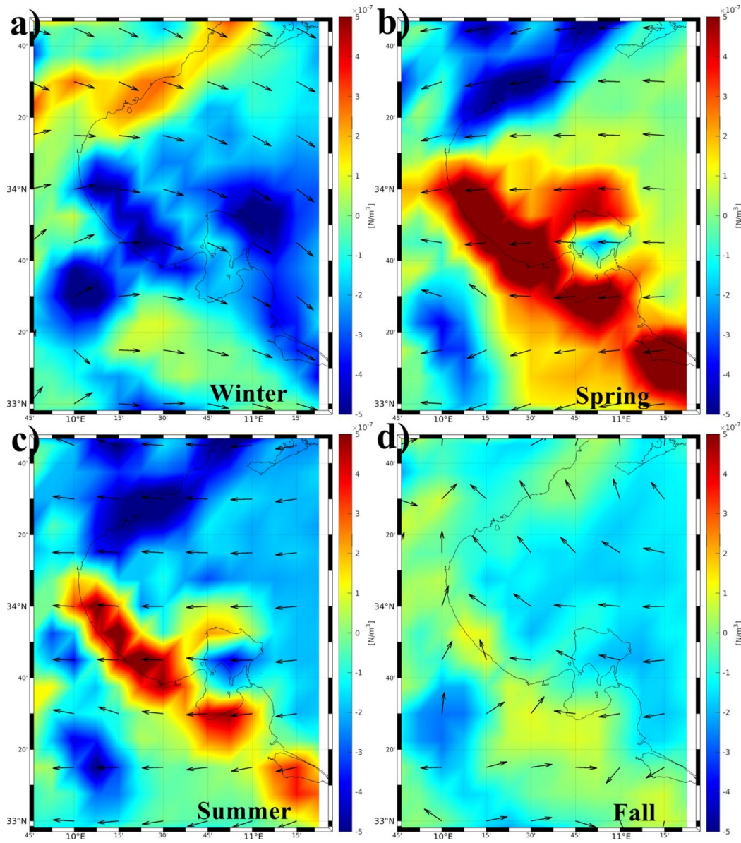
Figure 1. Seasonal variability of wind stress at 10 m above the Central Gulf of Gabes (CGG) in 2022 computed from ECMWF data (1/8°) superimposed to seasonal wind circulation, in (a) winter, (b) spring, (c) summer and (d) fall.
