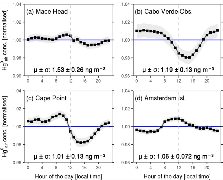
Figure 3: Normalised mean \text{Hg}^0_{\text{air}} diurnal variation at Mace Head, Cabo Verde Observatory, Cape Point and Amsterdam Island. The mean \pm the standard deviation of the hourly observations is shown for each site. The shaded area shows the mean \pm 2 times the standard error. The horizontal line represents the normalised mean value (i.e., 1 \text{ ng m}^{-3} ) and the dashed vertical line is plotted along 12:00 local time.
