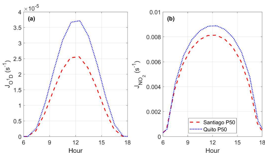
Figure 4. Comparison between the diurnal variation of frequencies of photolysis a) JO^1D and b) JNO_2 in Quito and Santiago at the 50 th percentile from model output. Time is in UTC-5.
