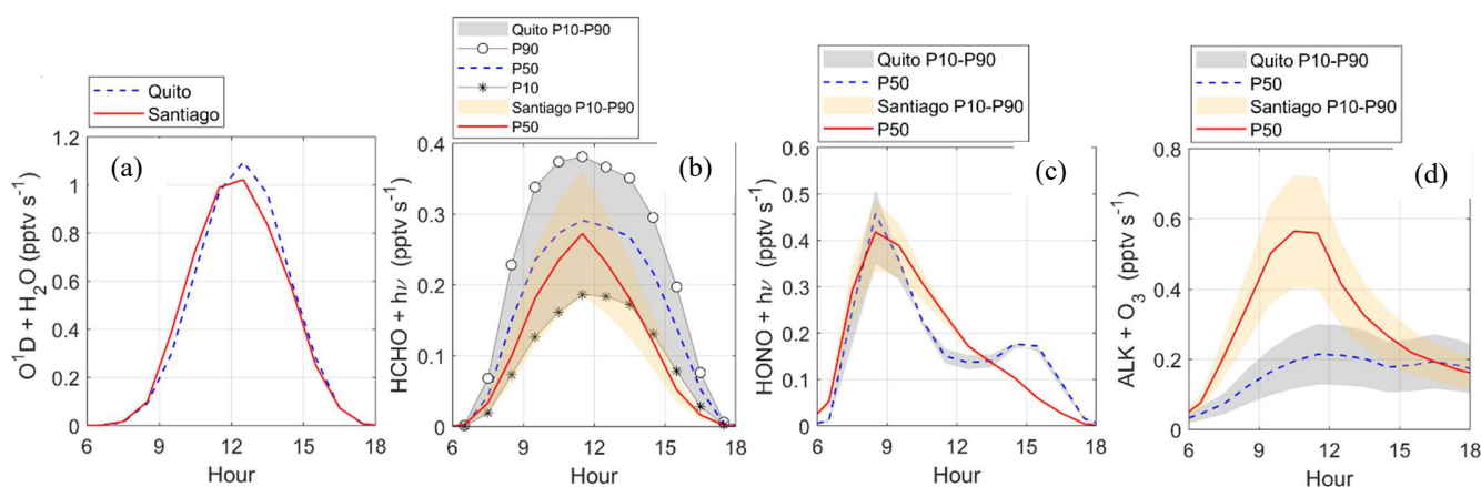
520 Figure 8. Diurnal variation of radical sources in Quito and Santiago: a) ozone photolysis followed by O^1D + H_2O , b) formaldehyde photolysis, c) HONO photolysis, and d) ozone reaction with alkenes. Shaded area indicates model output boundaries obtained with the 10 th and 90 th percentiles (P10 and P90) of the VOC Monte Carlo distribution (orange for Santiago and gray for Quito). Symbols were added to better visualize percentile boundaries when needed. The solid red line and dashed blue lines correspond to percentile 50 (P50) for Santiago and Quito, respectively. Time is in UTC-5.
