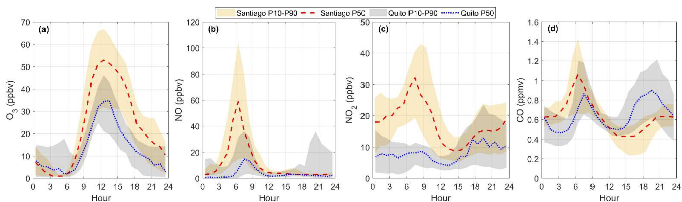
Figure 2. Diurnal variation of a) ozone, b) NO, c) NO 2 , and d) CO observed in Santiago and Quito in March 2021. The red dashed line is the diurnal variation from observations in Santiago at the 50 th percentile and the dotted blue line is the same but for Quito. The orange shadow is limited at the bottom and top by the 10 th and 90 th percentile diurnal variations from observations of every variable in Santiago. The gray shadow is the same but for Quito. Time is in UTC-5.
