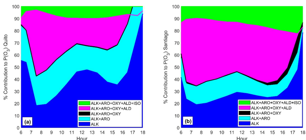
Figure 7. Percentage contribution to P(O_3) by chemical groups in a) Quito and b) Santiago obtained with model output at the 50 th percentile from VOC Monte Carlo simulations. Time is in UTC-5.
