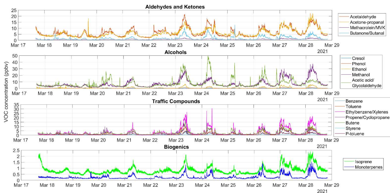
Figure B1. Time series (1-minute data) of VOC measurements taken in Santiago, Chile from 17 to 28 March.
