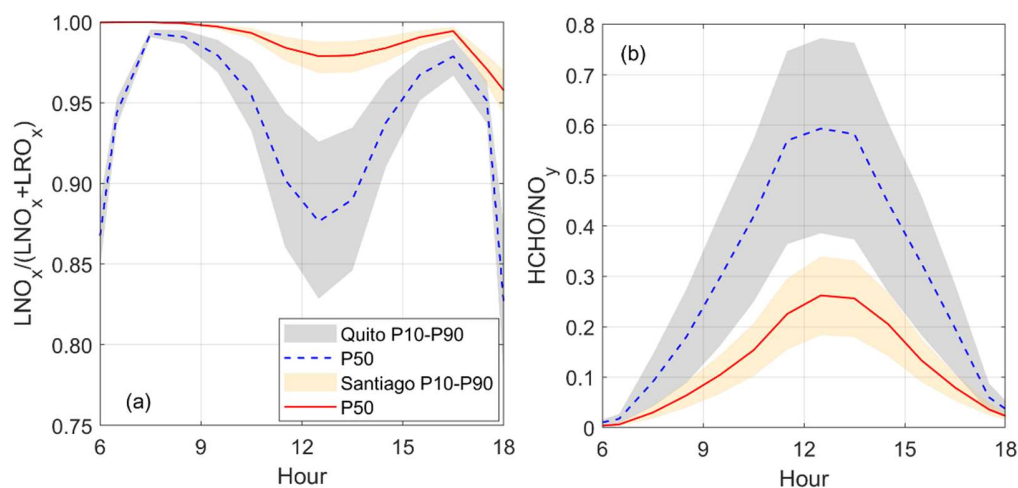
Figure 6. Indicators of the chemical regime of ozone production: a) Ratio LNO_x/(LNO_x+LRO_x) (defined by Eq. 3 and 4), b) Ratio HCHO/NO_y (formaldehyde to reactive nitrogen). Shaded area indicates model output boundaries obtained with the 10 th and 90 th percentiles (P10 and P90) of the VOC Monte Carlo distribution (orange for Santiago and gray for Quito). The solid red line and dashed blue lines correspond to model output at the 50 th percentile (P50) for Santiago and Quito, respectively. Time is in UTC-5.
