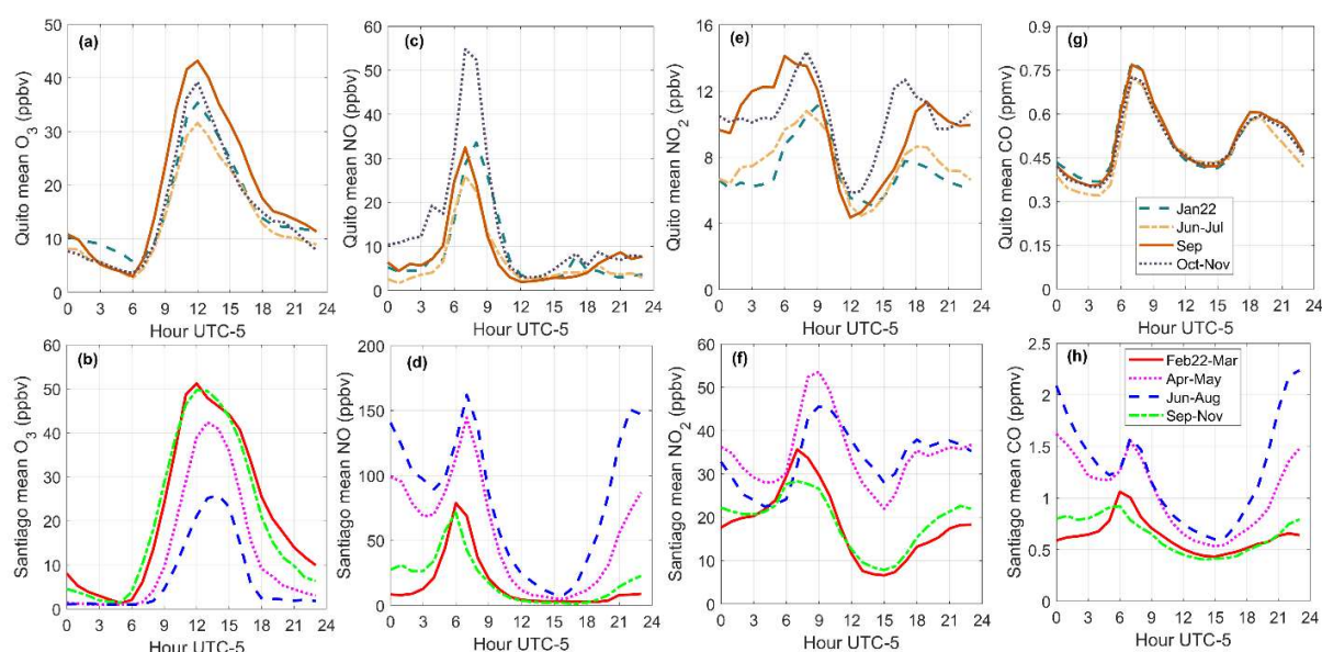
Figure 11. Mean air quality conditions observed within a year by season (Santiago) or month-grouping (Quito) presented comparatively for a) and b) ozone, c) and d) NO, e) and f) NO 2 , and g) and h) CO.
