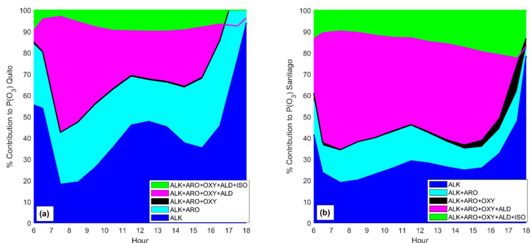
Figure 7. Percentage contribution to P(O 3 ) by chemical groups in a) Quito and b) Santiago obtained with model output at the 50 th percentile from VOC Monte Carlo simulations.
