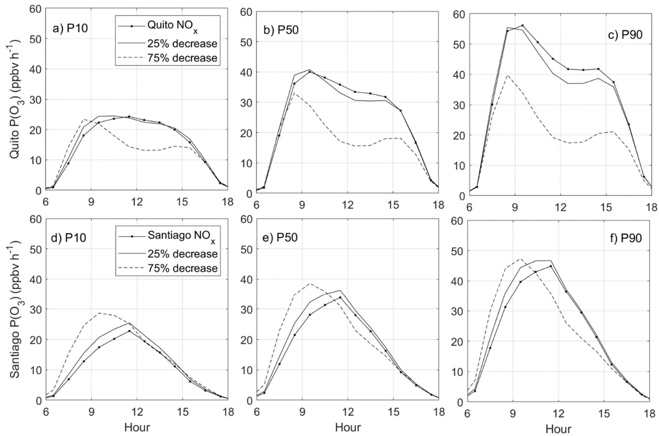
Figure 10. P(O 3 ) sensitivity to changes in NO x and VOCs in Quito (top panels) and Santiago (bottom panels) obtained with VOC levels P10, P50 and P90 from Monte Carlo simulations.
