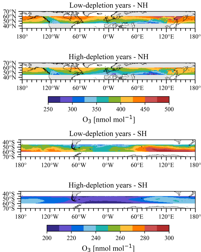
Figure 7: Ozone medians ( \text{nmol mol}^{-1} ) obtained from CAMS reanalysis filtered by RH less than 20% at a resolution of 0.75^\circ \times 0.75^\circ and between 300-200 hPa. The upper panel depicts the ozone median in UTLS of the northern hemisphere, separated into low and high depletion years (entire period), while the lower panel describes the same for the southern hemisphere. Note that the color scales are different in the NH and SH given the strong differences in ozone mixing ratios.
