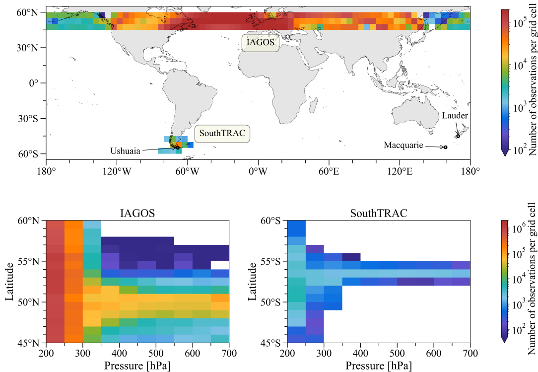
135 Figure 1: Routes position frequency obtained from aircraft GPSs. All panels show only SouthTRAC and IAGOS data within the same latitudinal band 45°-60° in the SH and NH. SouthTRAC shows data from 4 Sep to 20 Nov 2019 and IAGOS between 4 Mar and 20 May from 2002 to 2022. The upper panel shows the number of GPS observations by grid cell (5° x 5°) between 700 and 200 hPa. The lower panels show the number of GPS observations in every grid cell (1° x 50 hPa) between 700 and 200 hPa for IAGOS (left) and SouthTRAC (right). The upper panel also indicates the location of the ozonesonde sites of Ushuaia, Lauder and Macquarie Island.
