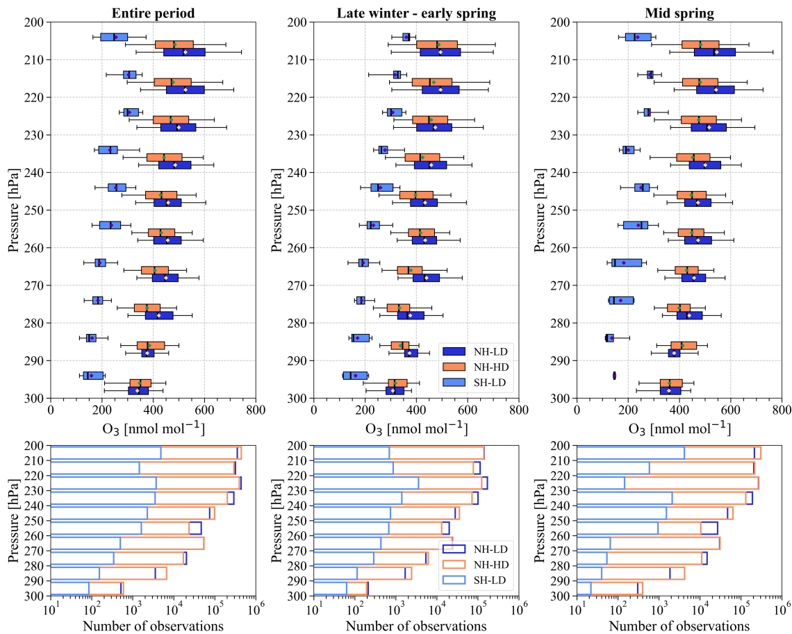
Figure C1: Ozone box plot (nmol mol -1 ) and associated observation numbers by pressure bins. The plots include ozone data with CO less than 50 nmol mol -1 . In the upper panel, the left, middle and right plots show the entire period, late winter-early spring and mid-spring for the northern and southern hemispheres and high-depleted and low-depleted years. Box plots indicate the median, the 25th and 75th percentiles. The diamonds in the upper panels indicate the mean values. The whiskers extend to the 5th and 95th percentiles. In the lower panels, the X-axis shows the observation numbers. The rest of the plot information is the same as described in the upper panel.
