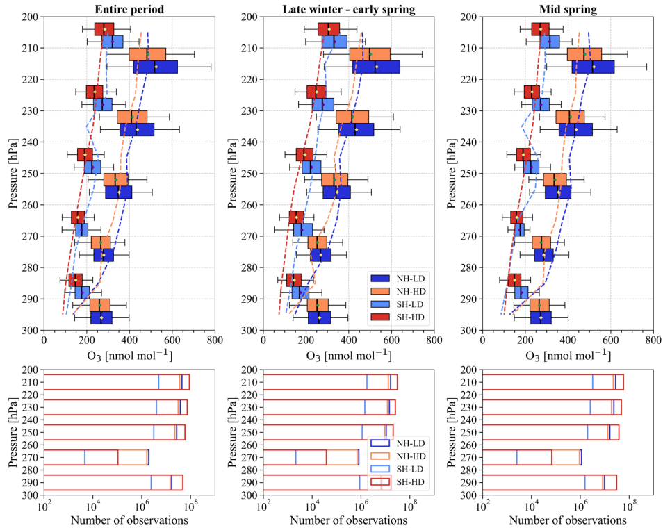
Figure 6: Ozone box plot ( \text{nmol mol}^{-1} ) and associated sample sizes by pressure bins obtained from the CAMS reanalysis. The plots include ozone data with RH less than 20%. The vertical dashed lines are the ozone medians obtained through in situ measurements previously shown in Figure 5. In the upper panel, the left, middle and right plots show the entire period, late winter-early spring and mid-spring, respectively, for the northern and southern hemispheres and high-depleted and low-depleted years. Box plots indicate the median, the 25th and 75th percentiles. The diamonds in the upper panels indicate the mean values. The whiskers extend to the 5 th and 95 th percentiles. In the lower panels, the X-axis shows the observation numbers. The rest of the plot information is the same as described in the upper panel.
