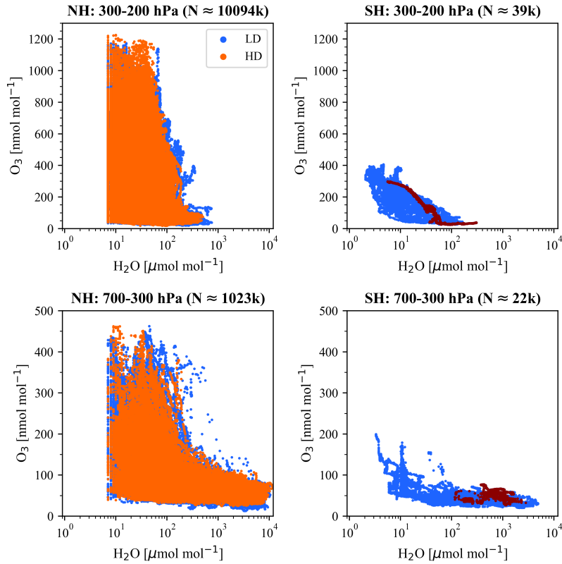
Figure 2: Scatter plots of ozone versus water vapor. The left panels show scatter plots for the period between 4 Mar and 20 May from 2002 to 2022 for the NH between 300-200 and 700-300 hPa (IAGOS data set described in Table 1). The right panels show the same for the SH between 4 Sep and 20 Nov 2019 (SouthTRAC data described in Table 1). Low and high-depletion (LD and HD) years are in blue and orange colors, respectively. Above each plot, N stands for the number of observations. In the SH, the flight conducted on 12 Nov 2019 is highlighted in dark red.
