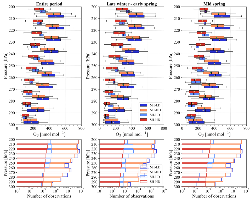
Figure 5: Ozone box plot ( \text{nmol mol}^{-1} ) and associated sample sizes by pressure bins. The plots include ozone data with RH less than 20% obtained from IAGOS, SouthTRAC and WOUDC (Table 1). In the upper panel, the left, middle and right plots show the entire period, late winter-early spring and mid-spring respectively, for the northern and southern hemispheres and high-depleted (HD) and low-depleted (LD) years. Box plots indicate the median, the 25 th and 75 th percentiles. The diamonds in the upper panels indicate the mean values. The whiskers extend to the 5 th and 95 th percentiles. In the lower panels, the X-axis shows the observation numbers. The rest of the plot information is the same as described in the upper panel. High and low-depletion years in SH included ozonesondes launched from Ushuaia, Lauder and Macquarie Island.
