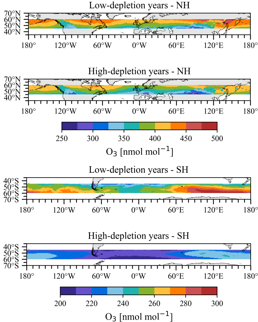
Figure 7: Ozone medians ( \text{nmol mol}^{-1} ) obtained from CAMS reanalysis filtered by RH lower less 20% at a resolution of 0.75^\circ \times 0.75^\circ and between 300-200 hPa. The upper panel depicts the ozone median in UTLS of the northern hemisphere, separated into low and high depletion years (entire period), while the lower panel describes the same for the southern hemisphere. Note that the color scales are different in the NH and SH given the strong differences in ozone mixing ratios.
