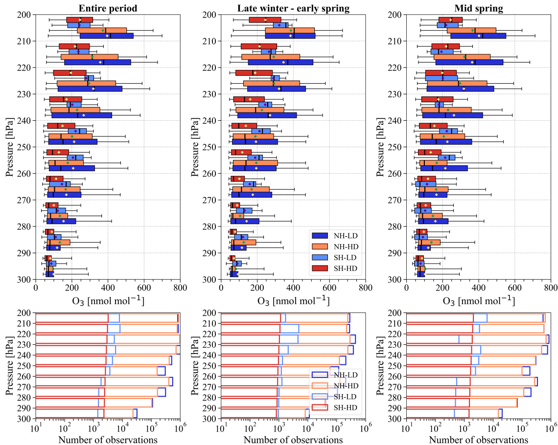
380 Figure A1: Ozone box plot (nmol mol -1 ) and associated sample sizes by pressure bins. The plots include ozone data without RH less than 20% obtained from IAGOS, SouthTRAC and WOUDC (Table 1). In the upper panel, the left, middle and right plots show the entire period, late winter-early spring and mid-spring respectively, for the northern and southern hemispheres and high-depleted (HD) and low-depleted (LD) years. Box plots indicate the median, the 25 th and 75 th percentiles. The diamonds in the upper panels indicate the mean values. The whiskers extend to the 5 th and 95 th percentiles. In the lower panels, the X-axis shows the observation numbers. The rest of the plot information is the same as described in the upper panel. High and low-depletion years in SH included ozonesondes launched from Ushuaia, Lauder and Macquarie Island. 385
