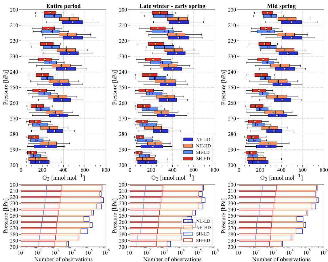
Figure B1: Ozone box plot (nmol mol -1 ) and associated sample sizes by pressure bins. The plots include ozone data with RH less than 20% obtained exclusively from IAGOS and WUDC (Table 1). In the upper panel, the left, middle and right plots show the entire period, late winter-early spring and mid-spring respectively, for the northern and southern hemispheres and high-depleted (HD) and low-depleted (LD) years. Box plots indicate the median, the 25 th and 75 th percentiles. The diamonds in the upper panels indicate the mean values. The whiskers extend to the 5 th and 95 th percentiles. In the lower panels, the X-axis shows the observation numbers. The rest of the plot information is the same as described in the upper panel. High and low-depletion years in SH included ozonesondes launched from Ushuaia, Lauder and Macquarie Island.
