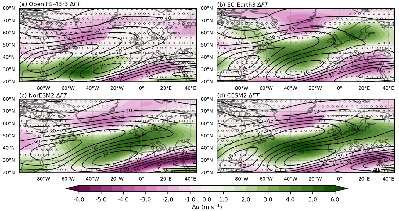
Figure 5. Future response \Delta F T in DJF mean of zonal wind speed u at 250 hPa (in colour shading), the Baseline climatology at 250 hPa (in black contours) for (a) OpenIFS-43r3, (b) EC-Earth3, (c) NorESM2, and (d) CESM2. Stippling-Shading indicates as consistent sign according to CDR testing and stippling indicates statistically insignificant changes ( p\text{-value} > 0.05 FDR corrected t-test).
