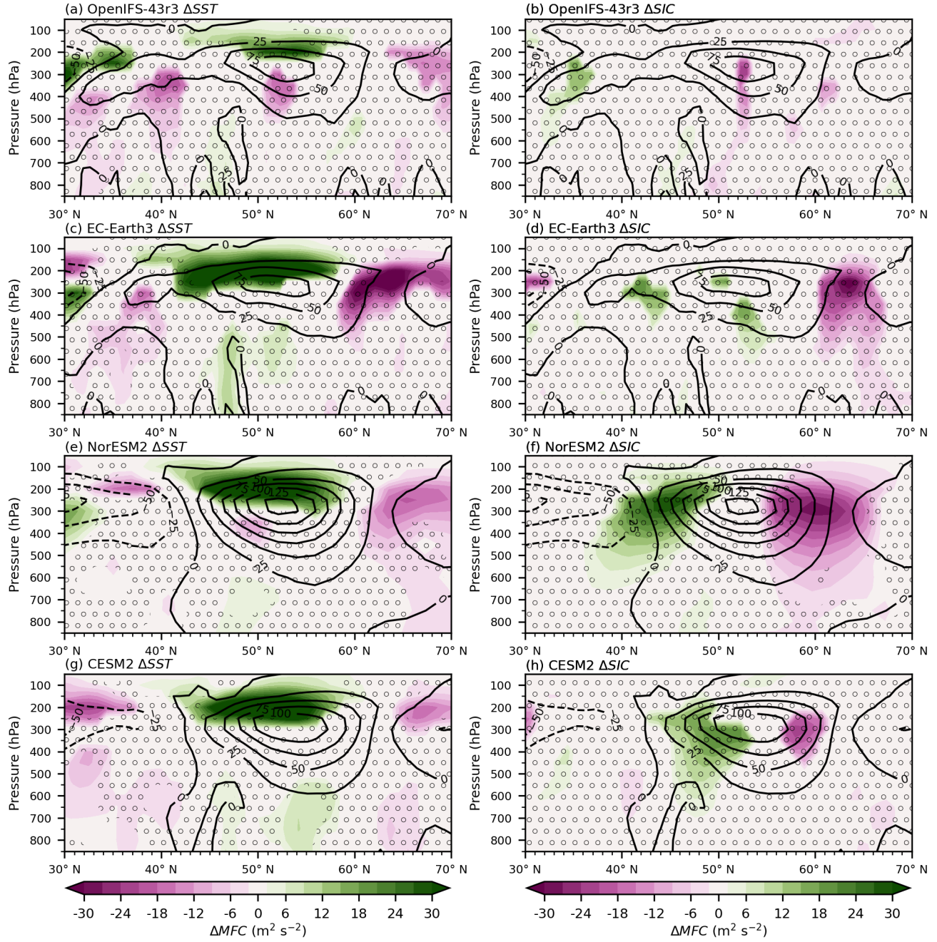
Figure 11. SST response \Delta SST (a,c,e,g) and SIC response \Delta SIC (b,d,f,h) of the zonal mean ( 15^\circ W - 35^\circ E ) of the 39-year DJF mean of momentum flux convergence MFC (in colour shading), the Baseline climatology (in black contours) for (a) & (b) OpenIFS-43r3, (c) & (d) EC-Earth3, (e) & (f) NorESM2, and (g) & (h) CESM2. Stippling-Shading indicates as consistent sign according to CDR testing and stippling indicates statistically insignificant changes ( p -value > 0.05 FDR corrected t-test).
