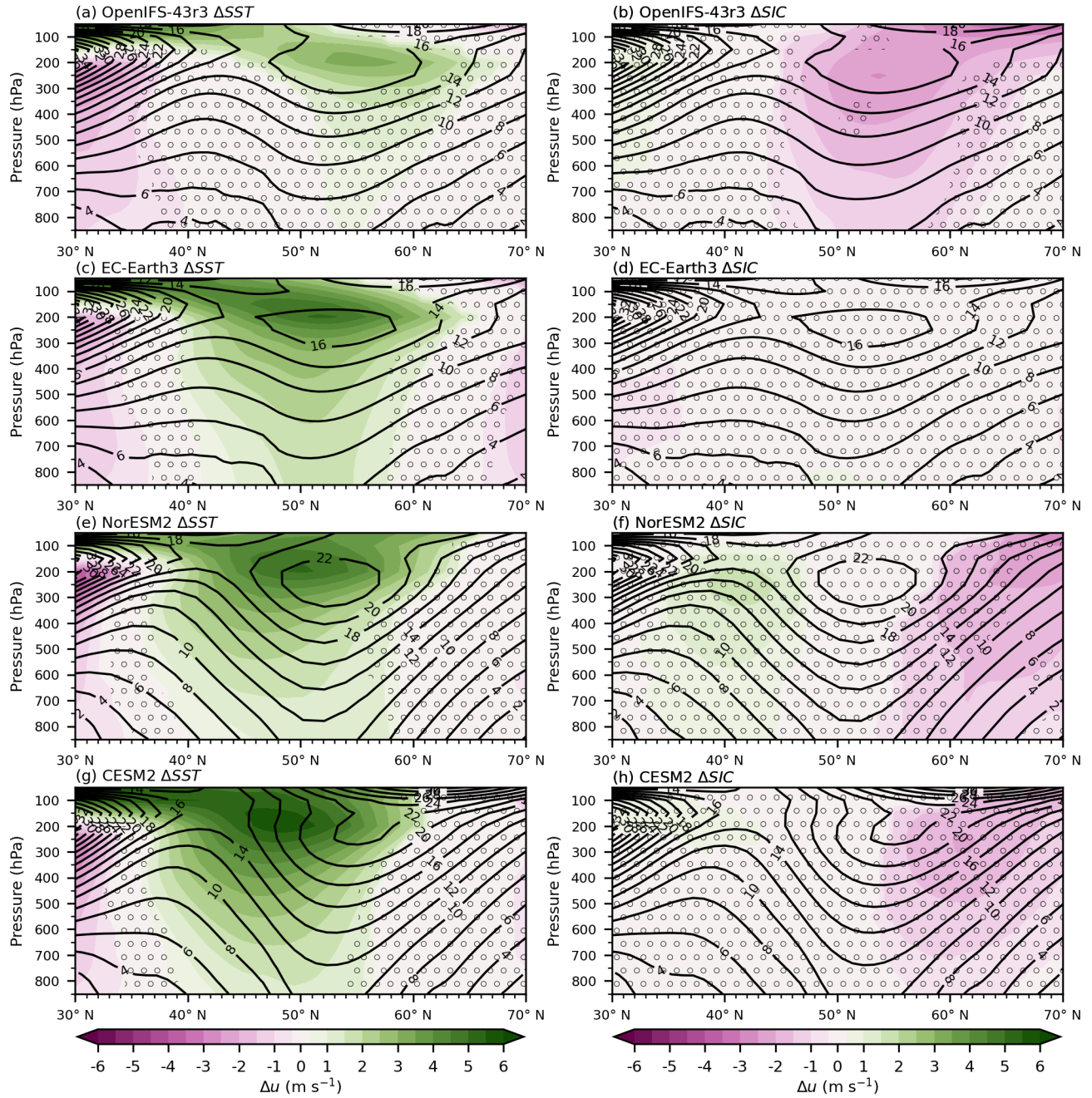
Figure 8. SST response \Delta SST (a,c,e,g) and SIC response \Delta SIC (b,d,f,h) of the zonal mean (15° W – 35° E) of the 39-year DJF mean of zonal wind speed u (in colour shading), the Baseline climatology (in black contours) for (a) & (b) OpenIFS-43r3, (c) & (d) EC-Earth3, (e) & (f) NorESM2, and (g) & (h) CESM2. Stippling Shading indicates as consistent sign according to CDR testing and stippling indicates statistically insignificant changes ( p\text{-value} > 0.05 FDR corrected t-test).
