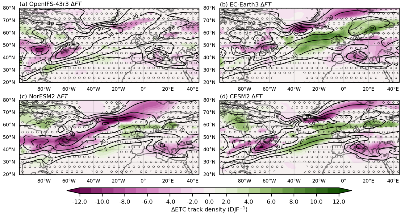
Figure 12. Future response \Delta FT of the 39-year DJF mean ETC track density (in colour shading), the Baseline climatology (in black contours) for (a) OpenIFS-43r3, (b) EC-Earth3, (c) NorEMS2, and (d) CESM2. The unit is number of ETCs per 5^\circ spherical cap per winter season (DJF). Stippling-Shading indicates as consistent sign according to CDR testing and stippling indicates statistically insignificant changes ( p\text{-value} > 0.05 FDR corrected t-test).
