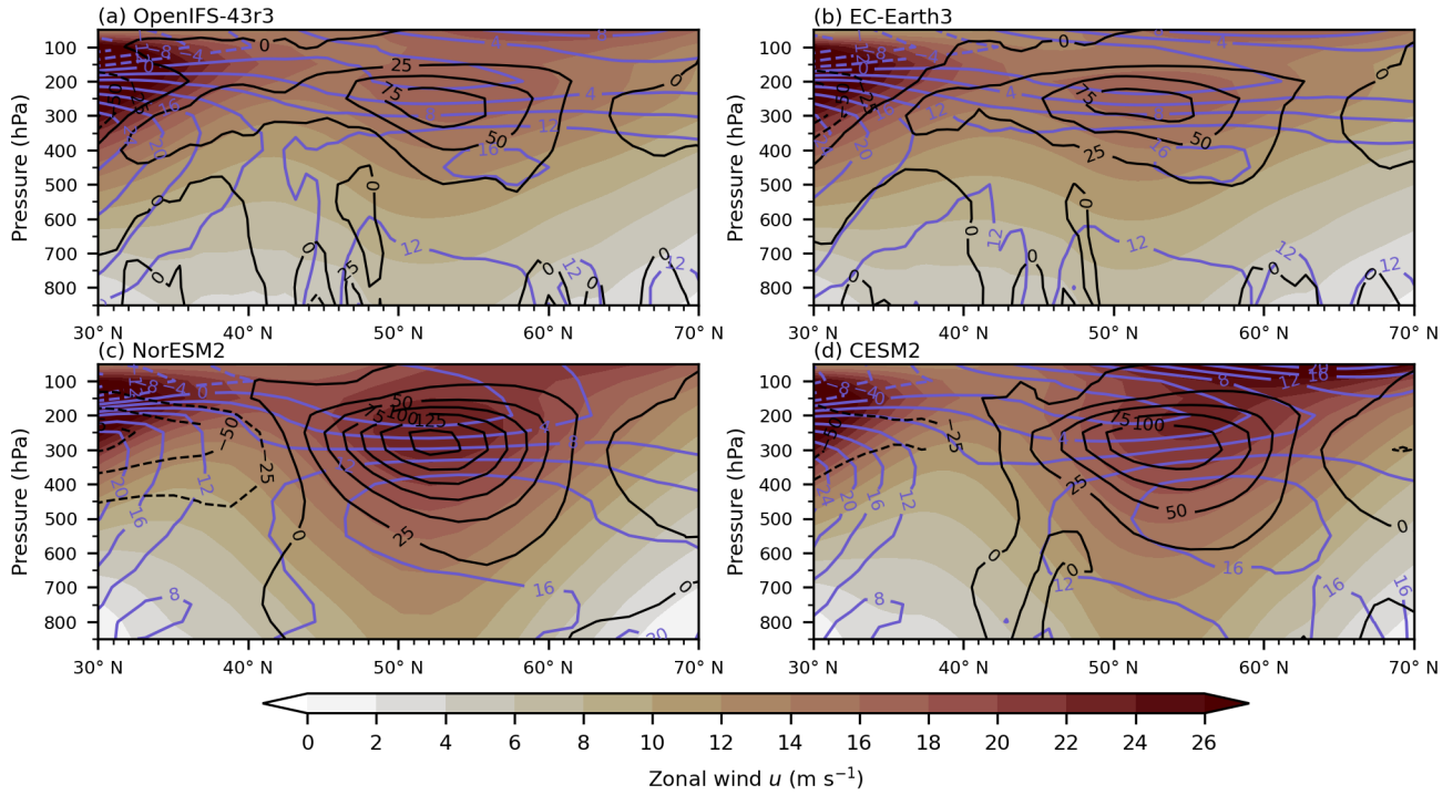
Figure 3. Zonal mean ( 15^{\circ} W – 35^{\circ} E) of the 39-year DJF mean of zonal wind speed u (in colour shading, \text{m s}^{-1} ), eddy momentum flux convergence MFC (in black contours, \text{m}^2 \text{s}^{-2} ), and baroclinicity B_y (in blue contours, 10^{-4} \text{s}^{-1} ) for (a) OpenIFS-43r3, (b) EC-Earth3, (c) NorESM2, and (d) CESM2.
