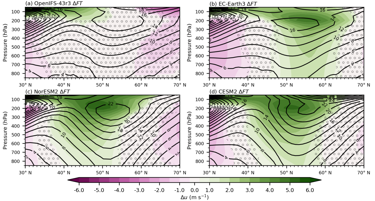
Figure 6. Future response \Delta F T of zonal mean ( 15^{\circ} \text{ W} - 35^{\circ} \text{ E} ) of the 39-year DJF mean of zonal wind speed u (in colour shading), the Baseline climatology (in black contours) for (a) OpenIFS-43r3, (b) EC-Earth3, (c) NorESM2, and (d) CESM2. Stippling-Shading indicates as consistent sign according to CDR testing and stippling indicates statistically insignificant changes ( p\text{-value} > 0.05 FDR corrected t-test).
