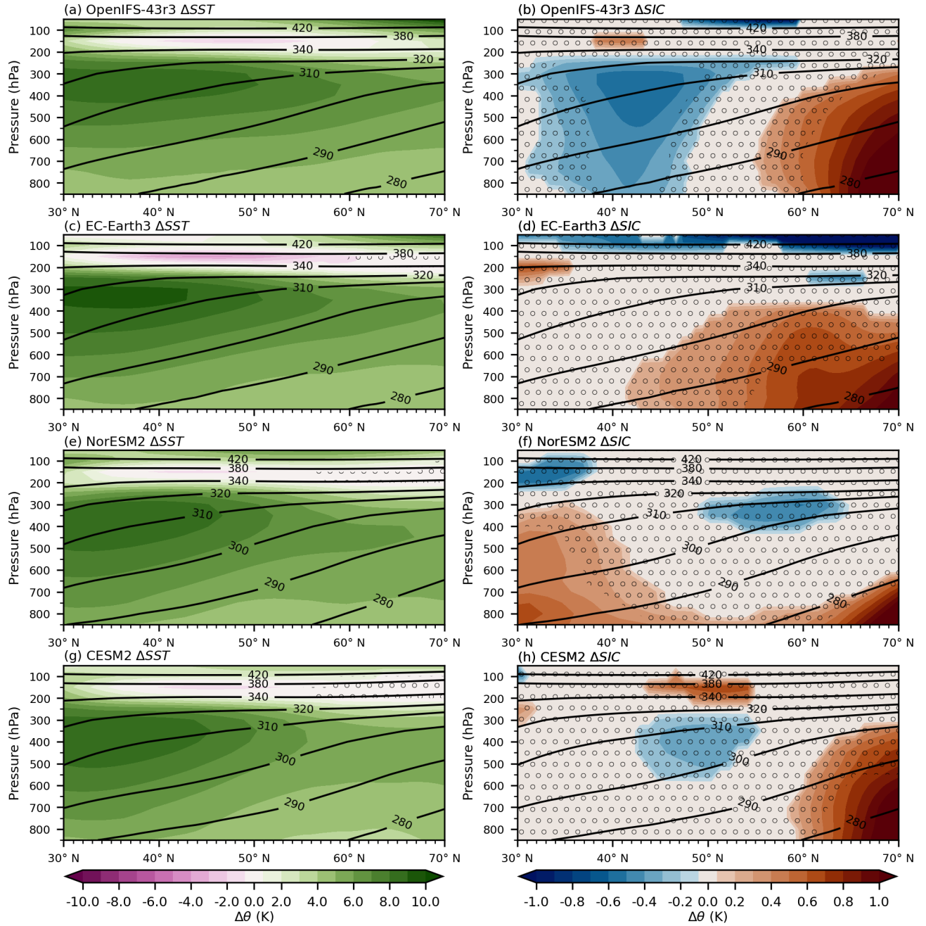
Figure 10. SST response \Delta SST (a,c,e,g) and SIC response \Delta SIC (b,d,f,h) of the zonal mean (15° W – 35° E) of the 39-year DJF mean of potential temperature \theta (in colour shading), the Baseline climatology (in black contours) for (a) & (b) OpenIFS-43r3, (c) & (d) EC-Earth3, (e) & (f) NorESM2, and (g) & (h) CESM2. Stippling Shading indicates as consistent sign according to CDR testing and stippling indicates statistically insignificant changes ( p\text{-value} > 0.05 FDR corrected t-test). Note that different colour scales are used because the absolute values of \Delta SST are larger than those of \Delta SIC .
