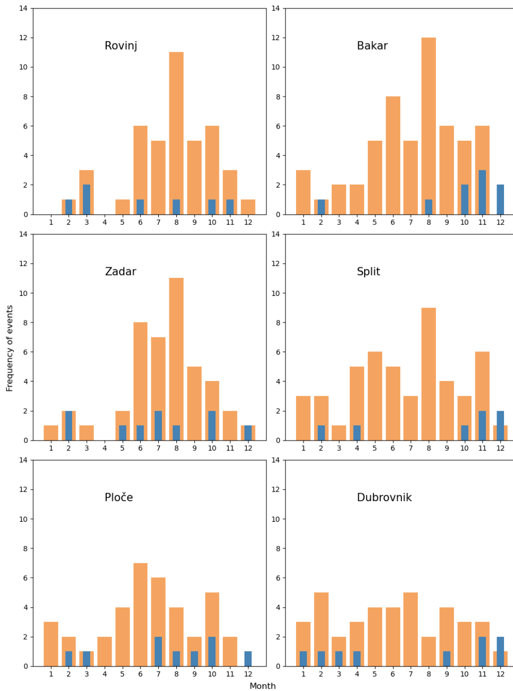
265 Figure 5: Monthly distribution of the HF (orange bars) and Compound (blue bars) extremes at six tide gauge stations, estimated for the entire period of measurements (2003 to 2021).
