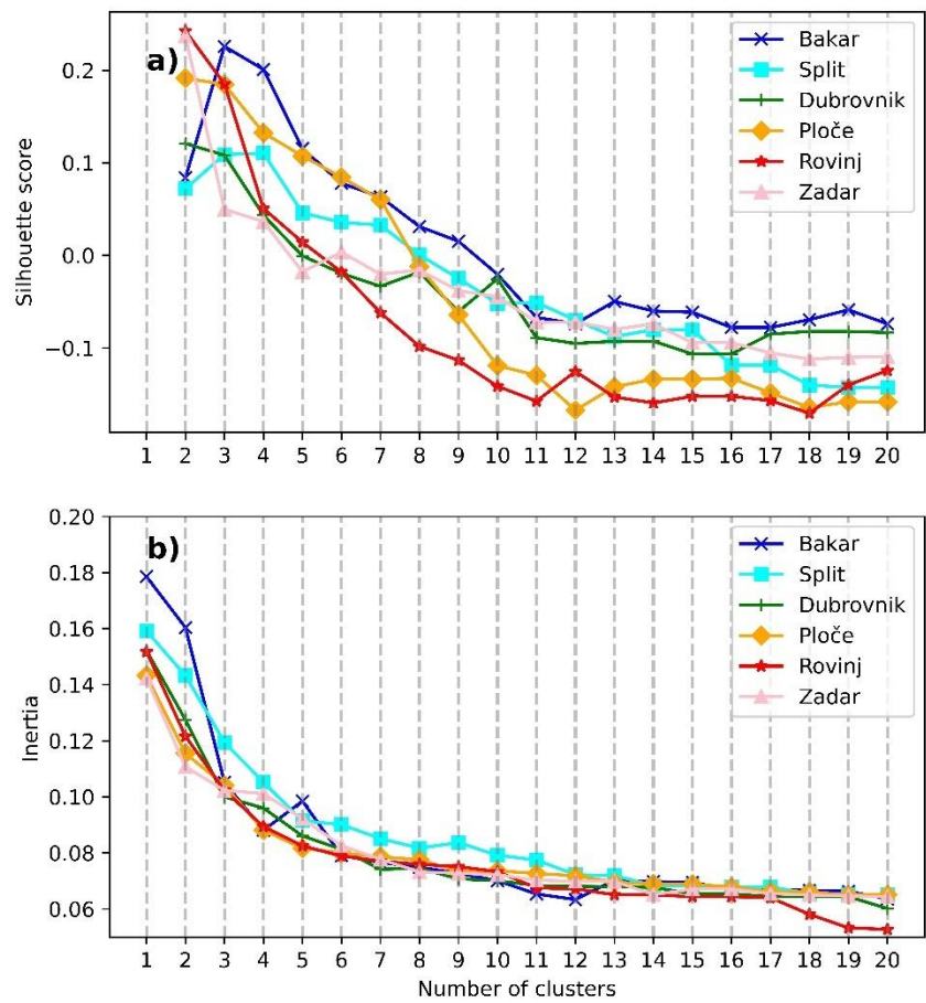
Figure 3: a) Silhouette and b) Elbow methods for determining the optimal number of clusters. Each colour in the plots represent a different tide gauge station as shown in the legend.
