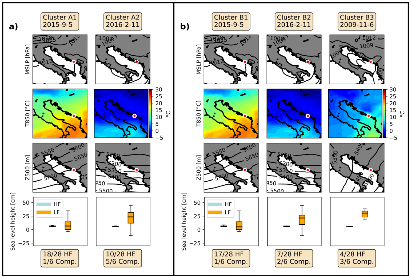
375 Figure 8: Medoids for the choice of a) two and b) three clusters for Dubrovnik. The first three rows are: MSLP, temperature at 850 hPa (T850), and geopotential height at 500 hPa (Z500). Forth row are the box-plots of HF (blue box) and LF (orange box) heights during HF extremes assigned to each medoid. The dates of medoids are given at the top of each column and the location of Dubrovnik tide gauge is marked with a circle. Additionally, at the bottom of each column the numbers of HF and Compound extremes labelled in each cluster are given.
