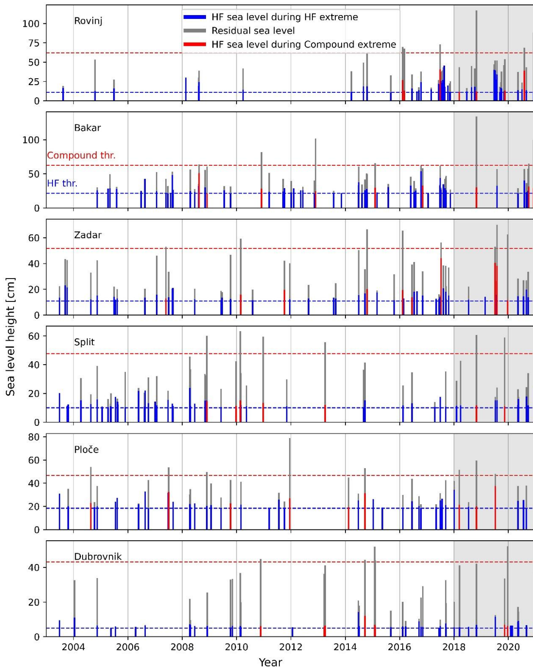
Figure 4: Temporal distribution of high-frequency sea level extremes at six tide gauge stations. Blue bars denote HF sea level during HF extremes, red bars denote HF sea level during Compound extremes, and grey bars denote residual sea levels for both types of extremes. The grey shaded area (2018 to 2021) marks the testing period, while the white area marks the training period (2003 to 2018). Red dashed line marks the threshold of the residual sea level height for the definition of a Compound extreme, while the blue dashed line marks the threshold of the HF sea level height for the definition of HF extremes.
