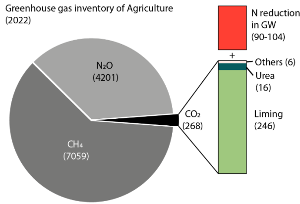
Figure 4. National inventory of greenhouse gas emissions from Danish agriculture. The numbers represent GHG emissions in kt of CO 2 equivalent yr -1 . The red box labeled “N reduction in GW” shows the potential CO 2 emissions from denitrification in groundwater estimated in this study.
