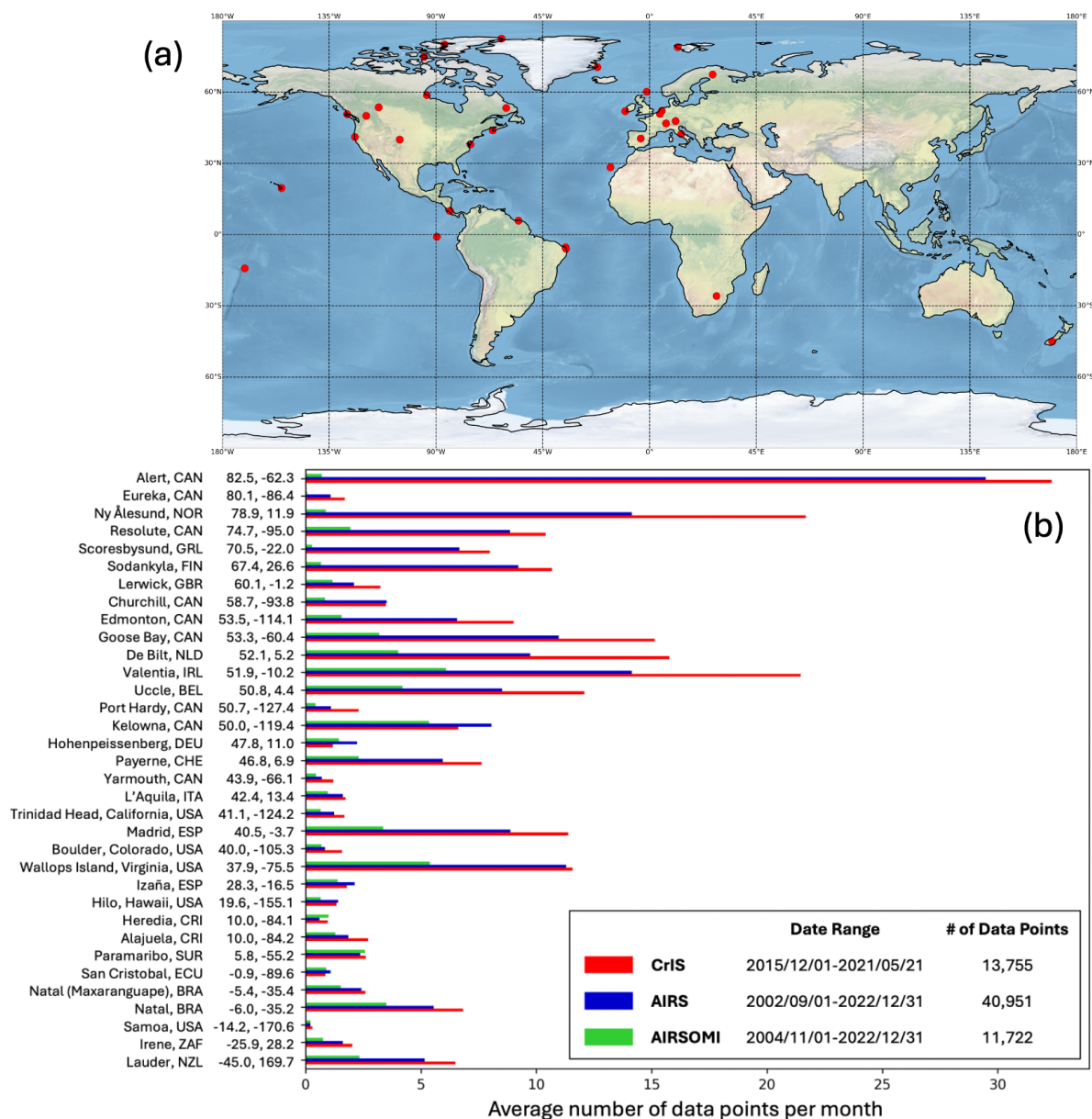
Figure 2. (a) Ozone sonde launch sites providing harmonized data in this study. (b) Monthly average number of matched satellite-sonde data points at each sonde launch site for each satellite product. Sites are ordered by decreasing latitude. The figure legend provides the date range of each satellite product and the total number of matched satellite-sonde data points over the date range at all sites.
